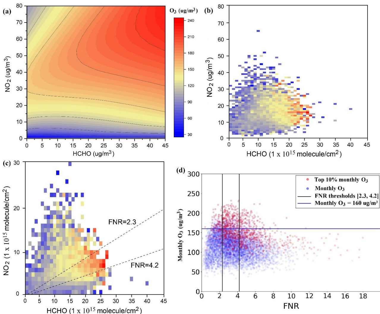
685 Figure 1: (a) The simulated O 3 isopleths versus NO 2 and HCHO using the CLASS model. (b) The 360 cities' monthly mean in-situ O 3 concentrations versus in-situ NO 2 concentrations and HCHO columns from OMI observations in the summer during 2016-2019. Note: daily ground-based O 3 and NO 2 observations are calculated from hourly observations at OMI overpass time (averaged at 13:00 LT and 14:00 LT). The O 3 numeric value of the grid cells is average of all points falling in each bin. (c) same as (b), but with NO 2 columns from OMI observations. (d) The top 10% monthly O 3 values and corresponding FNRs of each city. FNR thresholds 690 are defined as the \pm 30\% range from the median of monthly O 3 exceeding 160 \mu\text{g}/\text{m}^3 in the top 10% dataset.
