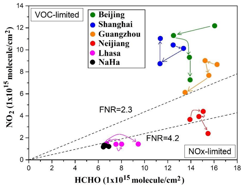
Figure 3: The change of \text{O}_3 formation sensitivity of six cities (Beijing, Shanghai, Guangzhou, Neijiang, Lhasa and NaHa) in summer from 2016 to 2019. The arrows represent time step from 2016 to 2019.
