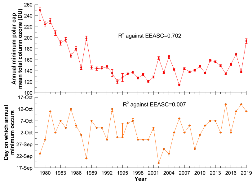
Figure 8. Annual minima in the daily polar cap mean TCO time series and the dates on which those minima occurred. Error bars show the \pm 1\sigma uncertainties which are often asymmetrical.
