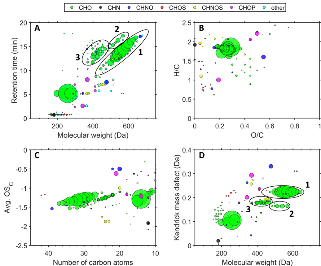
Figure 3. Molecular fingerprints (Retention time vs. MW [A], Van-Krevelen-diagram [B], Kroll-diagram [C], Kendrick mass defect vs. MW [D]) of six averaged airport-related ultrafine particle samples in the size range of 0.032-0.056 \mu\text{m} .
