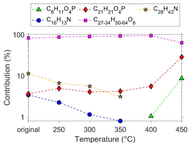
390 Figure 6. Development of the different constituents of the Eastman Turbo Oil 2380 during the temperature experiment. The contribution (%) is defined as the ratio of the area of one single compound relative to the total area of all jet oil constituents.
