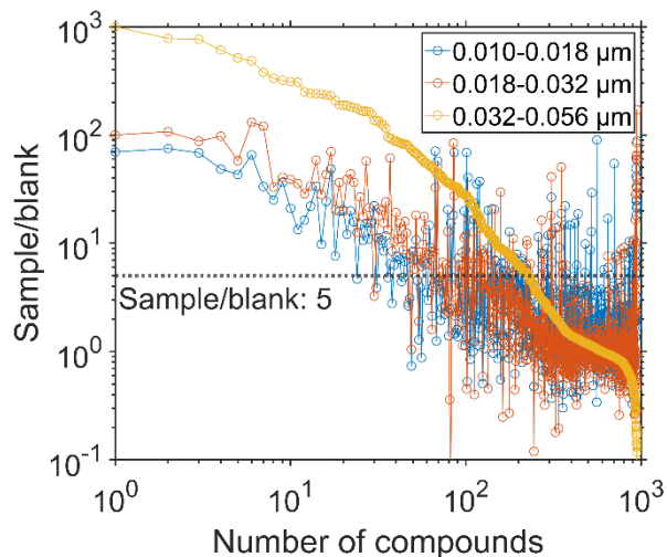
Figure 2. The sample-to-blank ratios of the detected compounds, averaged over all samples belonging to a certain size fraction (0.010-0.018 \mu\text{m} ; 0.018-0.032 \mu\text{m} ; 0.032-0.056 \mu\text{m} ). Detection of the compounds was accomplished in positive ionisation mode. The sample-to-blank ratio of 5 was specified for data filtering and is displayed as a dashed horizontal line.
