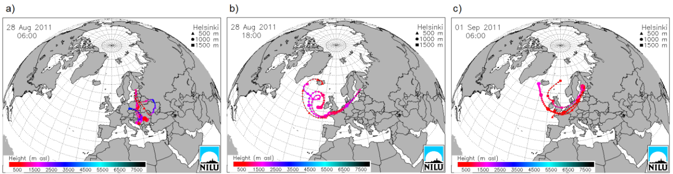
Figure 5. Selected airmass trajectories 28.8. at 6 am (a) and at 6 pm (b), and 1.9. at 6 am (c) during our campaign of 2011. The times are given in UTC, whereas our data sets are given in EET (UTC+2).
