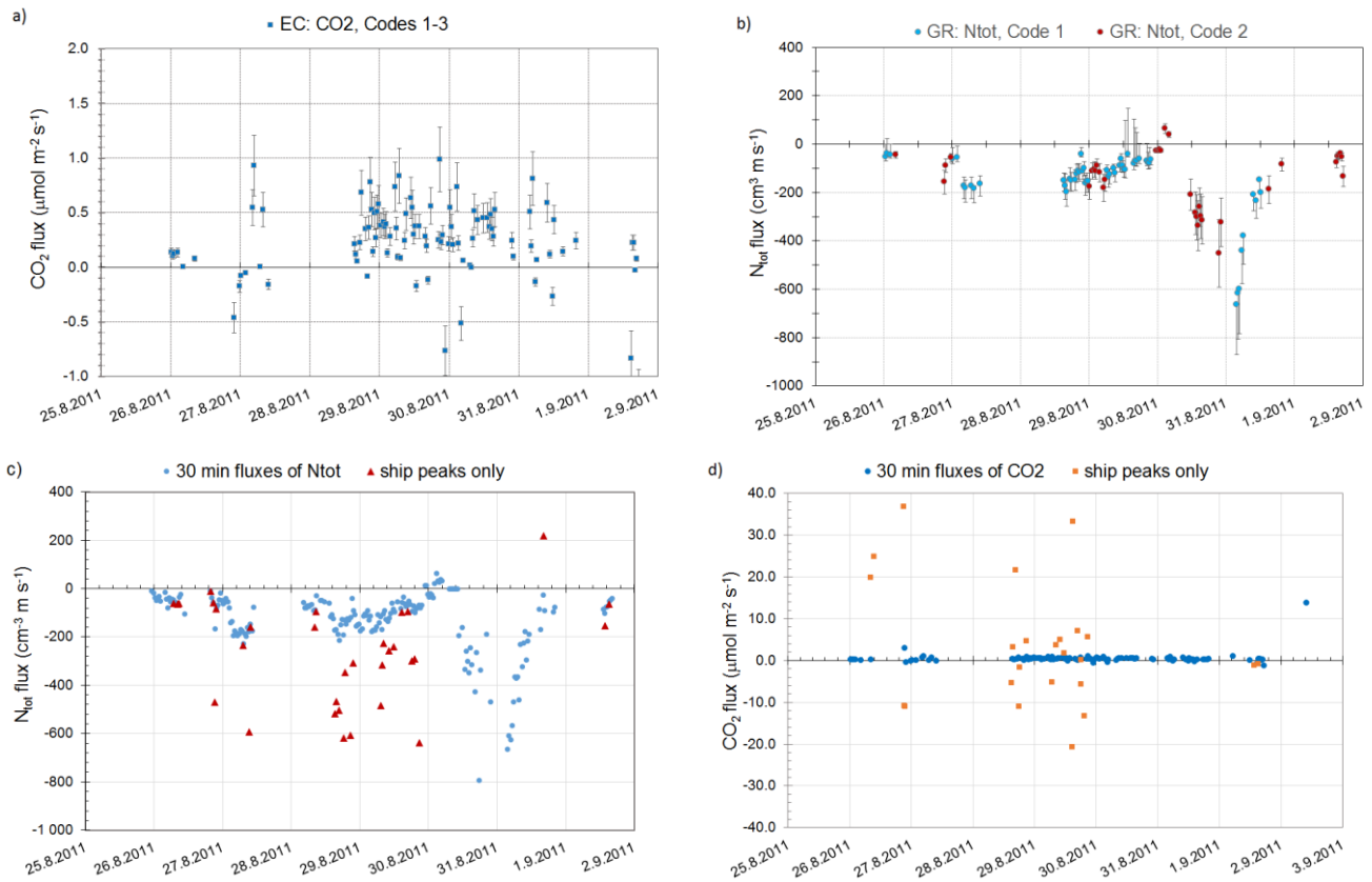
790 Figure 11. Time series of 30 min fluxes for CO 2 (μmol m -2 s -1 ) by the EC methods (a) in all wave conditions (codes 1 to 3), and N tot (cm -3 m s -1 ) by the GR method (b) with no swell (codes 1-2), along with the uncertainties. The data in (a) and (b) include only events in the wind sector between 150° and 270° and with the stationary criteria based on the momentum flux for N tot and the CO 2 flux for CO 2 . c) Time series of the 30 min fluxes of N tot by the GR method in the wind direction of 150-270 °. Additionally, the fluxes of ship peaks are shown separately. d) The same as c) but for CO 2 fluxes.
