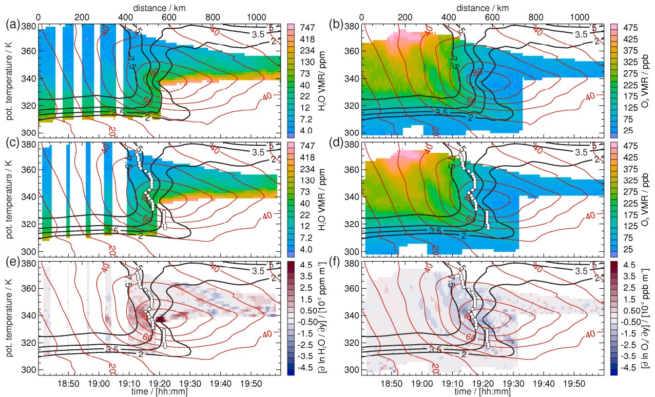
430 Figure 9: Regridded DIAL observations of (a) H_2O and (b) O_3 (as shown in Fig. 3) using potential temperature as vertical coordinate (same profile locations and for potential temperature bins of 2 K). (c, d) as (a, b) but using a moving average filter along isentropic levels (using 7 observations for H_2O and O_3 and 13 model values for PV and wind speed). (e, f) show isentropic gradients of the natural logarithm of VMR H_2O and VMR O_3 based on the isentropically smoothed data. All panels are superimposed by PV contours (2, 3.5, 5 and 7 PVU, thick black contours) and wind speed (in m s^{-1} for > 30 m s^{-1} ). White dots in c–f mark the PV-gradient-tropopause based on maximum gradients of isentropic PV and winds following Kunz et al. (2011a) (for details see text).
