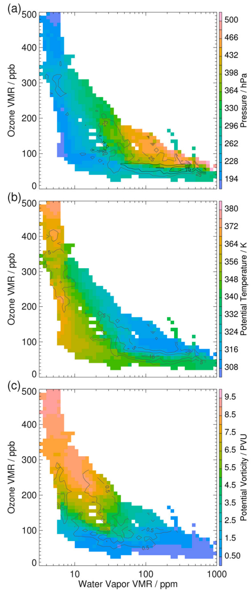
340 Figure 5: T-T correlation as in Fig. 4b but for mean (in colours) and standard deviation (grey contours) of (a) pressure (in hPa), (b) potential temperature (in K) and (c) potential vorticity (in PVU).
