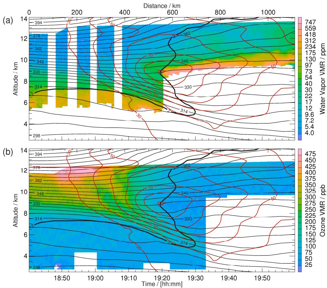
255 Figure 3: DIAL observations (in colours) of (a) H 2 O volume mixing ratio (VMR, in ppm = 10 -6 = μmol mol -1 ) and (b) O 3 VMR (in ppb = 10 -9 = nmol mol -1 ) on 1 October 2017 (see Fig. 1 for the flight track). (a) and (b) are superimposed by horizontal wind speed (red contours, in m/s for wind speeds > 30 m s -1 ), potential temperature (black contours, in K) and dynamical tropopause (2 PVU, thick black contour) interpolated from one-hourly ECMWF ERA-5 reanalyses.
