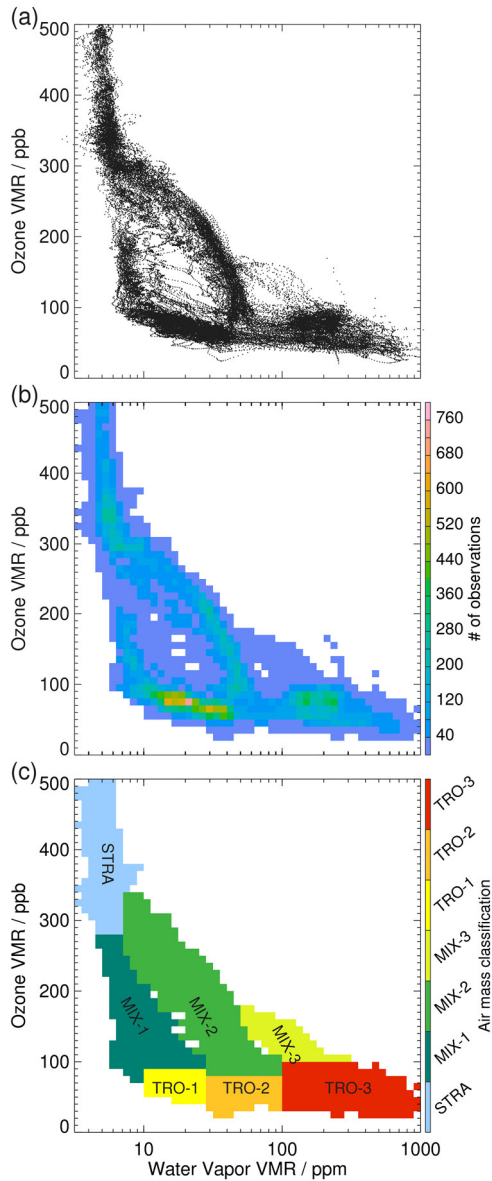
335 Figure 4: Tracer-tracer (T-T) correlations of O_3 and H_2O for the collocated DIAL data on 1 October 2017. (a) All collocated observations. (b) Number of data points and (c) air mass classification for bins in T-T space (bin sizes of 10 ppb for VMR O_3 and 0.05 of \log_{10} (VMR H_2O /ppm)).
