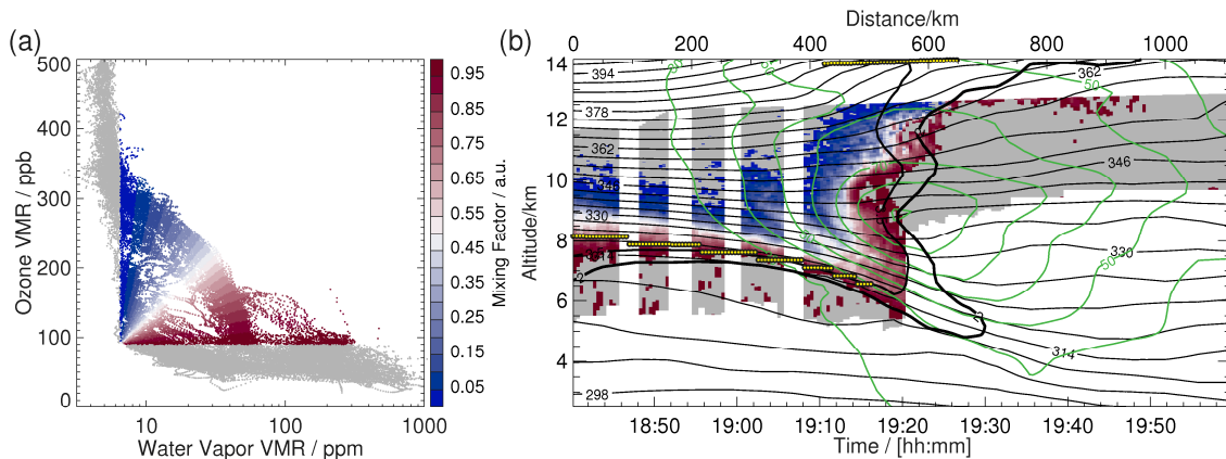
Figure 7: Mixing factor diagnostic for all collocated measurements in (a) T-T space using lower limits for H 2 O VMR of 6.5 ppm and for O 3 VMR of 90 ppb for selecting mixed air masses (for details see text) and (b) projected back to geometrical space with superimposed model information as in Fig. 6.
