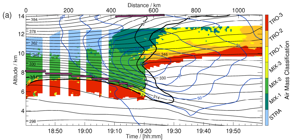
355 Figure 6: (a) Collocated observations coloured by the air mass classification in Fig. 4c. Superimposed model information as in Fig. 3 with an additional PV contour for 3.5 PVU. Pink circles mark the thermal tropopause according to the temperature lapse rate criterion (WMO, 1957)
