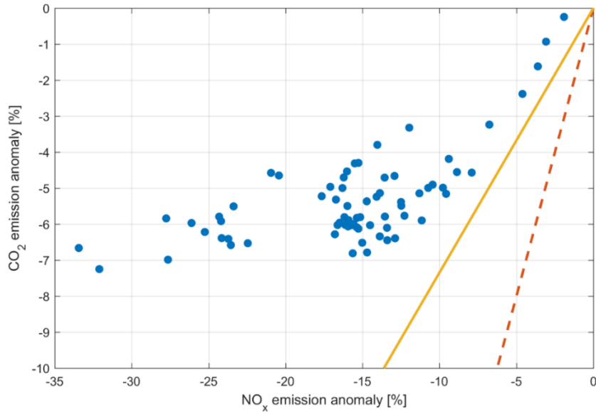
716 717 Fig. 5. Daily change of CO 2 and NO x fluxes during the lockdown period. Flux observations are 718 depicted by the blue dots. Emission model projections are represented by the solid orange 719 line (Austrian emission inventory) and the dashed red line (Quéré et al., 2020). 720
