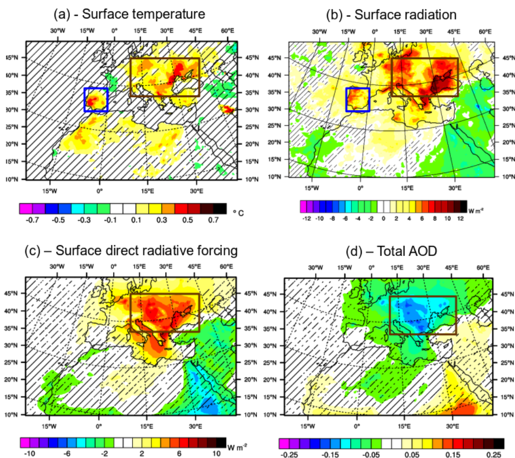
Figure 13. Mean differences, for the months of June, July and August, between SSP585 and SSP585cst simulations over the period 2021-2050 for the surface temperature ( ^{\circ}\text{C} , a), the surface radiation ( \text{W m}^{-2} , b), the surface direct radiative forcing ( \text{W m}^{-2} , c) and the total AOD (d). The brown frame represents Central Europe and the blue frame locates the Iberian Peninsula. The hatched areas are statically non significant with a threshold of 10%.
