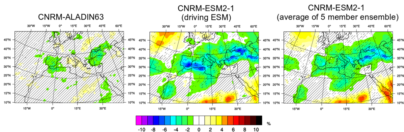
Figure A2. Mean difference, for the months of June, July and August, between SSP585 and SSP585cst simulations over the period 2021-2050 for the cloud cover (%) with the CNRM-ALADIN63 model and its driving ESM. The hatched areas are statically non significant with a threshold of 10%.
