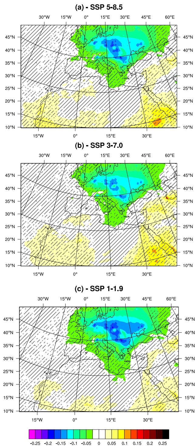
Figure 4. Total AOD evolution between the past period (1971-2000) and the future period (2021-2050) following SSP 5-8.5 (a), SSP 3-7.0 (b) and SSP 1-1.9 (c). The hatched areas are statically non significant with a threshold of 10%.
