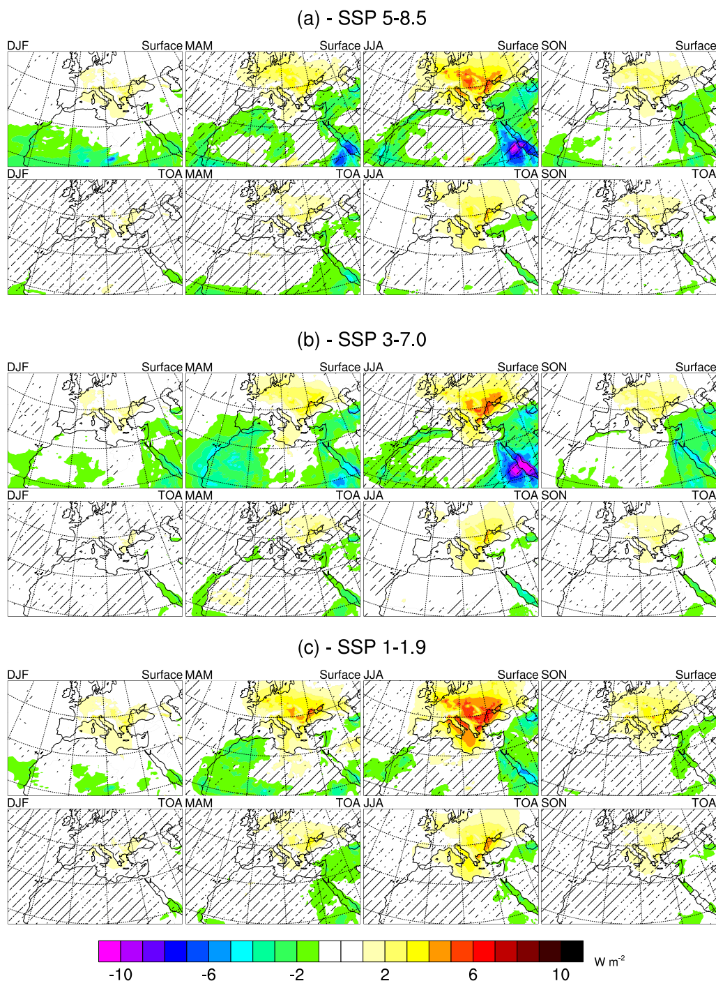
Figure 9. Mean aerosols SW DRF evolution ( W m^{-2} ) at the surface and at the TOA between the historical period (1971-2000) and the future period (2021-2050) according to SSPs 5-8.5 (a), 3-7.0 (b) and 1-1.9 (c). The hatched areas are statically non significant with a threshold of 10%.
