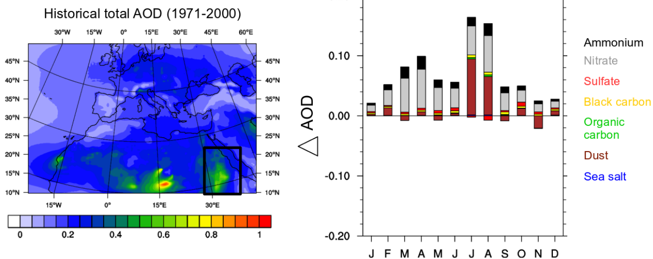
Figure 6. Historical total AOD and its evolution between the past period (1971-2000) and the future period (2021-2050) according to the SSP 5-8.5 over the East African region which is framed in black. The hatched areas are statically non significant with a threshold of 10%.
