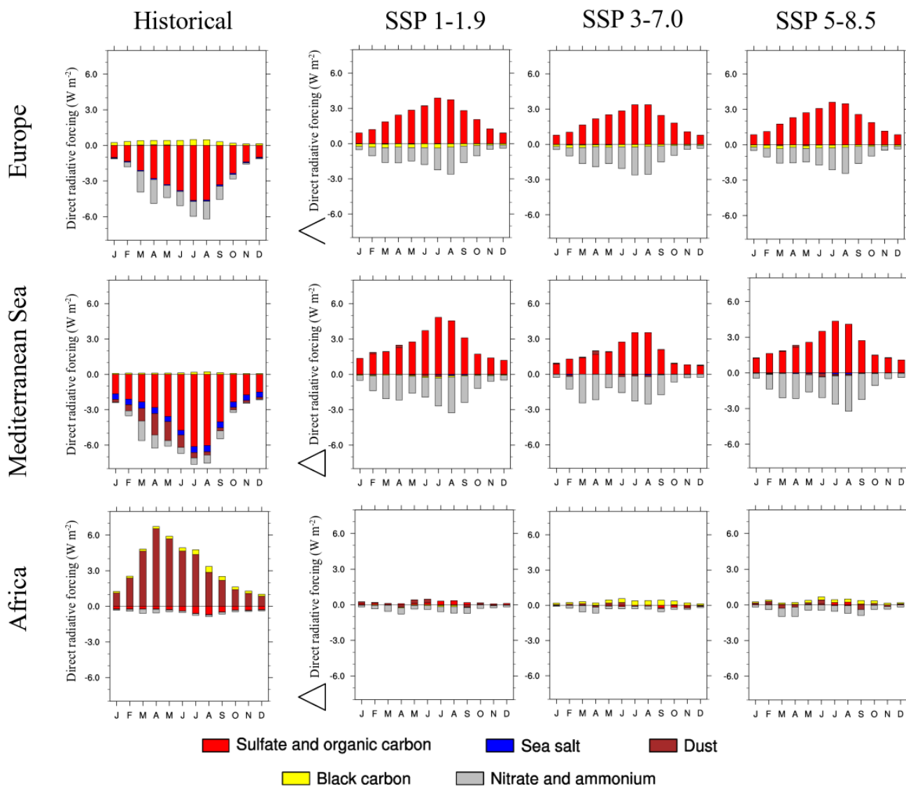
Figure A1. SW DRF evolution ( W m^{-2} ), at the TOA, of sulfate and organic carbon (in red), sea salt (in blue), dust (in brown), black carbon (in yellow) and nitrate and ammonium (in grey) between the historical period (1971-2000) and the future period (2021-2050) according to SSPs 1-1.9, 3-7.0 and 5-8.5.
