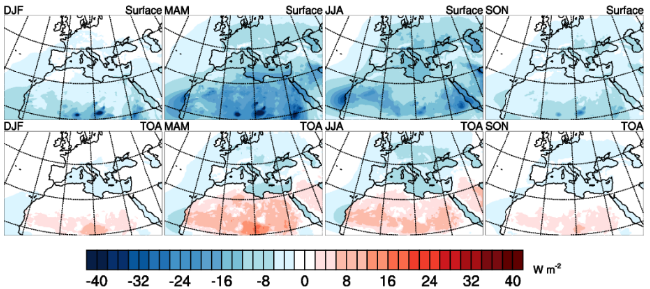
Figure 8. Mean SW DRF ( W m^{-2} ) of all aerosols over the period 1971-2000 at the surface and at the TOA.
