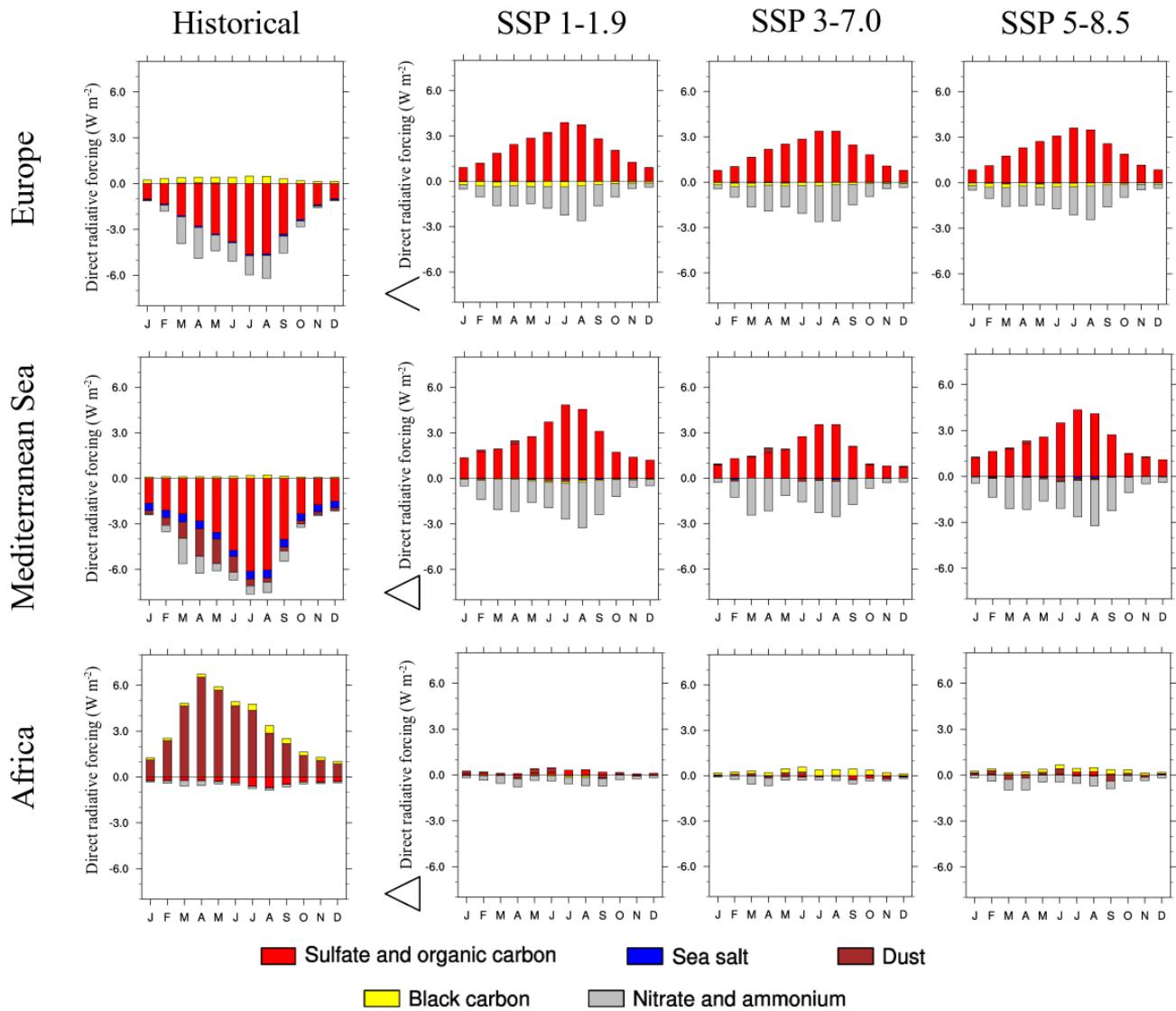
Figure A3. SW DRF evolution ( W m^{-2} ), at the TOA, of sulfate and organic carbon (in red), sea salt (in blue), dust (in brown), black carbon (in yellow) and nitrate and ammonium (in grey) between the historical period (1971-2000) and the future period (2021-2050) according to SSPs 1-1.9, 3-7.0 and 5-8.5.
