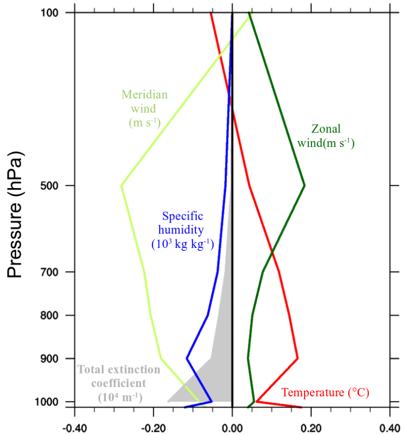
Figure 16. Vertical profile, obtained by the difference between SSP585 and SSP585cst simulations, of the temperature (°C), the total extinction coefficient (10 4 m -1 ), the meridional and zonal wind (m s -1 ) and the specific humidity (10 3 Kg Kg -1 ) over the Iberian Peninsula for the months of June, July and August.
