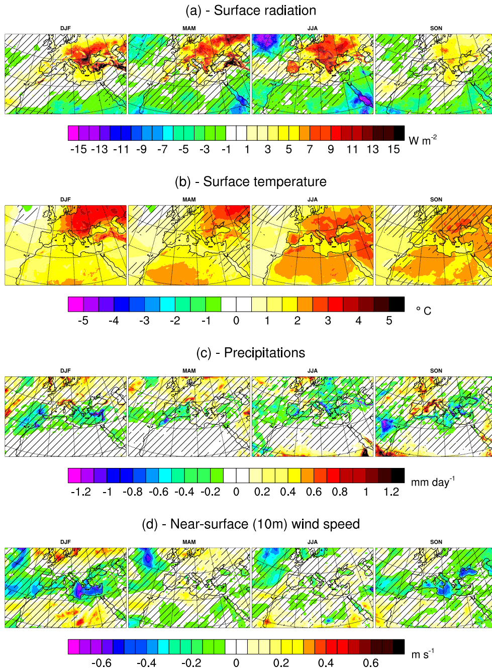
Figure 11. Surface radiation ( W m^{-2} , a), surface temperature ( ^{\circ}C , b), precipitation ( mm day^{-1} , c) and surface wind speed ( m s^{-1} , d) evolution between the period 1971-2000 and 2021-2050 for the SSP 5-8.5. The hatched areas are statically non significant with a threshold of 10%.
