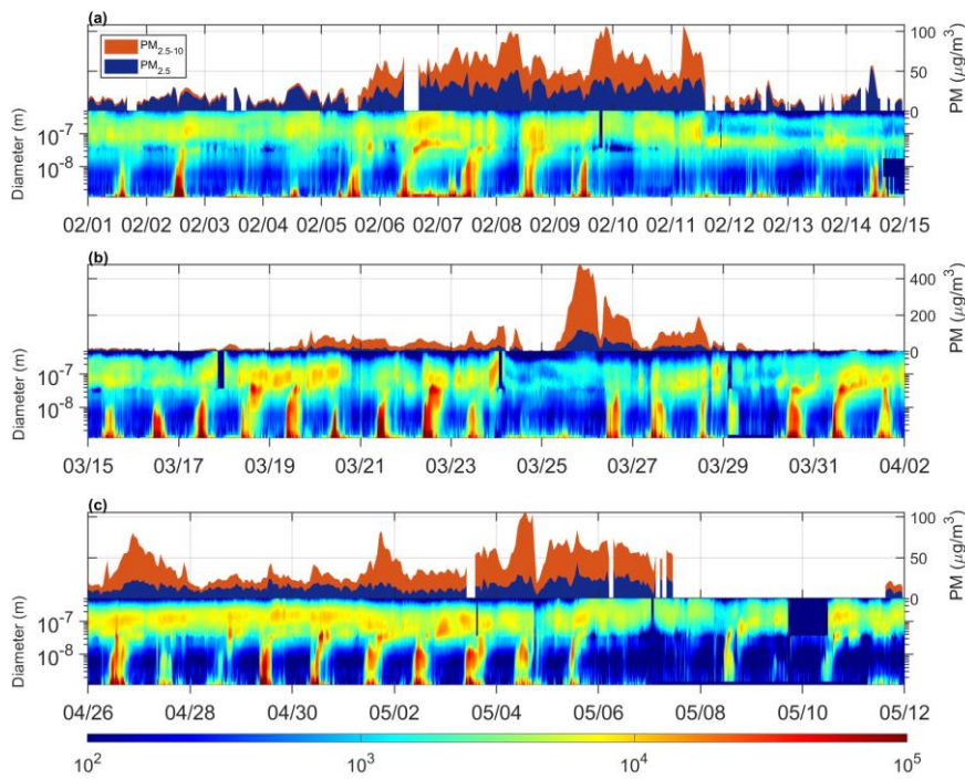
Figure 10. Temporal variations of aerosols during dust episodes with 5 days before and 5 days after the dust episode. (a) Time series of particle size distribution, PM_{10} , and PM_{2.5} between Feb 1, 2018 and Feb 15, 2018 (dust episode: Feb 6 to Feb 10). (b) Time series of particle size distribution, PM_{10-2.5} (coarse PM), and PM_{2.5} between Mar 15, 2018 and Apr 2, 2018 (dust episode: Mar 20 to Mar 28). (c) Time series of particle size distribution, PM_{10} , and PM_{2.5} between Apr 26, 2018 and May 15, 2018 (dust episode: Apr 26 to Apr 27 and May 1 to May 7 ).
