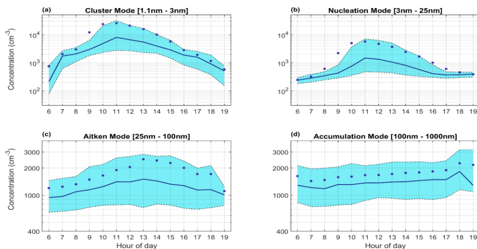
1 Figure 3. The diurnal cycle (at radiation >50 \text{ W. m}^{-2} ) of particle number concentration of Cluster mode (a), 2 Nucleation mode (b), Aitken mode (c), and Accumulation mode (d). The shaded areas with black dashed 3 boundaries represent the 25 th and 75 th percentile limits while the solid line represents the median and the 4 squares indicate the mean. Notice the difference in the y-scale between the top and bottom plots.
