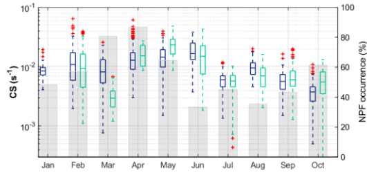
Figure 14. Monthly variation of condensation sink ( \text{s}^{-1} ) during event (blue) and non-event (green) days using data corresponding to global radiation is greater than 50 \text{ W.m}^{-2} . The bottom and top edges of the box plots indicate the 25 th and 75 th percentiles, respectively. The central mark indicates the median. The whiskers extend to the most extreme data points not considered outliers, and the outliers are plotted individually using the '+' symbol. Data presented have hourly time resolution. The shaded grey bars represent the monthly NPF percent occurrence
