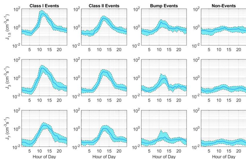
Figure 12. Diurnal variation of J1.5 (top), J3 (middle) and J7 (bottom) during class I, class II, bump events and non-events. Shaded areas represent the 25 th and 75 th percentile bounds while the solid line represents the median.
