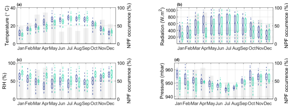
Figure 15. Monthly variation of metrological parameters during event (blue) and non-event (green) days: (a) temperature, (b) global radiation, (c) relative humidity, (d) pressure, (e) wind speed, and (f) wind direction using data corresponding to global radiation greater than 50 \text{ W.m}^{-2} . The bottom and top edges of the box plots indicate the 25 th and 75 th percentiles, respectively. The central mark indicates the median. The whiskers extend to the extreme data points not considered outliers. Data presented have hourly time resolution. The shaded grey bars represent the monthly NPF percent occurrence
