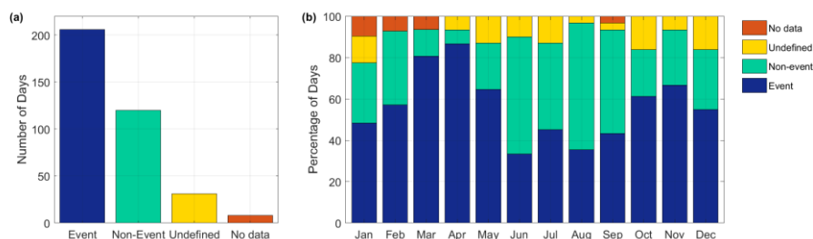
5 6 Figure 4. Classification of NPF events presented (a) annually and (b) monthly.
