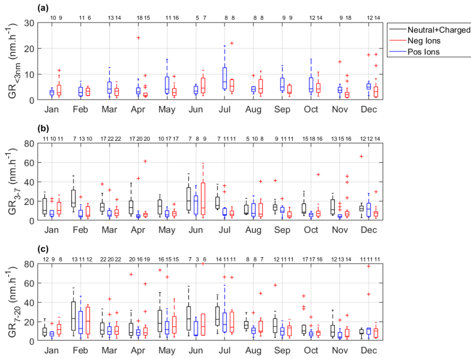
Figure 13. Monthly variation of growth rates during NPF events in three size ranges: (a) <3nm, (b) 3-7nm, and (c) 7-20nm. The central marks indicate the median, the bottom and top edges of the big box indicate the 25th and 75th percentiles, respectively. The whiskers extend to the most extreme data points not considered outliers, and the outliers are plotted individually using the '+' symbol. The numbers above the box plot represent the number of data points within each boxplot. Black boxes represent the total particles (neutral+charges), blue boxes represent negative ions and red boxes represent positive ions.
