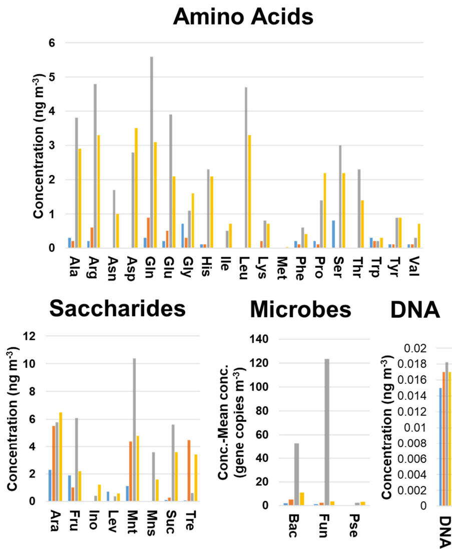
Figure 2. Comparison of the concentration profiles obtained for the different chemical and microbiological species and total DNA found in the filters as a function of the particle size. ■, <math>< 1.0 \mu\text{m}</math> particles; ■, 1.0–2.5 <math>\mu\text{m}</math> particles; ■, 2.5–10.0 <math>\mu\text{m}</math> particles; and ■, > 10 <math>\mu\text{m}</math> particles. Bac, bacteria; Pse, Pseudomonas ; and Fun, fungi.
