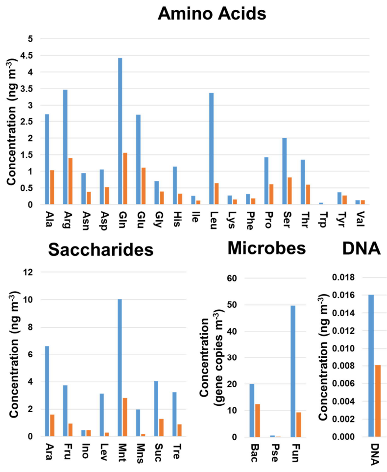
Figure 3. Differences in the chemical and microbiological composition of the PBAPs-biogenic aerosols according to the sampling period. Average concentrations were calculated for all filter sizes analyzed. ■ Sampling period 1 (04.09.2017 to 13.10.2017) and ■ Sampling period 2 (23.10.2017 to 22.11.2017). Bac, bacteria; Pse, Pseudomonas ; and Fun, fungi.
