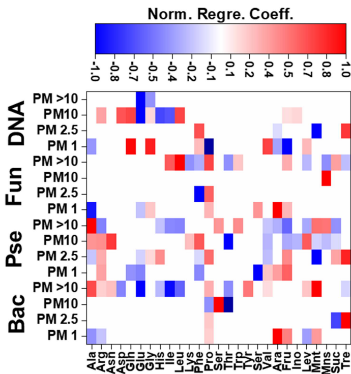
Figure 4. Normalized regression coefficient obtained for the MLR models developed for the potential elucidation of chemical signals fingerprints from microbes in the PBAP-biogenic aerosol particles. Maximum normalization was applied in all the cases. Bac, bacteria; Pse, Pseudomonas ; and Fun, fungi.
