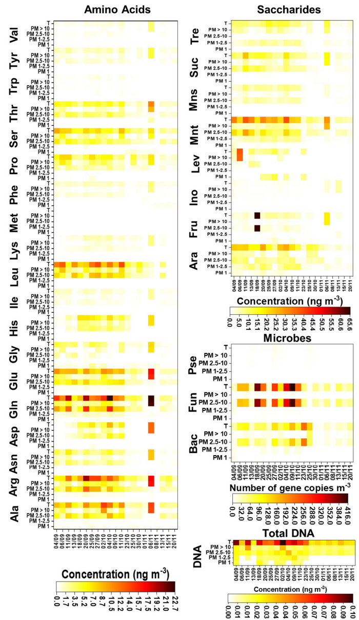
Figure 1. Chemical and microbiological composition of the analyzed filters. Start sampling day was represented in x-axis. Bac, bacteria; Pse, Pseudomonas ; and Fun, fungi.
