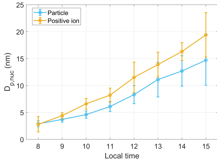
Fig. 5. The time evolution of geometric mean diameter of nucleation mode ( D_{p,nuc} ) of neutral particle and positive charged ions during the NPF events. The circle and bar present the mean value and the
