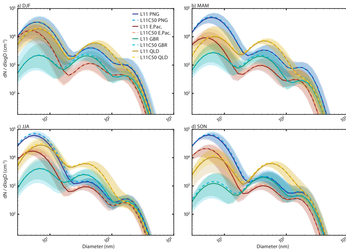
Figure 6. Aerosol dry diameter in nm (x-axis) and number concentration (as a function of number over the log of the diameter) in \text{cm}^{-3} (y-axis), both in log scales, for four regions: off the coast of PNG (blues), in the East Pacific (reds/oranges), over the GBR (green/turquoise) and inland QLD (yellow/brown), for the L11C50 (dashed lines) and L11 simulations (solid lines) (see Figure 1b for regions), for four seasons DJF (a), MAM (b), JJA (c), SON (d). The lines show the ensemble mean for the free running simulations and the shaded regions show the range of results from all years in the ensemble
