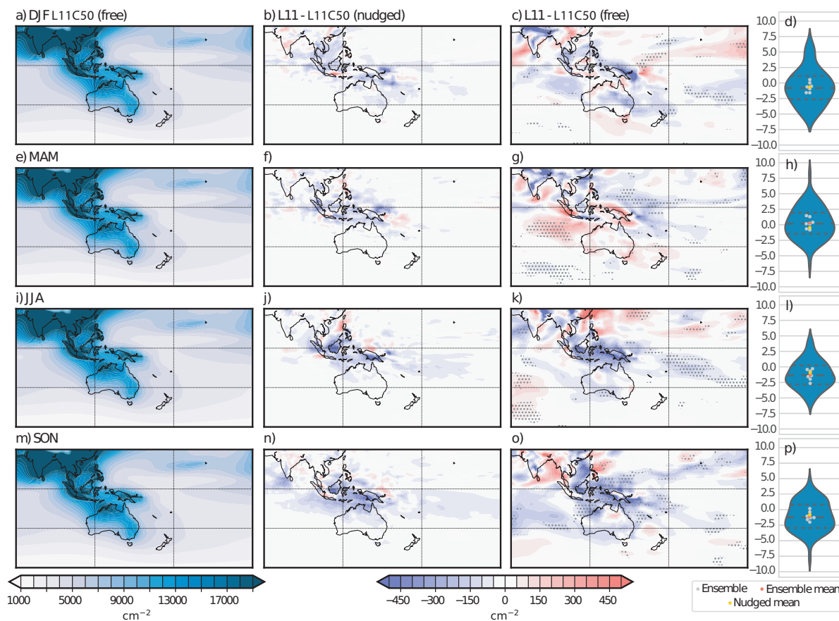
Figure 7. The seasonal (DJF - top row, MAM - upper middle row, JJA - lower middle row and SON - bottom row) total column CCN_{70} concentration (in cm^{-2} ) over the broad MC-Aus region for the free L11C50 simulation (left column); the L11-L11C50 difference for the nudged simulations (middle left column); and the L11-L11C50 difference for the free running ensemble (middle right column) with the model agreement shown by stippling, where at least five of the seven ensemble pairs agree in the sign of the difference. The right column shows violin plots of the average seasonal difference (L11-L11C50) in total column CCN_{70} over the MC-Aus region as a percentage, where all years in the ensemble is shown by the distribution, the dashed lines represent the 25, 50 and 75th percentiles, the grey dots show the mean of each pair of models, the red dots the ensemble average and the yellow the nudged average
