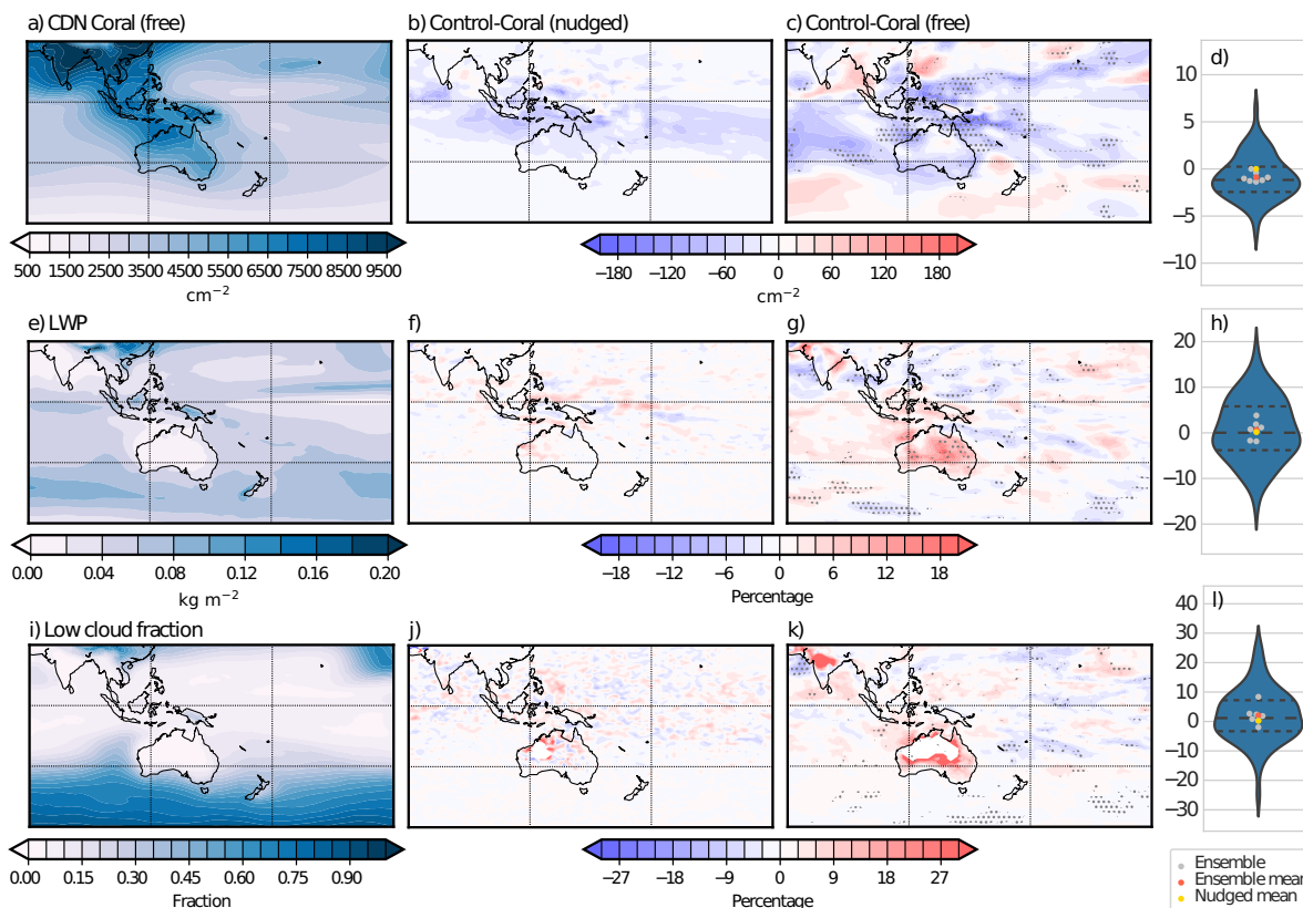
Figure 10. As for Figure 8 but for column integral of CDN (top row) in \text{cm}^{-2} , LWP (middle row) in \text{kg m}^{-2} and percent and low cloud fraction (bottom row) as a fraction and in percent
