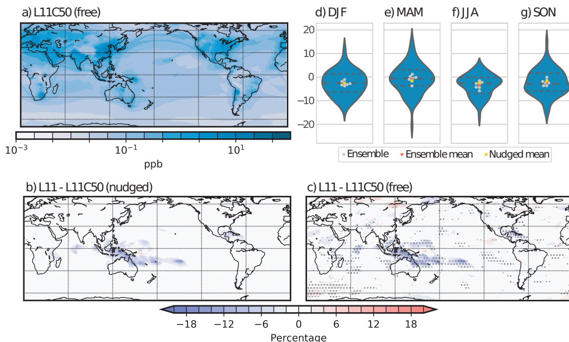
Figure 4. As for Figure 3 but for SO 2 in parts per billion (ppb) (a) and percent (b-g)
