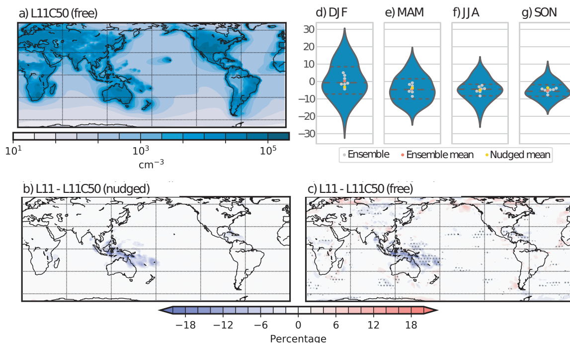
Figure 5. As for Figure 3 but for N_3 number concentration in \text{cm}^{-3} (a) and percent (b-g)
