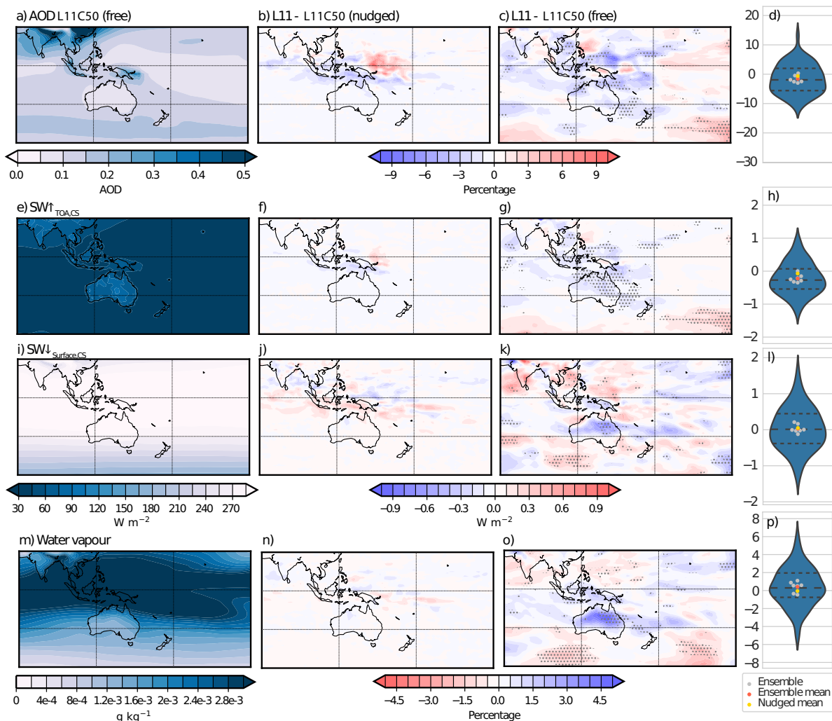
Figure 8. SON averages over the MC-Aus region for top row: the AOD (unitless and changes in percentage); upper middle row: SW\uparrow_{TOA,CS} ( W m^{-2} ); lower middle row: SW\downarrow_{Surf,CS} ( W m^{-2} ); and bottom row: column average specific humidity ( g kg^{-1} and percent). The left column shows the free L11C50 simulation; the middle left column shows the L11-L11C50 difference for the nudged simulations; the middle right column shows the L11-L11C50 difference for the free running ensemble with the model agreement shown by stippling, where at least five of the seven ensemble pairs agree in the sign of the difference; and the right column shows violin plots of the average seasonal differences (L11-L11C50) as a percentage for AOD and specific humidity and in W m^{-2} for SW\uparrow_{TOA,CS} and SW\downarrow_{Surf,CS} , where all years in the ensemble are shown by the distribution; the dashed lines represent the 25, 50 and 75th percentiles; the grey dots show each pair of models mean, the red dot the ensemble average and the yellow the nudged average
