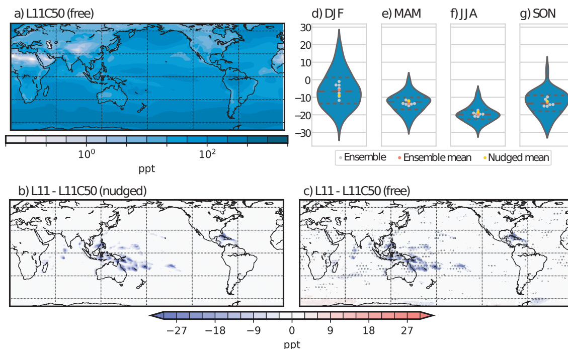
Figure 3. The annual \text{DMS}_a concentration (ppt) for the L11C50 simulation (a) and the L11-L11C50 difference for the nudged simulations (b) and free running ensemble (c). In c) the model agreement, where at least five of the seven ensemble pairs agree in the sign of the difference, is shown by stippling. d-g) show violin plots of the average seasonal difference (L11-L11C50) in \text{DMS}_a over the MC-Aus region as a percentage, where all years in the ensemble is shown by the distribution, the dashed lines represent the 25, 50 and 75th percentiles, the grey dots show each pair of models mean difference, red represents the ensemble average and yellow represents the nudged average
