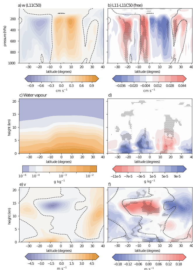
Figure 9. The zonal mean vertical profiles over the MC-Aus longitudinal region for vertical velocity ( w , top row) in \text{cm s}^{-1} , water vapour (middle) in \text{g kg}^{-1} and the v component of wind (bottom) in \text{m s}^{-1} for the free running L11C50 simulation (left column) and the difference in L11-L11C50 the free ensemble (right column), with the model agreement shown by stippling where at least five of the seven ensemble pairs agree in the sign of the difference. For a-b) and (e,f), the black dashed lines in all plots represent the zero contour of the L11C50 field, while in b) and f) the solid grey line indicates the zero contour of the L11 field
