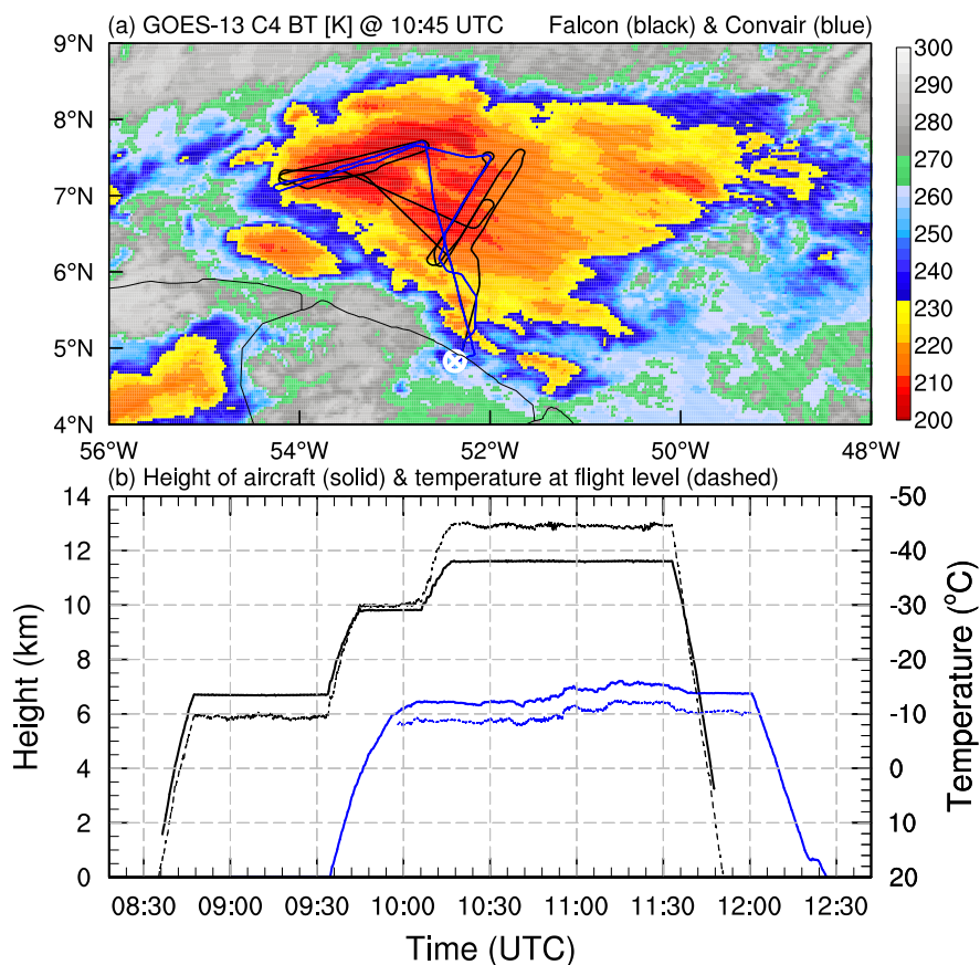
Figure 1. (a) Observed brightness temperature (K, shaded) from GOES-13 geostationary satellite channel 4 ( 10.8 \mu\text{m} ) at 1045 UTC 26 May 2015 and flight tracks of SAFIRE Falcon 20 (black thick line) and NRC Convair 580 (blue thick line). (b) Height (km, thick solid curves) of aircraft above mean sea level and air temperature ( ^{\circ}\text{C} , thin dashed curves) at the flight level for SAFIRE Falcon 20 (black) and NRC Convair 580 (blue). The white mark “ \otimes ” in (a) represents the location of the release of a radiosonde at Cayenne.
