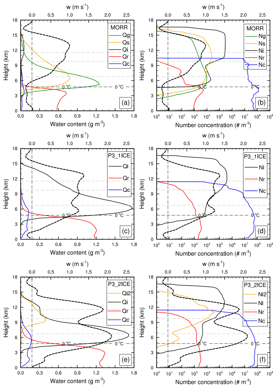
Figure 12. Vertical profiles of averaged water content (a, c and e, solid curves, \text{g m}^{-3} ) and total number concentration (b, d, and f, solid curves, \# \text{m}^{-3} ) of each hydrometeor category in MORR (a and b, cloud water: blue, rain water: red, cloud ice: black, snow: orange, and graupel: green), P3-1ICE (c and d, cloud water: blue, rain water: red, and cloud ice of first category: black) and P3-2ICE (e and f, cloud water: blue, rain water: red, cloud ice of first category: black, and cloud ice of second category: orange). The thick black dashed lines represent vertical profiles of vertical velocity ( \text{m s}^{-1} ). The vertical thin black dashed lines indicate vertical velocity of 0 \text{ m s}^{-1} . The horizontal thin black and gray dashed lines indicate the heights of temperatures at 0 , -10 , -30 , and -45^\circ\text{C} from bottom to top, respectively. The numbers of samples used to calculate the averages are shown in Table 2.
