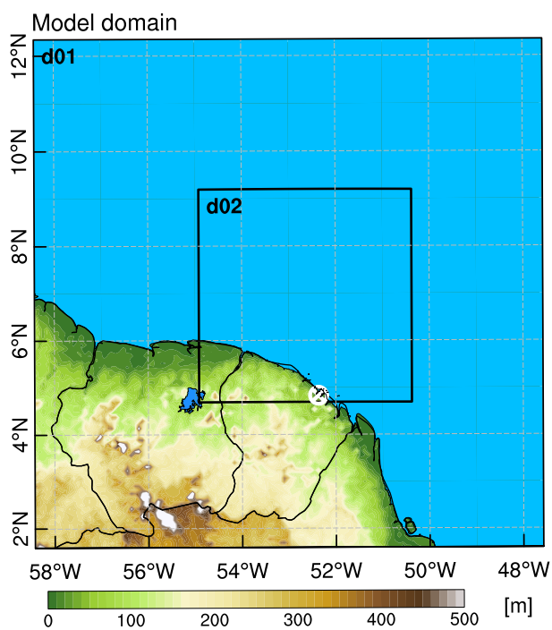
Figure 2. The model domain configuration (color shaded fields represent terrain elevation, in m). The horizontal grid spacings of d01 and d02 are 3 and 1 km, respectively. The white mark “⊗” represents the location of the release of a radiosonde at Cayenne.
