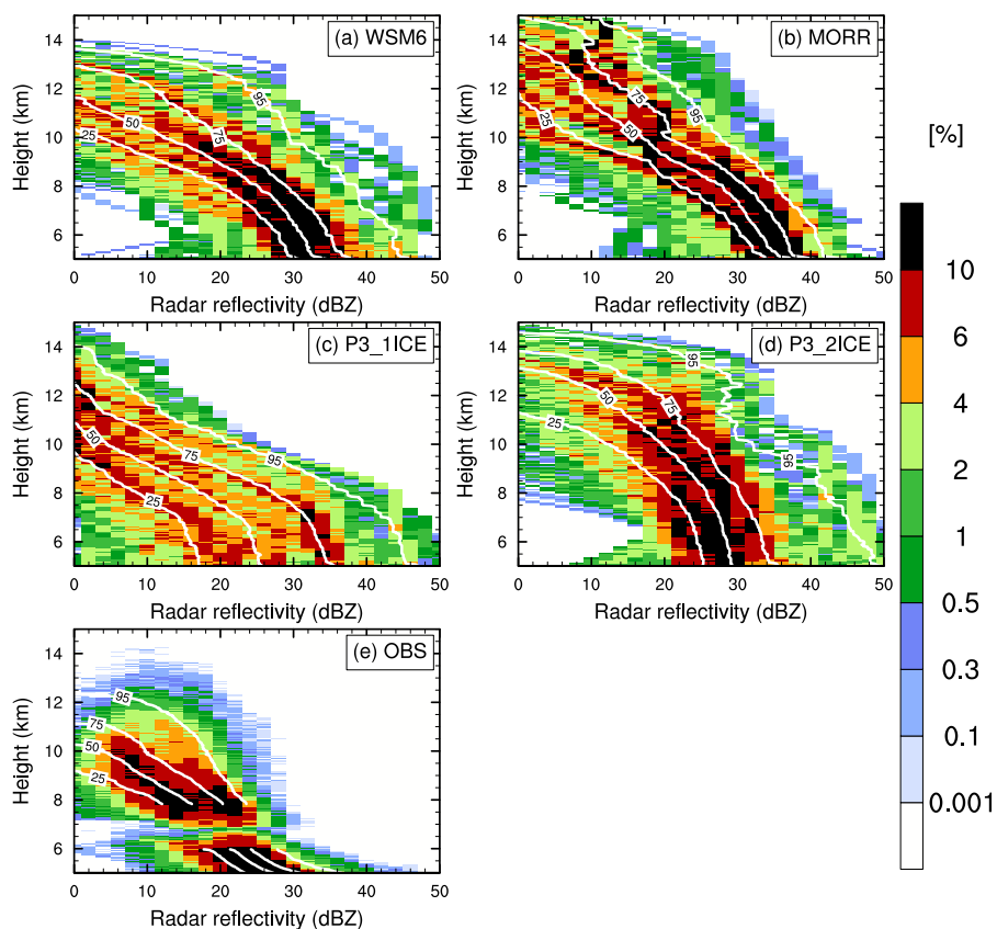
Figure 7. Frequency (% , shaded) of simulated (a: WSM6, b: MORR, c: P3-1ICE, d: P3-2ICE) and observed (e) X-band radar reflectivity. Contours represent cumulative frequencies 25%, 50%, 75% and 95%, respectively. The gap at 6–7 km in (e) is due to observed radar reflectivity data not available at the first few range gates (within \sim 500 m) from the aircraft.
