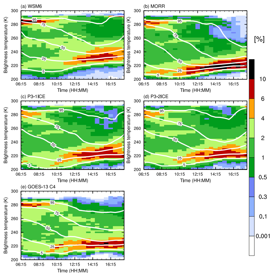
Figure 5. Frequency (% , shaded) of simulated and observed BT from GOES-13 channel 4 from 0615 to 1745 UTC 26 May 2015. Contours represent cumulative frequencies 5%, 25%, 50%, 75% and 95%, respectively.
