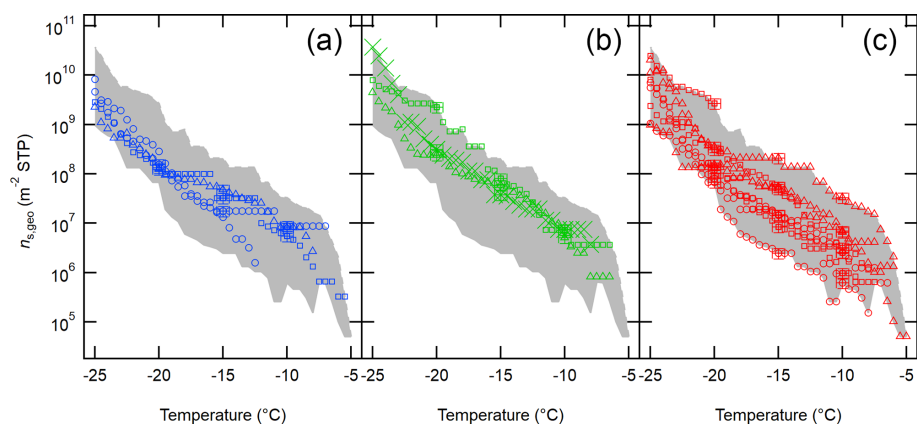
Figure 8. The n_{s,geo} spectra of OLLF aerosol particles from field ambient samples collected in 2017–2019. All downwind n_{s,geo} spectra from winter (a), spring (b), and summer (c) are shown. Different symbol shapes correspond to individual OLLF sites as indicated in the legend. The uncertainties in temperature and n_{s,geo} are \pm 0.5\text{ }^{\circ}\text{C} and \pm 23.5\% , respectively, and representative error bars are shown at -5 , -10 , and -15\text{ }^{\circ}\text{C} . The shaded area represents minimum – maximum n_{s,geo} .
