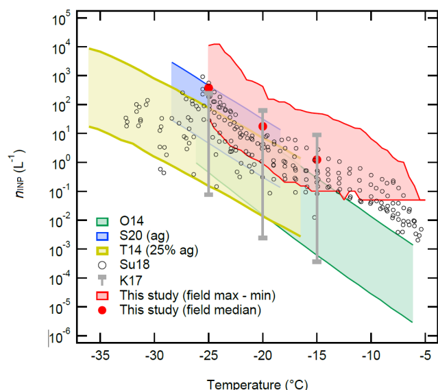
Figure 9. The n_{\text{INP}}(T) spectra of soil dust and aerosol particles as a function of temperature. The red-shaded area represents the range of our field n_{\text{INP}} values at 0.5^\circ\text{C} intervals for -5^\circ\text{C} > \text{temperature} > -25^\circ\text{C} from this study (Fig. 6). The red solid symbols are our medians at -15 , -20 , and -25^\circ\text{C} . Five reference data are adapted from O’Sullivan et al. (2014 Fig. 9; O14), Steinke et al. (2020 Fig. 3; S20), Tobo et al. (2014 Fig. 6b; T14), Suski et al. (2018 Fig. 1a–d; Su18), and Kanji et al. (2017 Figs. 1–10; K17). Note that we display the maximum and minimum at -15 , -20 , and -25^\circ\text{C} of K17 in comparison to our estimation.
