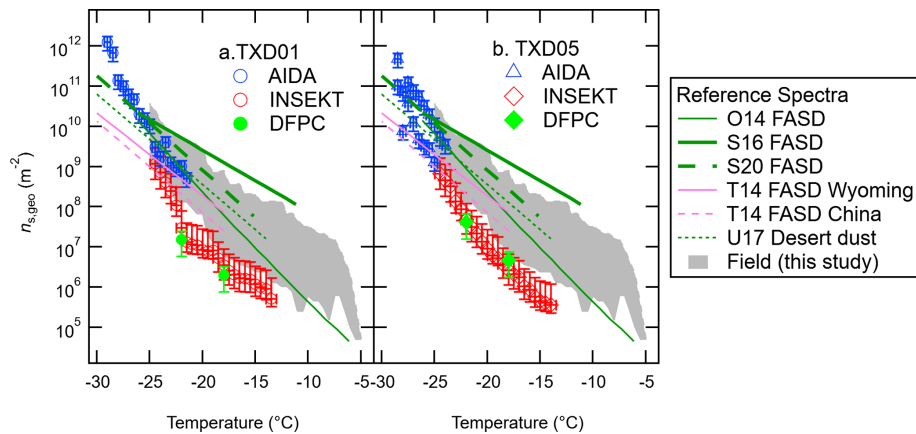
Figure 4. IN-active surface-site density, n_{s,\text{geo}} , of surface materials, TXD01 (a) and TXD05 (b), was assessed by AIDA, INSEKT, and DFPC (total aerosol particles) as a function of temperature. Six reference n_{s,\text{geo}} curves for fertile and agricultural soil dust (FASD) and desert dust are adapted from O’Sullivan et al. (2014; O14), Steinke et al. (2016; S16), Steinke et al. (2020; S20), Ullrich et al. (2017; U17), and Tobo et al. (2014; T14). The grey-shaded area represents the range of our field n_{s,\text{geo}} values at a 0.5 °C interval for -5\text{ °C} > \text{temperature} > -25\text{ °C} (Fig. 8).
