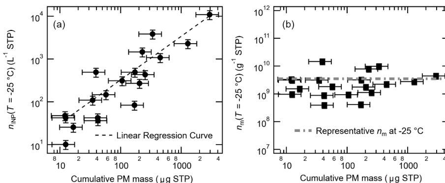
Figure 7. Correlation between cumulative PM mass vs. n_{\text{INP}} (a) and vs. n_{\text{m}} (b) at -25 °C; a linear regression curve in log scale ( n_{\text{INP}} = 3.51 \times \text{cumulative PM mass} - 2.41 ; r = 0.94 ) is shown in (a), and the constant value of representative n_{\text{m}} at the given temperature ( 3.55 \times 10^9 \text{ g}^{-1} ), which is a median n_{\text{m}} value of minimum – maximum, is shown in (b). Note that the errors in cumulative PM mass are \pm 40.4 %. The uncertainty in n_{\text{INP}} and n_{\text{m}} is \pm 23.5 %.
