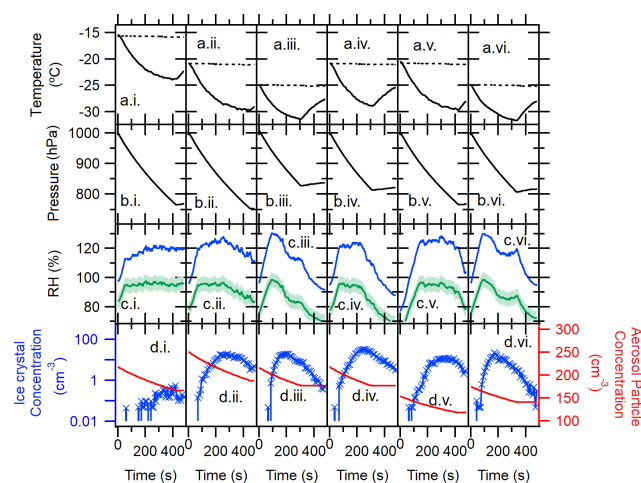
Figure 3. Temporal profiles of the AIDA immersion freezing experiment: TXDUST01_07 (i), _08 (ii), _30 (iii), _12 (iv), _13 (v), and _32 (vi). Arrays of alphabetical panels represent the chamber gas temperature (solid line) and the chamber wall temperature (dashed line) (a), pressure in the AIDA chamber vessel (b), RH with respect to water (green line) and ice (blue line) (c), and aerosol particle concentration measured by the CPC (red solid line) as well as number concentration of >20 µm D_{ve} AIDA particles measured by a welas optical particle counter (blue line) (d). Horizontal numerical panels represent different sample types and AIDA experiments, including TXD01 (i)–(iii) and TXD05 (iv)–(vi). RHs were determined with an accuracy of \pm 5 %, represented as the green shaded area in (c), using the mean gas temperature and the mean water vapor concentration.
