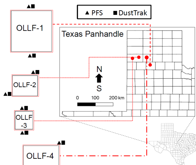
Figure 2. Schematic of the field sampling activity at individual sites (only the counties are shown). The dimension of each facility (east–west \times north–south) is (1) 1.6 \times 1.6 km, (2) 1.0 \times 0.8 km, (3) 0.7 \times 0.7 km, and (4) 0.8 \times 1.4 km TS3 . A combination of polycarbonate filter samplers (PFSs) and DustTrak instruments was used at the nominally upwind and downwind edges of OLLF-1 to OLLF-3.
