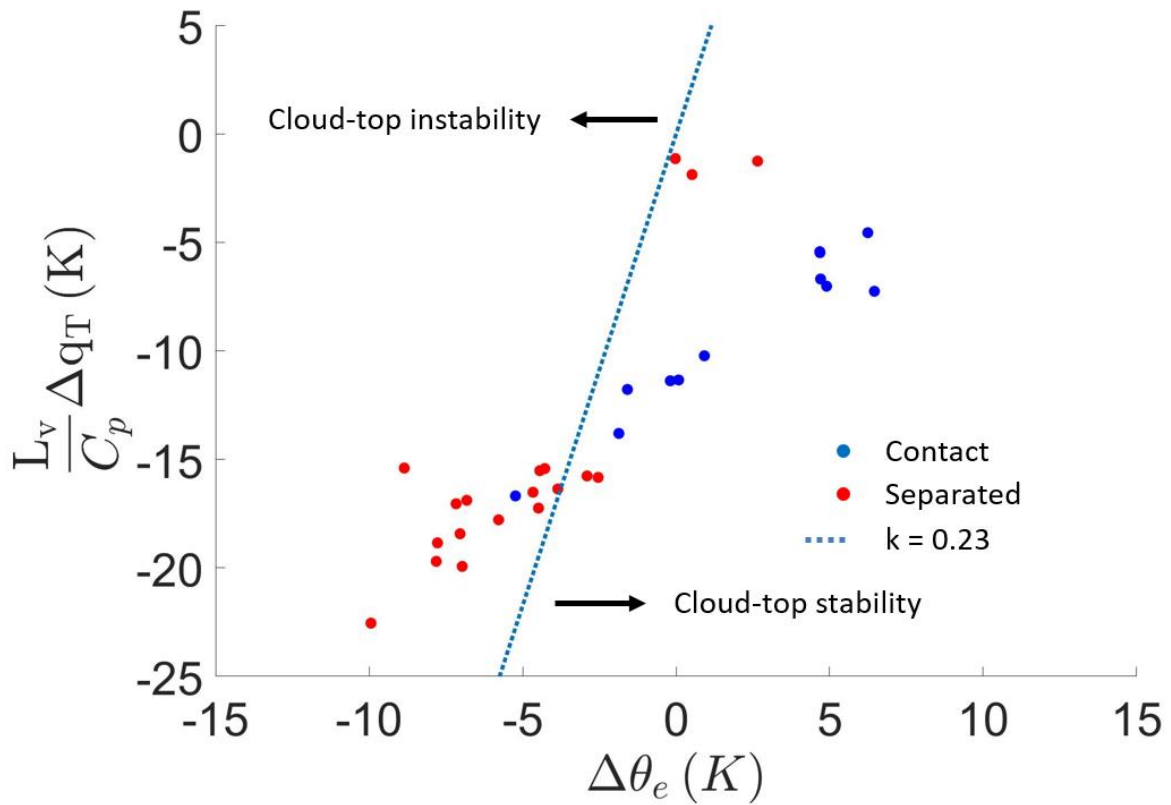
990 Figure 11: Difference between equivalent potential temperature ( \theta_e ) and total water mixing ratio ( q_T ) measured within cloud and 100 m above cloud top for contact (blue) and separated (red) profiles (only ascents through cloud shown).
