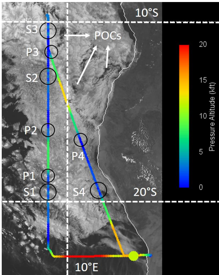
Figure 1: Visible image from the Spinning Enhanced Visible and Infrared Imager at 14:00 UTC on 6 September 2016 (PRF5), overlaid by the PRF5 flight track, and colored by flight altitude. Circles indicate sawtooth maneuver (S) and individual cloud profile (P) locations.
