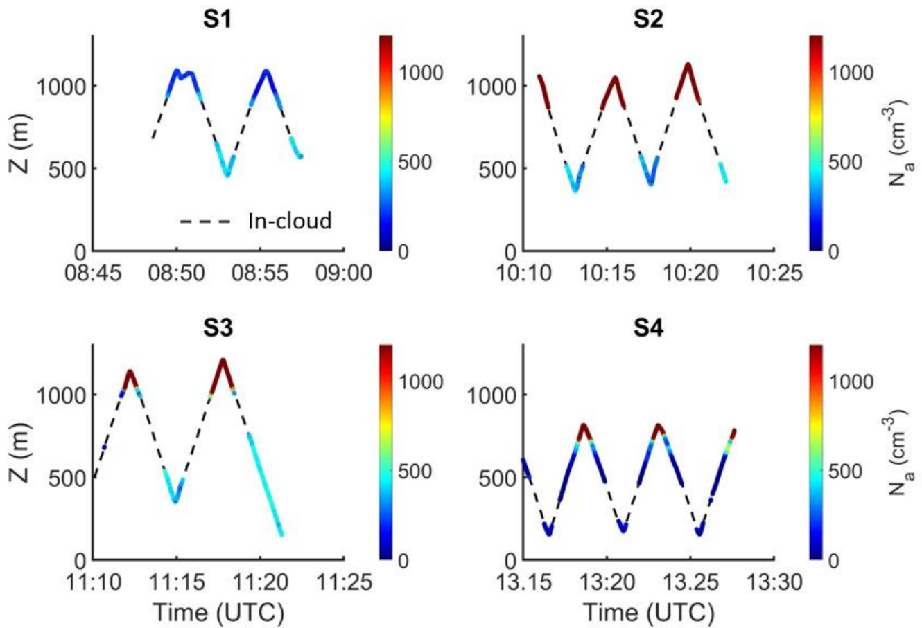
Figure 3: P-3 aircraft altitude as a function of time, colored by PCASP accumulation-mode ( 0.1 < D < 3 \mu\text{m} ) N_a for 4 sawtooth maneuvers flown on 6 September 2016. Dashed lines indicate the cloud altitudes and in-cloud N_a are masked due to potential for droplet shattering on the PCASP probe inlet.
