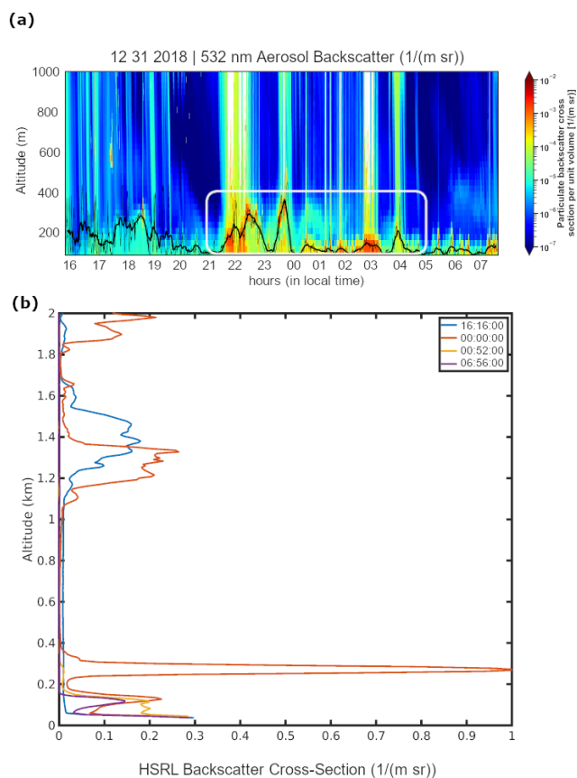
Figure 3. (a) Time series of the aerosol backscatter vertical profile from the high-spectral-resolution lidar (HSRL). The time shown is local time (UTC+8) at the Manila Observatory CEI . The times circled by the white oval correspond to the peak of aerosol backscatter in the mixing layer due to firework activity. The approximate surface-attached aerosol layer height is shown as a thick black line. It is derived from a 30 min moving window average based on the 1 min values shown as a thin black line. (b) Vertical profiles of aerosol backscatter at specific UTC times of interest before, during, and after the fireworks.
