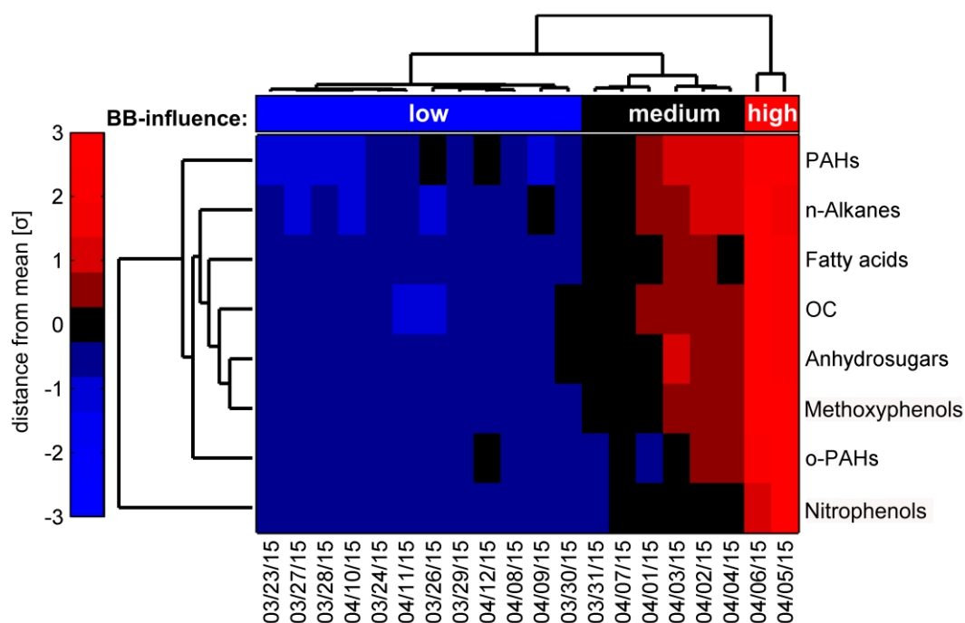
Figure 4. Clustergram based on organic composition of PM 2.5 sampled at PDI during the sampling campaign from 23 rd March to 12 th April 2015. Dendrograms indicating organic compounds and OC can be seen at the top and sampling days clustering on the left of the diagram. The colorbar on the left indicates the shades associated with values in the cells and denotes the distance to the mean in multiples of the standard deviation \sigma : Dark to bright green-blue denotes the lower values, dark to bright red the higher values and black refers to values closest to the mean.
