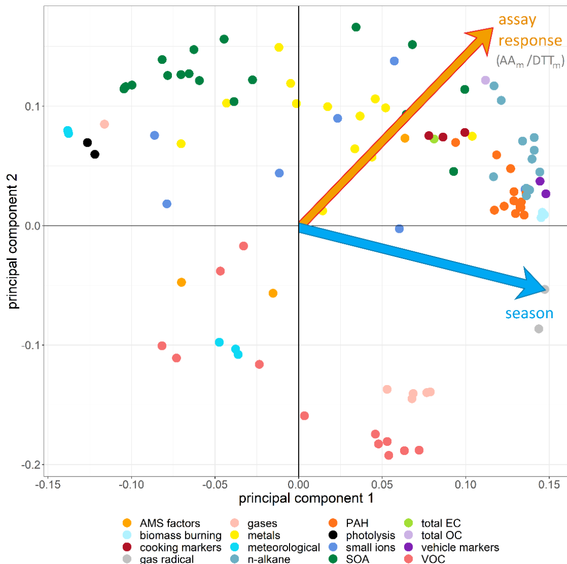
Figure 7. Principal components analysis loading plot for all data points. Points are coloured by measurement category; fully labelled loadings are provided in Figure S14 . The plot is annotated with the same orientation as the scores plot, to indicate the direction of visualised trends for selected assays and for season from the latent variable origin as shown in Figure 6 . In PC 1, the winter classification is driven by increased gas radicals, n -alkanes, PAH, vehicle markers, biomass burning markers, total OC and selected metals and SOA markers; the summer classification is driven by increased temperature and photolysis, ozone (the single gas species in this section of the plot), selected SOA markers and metals, and selected VOCs. In PC 2, high AA_m and DTT_m response is associated with increased SOA, transition metals, cooking markers, n -alkanes and PAH concentrations in samples; low AA_m and DTT_m response associated with low VOCs, gases and selected meteorological parameters (relative humidity).
