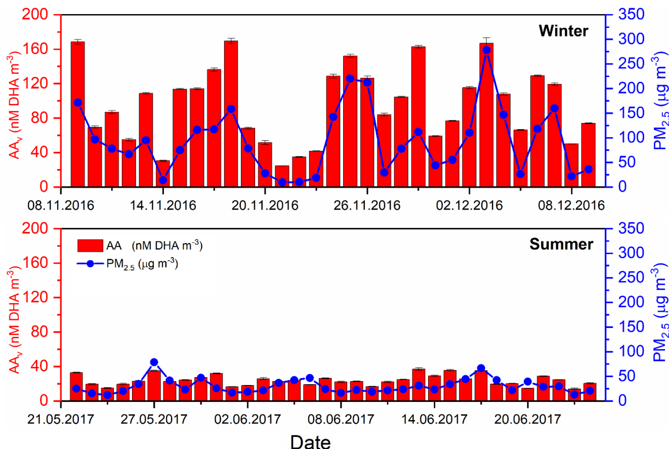
260 Figure 1. 24-hour averaged volume-normalised AA_v (red bars) and PM_{2.5} mass (blue dots), analysed from 24-hour high volume filters, for both winter 2016 (08/11/2016 – 08/12/2016) and summer 2017 (21/05/2017 - 24/06/2017) (Shi et al., 2019; Xu et al., 2020a). Substantially higher average PM_{2.5} mass concentrations ( \mu g m^{-3} ) and AA_v were observed in the winter season compared to the summer (see Table S1 for summary). DCFH v , DTT v and EPR v 24-hour averaged datasets can be found in Figures S8-S10 respectively.
