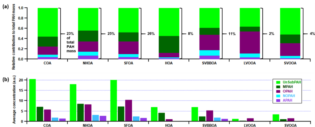
Figure 10 – Relative contribution of PAH families to total PAH factor mass (a) and the PAH family average uncalibrated concentrations (b). The PAH families: UnSubPAH, MPAH, OPAH, NOPAH and APAH, are described within section S6 and in Herring et al. (2015).
