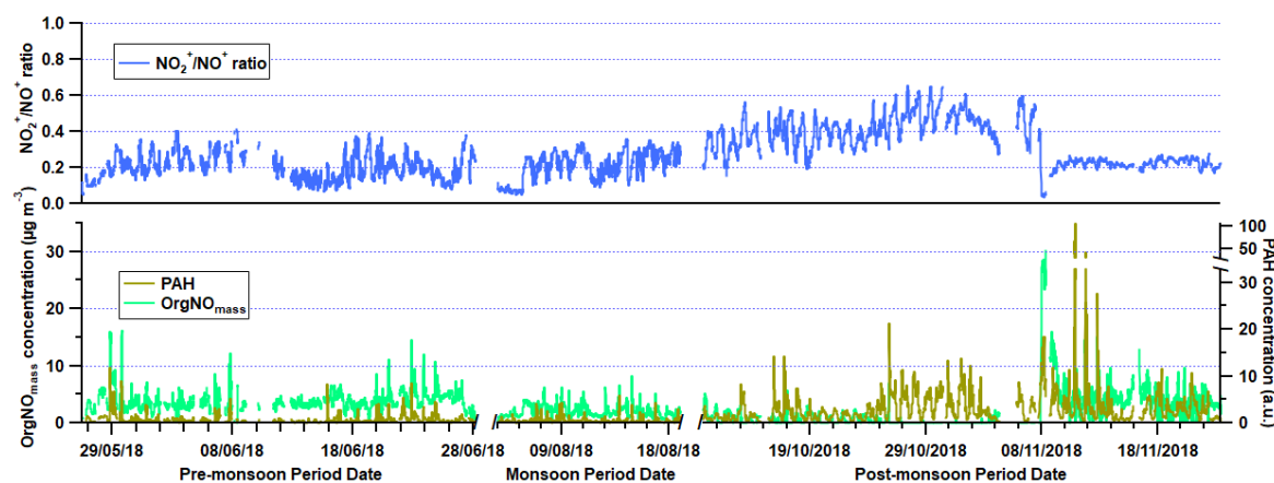
Figure 4 – Upper panel: time series of \text{NO}_2^+/\text{NO}^+ ratio in the three measurement periods. Lower panel: time series of polyaromatic hydrocarbon (PAH) uncalibrated concentrations and organic nitrogen oxide species ( \text{OrgNO}_{\text{mass}} ) concentrations.
