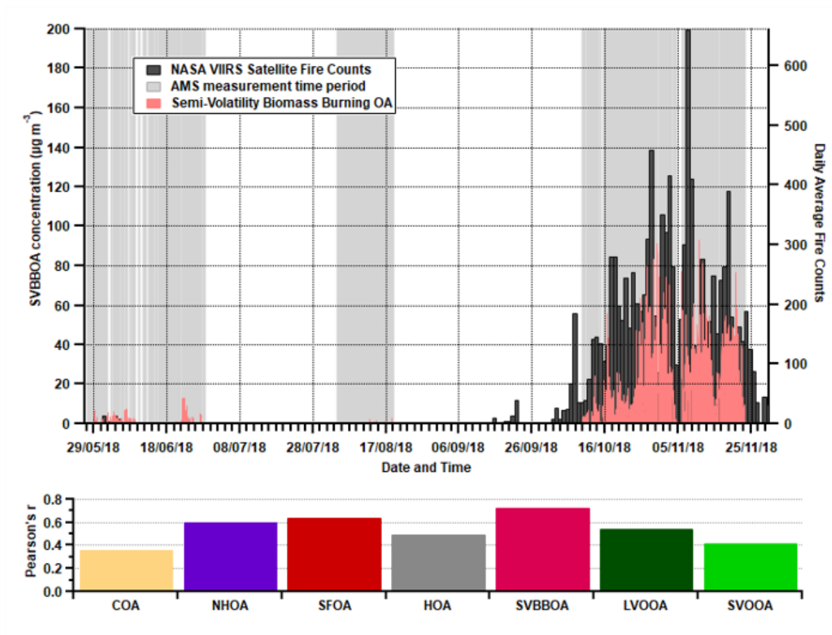
Figure 12 – Upper panel: time series for SVBBOA along with the daily average fire counts from the NASA Visible Infrared Imaging Radiometer Suite (VIIRS) sensor on the Suomi National Polar-orbiting Partnership (S-NPP) satellite. Lower panel: Pearson's r correlations between daily average factor concentrations and the daily average fire counts. The VIIRS data covers all days displayed along the x-axis while the AMS measurements cover the grey shaded regions.
