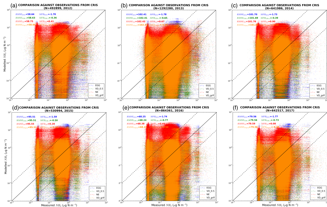
Fig. 1. Annual scatterplots of modelled versus CrIS \text{NH}_3 surface concentrations from the relevant four simulations using emissions from EGG, VD0.5, NE and VDgrff.
