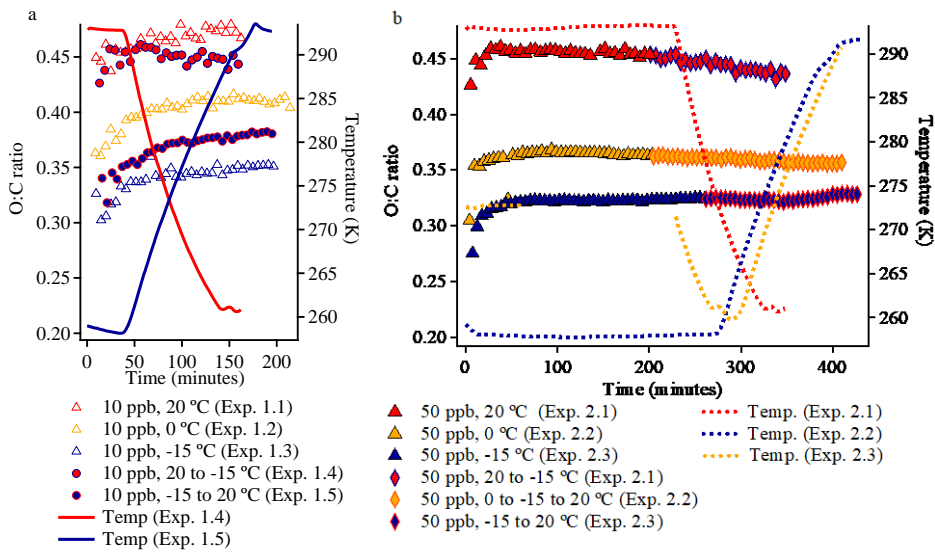
Figure 5. Time series of O:C ratio in (a) 10 ppb \alpha -pinene experiments (1.1-1.5) and (b) 50 ppb \alpha -pinene experiments (2.1-2.3).
