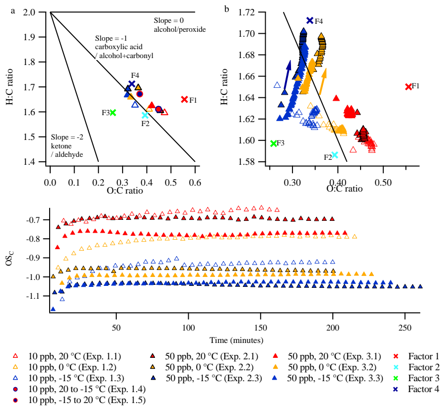
Figure 5. Van Krevelen plots (H:C ratio vs. O:C ratio) at (a) at SOA mass peak (five data point average) and in the expansion (b) during the constant temperature experiments in this work ( ←5 minutes time resolution , (arrows indicate direction of time)-), as well as (c) the OSC during the experiments . The lines in the Van Krevelen plot are based on Heald et al. (2010) and Ng et al. (2011). Notice the different scales of the axes in panels a and b. The positions of the four factors obtained from the PMF analysis are indicated by crosses: F1: Factor 1 (high temperature), F2: factor 2 ( low concentration ), F3: Factor 3 (high concentration), F3: Factor 3 (low concentration) , and F4: Factor 4 (low temperature). Panel b and c show every fifth data point. Standard errors are shown in S25 and S26.
