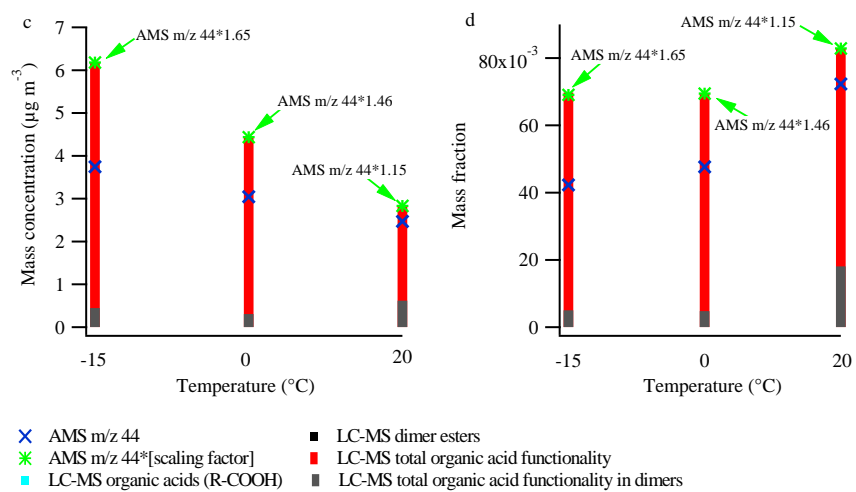
Figure 7. LC-MS derived organic acid (R-COOH) mass concentration (panel a) and organic acid mass fraction (panel b) at -15, 0, and 20 °C. The organic acid functionality (-COOH) mass concentration and mass concentration at the three temperatures are shown in panels c and d respectively. Additionally the corresponding results related to dimers are shown. The panels also show m/z 44 - a tracer of organic acids - from the AMS mass spectra and the scaling factors to be applied to reach the level of organic acid (functionality) measured by the LC-MS. The particle filter samples analyzed by the LC-MS are obtained by the end of the experiments (see Table 1) while the AMS results are obtained right before the filter sampling, 10 minutes average). The figure is based on data from experiments 3.1-3.3.
