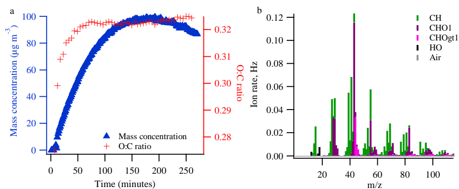
10 Figure 1. (a) Evolution of SOA mass (density corrected), density, and O:C ratio during a typical experiment (50 ppb \alpha -pinene, -15 °C, experiment 2.3) and (b) mass spectra of the experiment obtained at mass peak (5 minutes average). gt means greater than.
