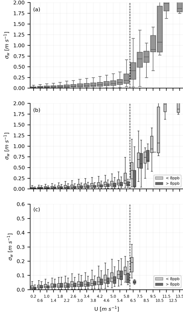
Figure 10. Standard deviation ( \sigma_w ) of the vertical velocity, plotted against the mean wind speed, for 1-minute averaging time. On the top panel (a), the variability of \sigma_w for each wind speed bin is shown for all data points, with no classification based on \text{CH}_4 gradients. On (b), the same as (a) is shown, but separating between measurements with gradients above and below 8 ppb. Note that our \text{CH}_4 mixing ratio measurements are at 15-minute resolution, therefore we assume the same value every 15-minute window so we can associate the 1-minute \sigma_w and U with \text{CH}_4 mixing ratios. On the bottom panel (c), we excluded the 15-minute time periods where the wind speed varied by more than 0.5 \text{ m s}^{-1} . Note the difference in y-axis for (c). The wind speed bins are shown every 0.4 \text{ m s}^{-1} until 5.8 \text{ m s}^{-1} , after the spacing is 1 \text{ m s}^{-1} . This gradually increase to coarser wind speed bins is done due to less amount of data at higher wind speeds. High-frequency measurements cover six months of 2014: March, April, May, July, August and September.
