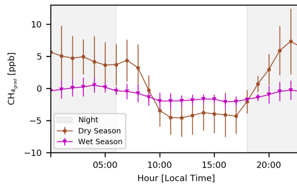
Figure 6. Mean diurnal cycle of the \text{CH}_4 gradient between the 79 m and 4 m levels. The period between June 2013 and November 2018 was used and separated by dry and wet seasons. The error bars show the standard deviations
