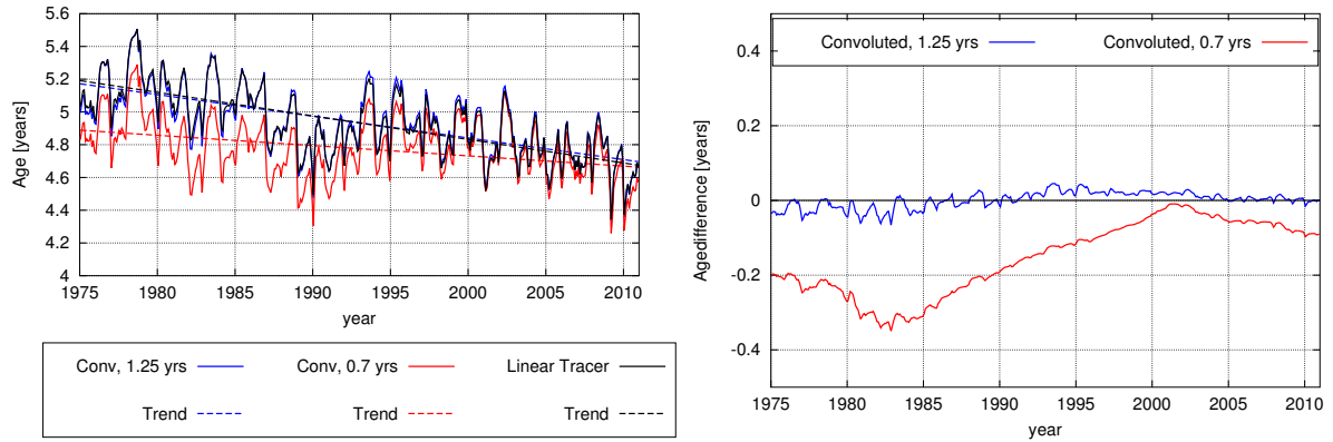
Figure 15. Left, mean AoA and its trend derived from SF 6 using the convolution method for 0.7 and 1.25 years ratio of moments (red and blue) and from the linear tracer (black) at 20 hPa and 40°N from 1975 to 2011 from the RC1-base-07 simulation. Right, the difference in mean AoA derived from SF 6 and the linear tracer.
