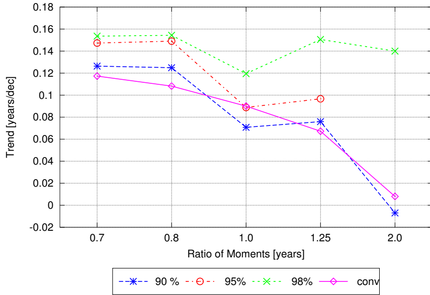
Figure 17. Trend in mean AoA derived from the observations for the fit and the convolution method for the respective fraction of input and ratio of moments.
