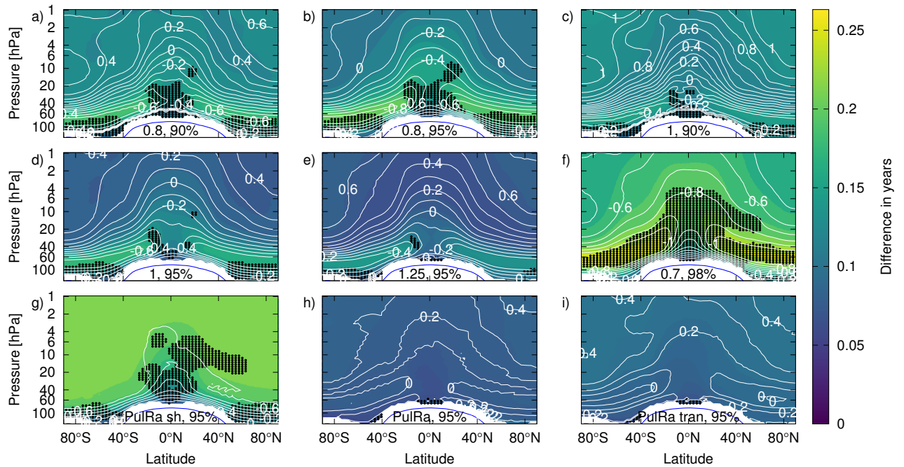
Figure 8. Mean absolute deviation of mean AoA calculated from SF6 from AoA derived from an ideal tracer for different ratio of moments and fraction of input (colors). The overlaid white contours are the difference in trends in 10^{-1} years decade ^{-1} . At the bottom of each panel, the fraction of input and ratio of moments considered in the derivation are stated. PulRa denotes the ratio of moments derived from the tranPul simulation annual mean extended age spectra, PulRa sh is from the 9.5 year spectra. PulRa tran uses the transient extended spectra from that simulation. White areas indicate where the derivation is not applicable. Black stippling show insignificance of the SF6 trend from zero on the 95% confidence level. The trend calculation considered the time series from 1975 to 2011. The tropopause and the range 30 K above are excluded, as the AoA calculation is not defined in this region due to the different entry regions into the stratosphere that have to be considered.
