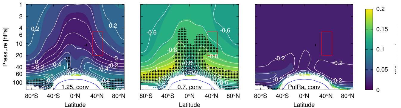
Figure 16. As Fig. 8, in color are the mean absolute deviation of mean AoA calculated from SF 6 from AoA derived from an ideal tracer for every month from 1975 to 2011 for different ratio of moments using the convolution method. The left panel is 1.25 years of ratio of moments and the middle is 0.7 years. PulRa denotes the ratio of moments derived from the tranPul simulation annual mean extended age spectra (right). The white contours are the difference in trends in 10 -1 years decade -1 . White areas indicate where the derivation is not applicable. Black stippling shows insignificance of the SF 6 trend from zero on the 95% confidence level. The trend calculation considered the time series from 1975 to 2011. The red box shows the range of the balloon observations.
