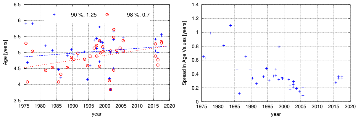
Figure 18. Left, example AoA time series derived from the observations using the stated parameters F=90%, 1.25 years ratio of moments and F=98%, 0.7 years . Right, the difference between maximum and minimum mean AoA found from the observations for the considered parameters (0.7, 0.8, 1.0 and 1.25 years for the fit and convolution method and 90%, 95% and 98% for the fit method).
