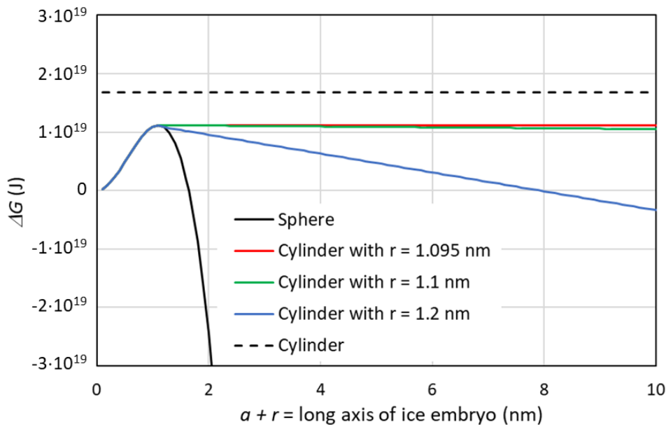
5 Figure 6. Gibbs free energy of a growing ice embryo calculated with CNT using the Ick15 parameterization for T = 230 K and P_0 = 0.1 MPa. The black solid line describes spherical growth of the ice embryo as expected in bulk water. The black dashed line gives \Delta G for the growth in length of a cylinder starting from a thin disk with radius r_c = 1.095 nm. The colored lines show \Delta G for growth in cylindrical pores with radii available for free water of 1.095 nm (critical value, red line), 1.1 nm (green line), and 1.2 nm (blue line), respectively.
