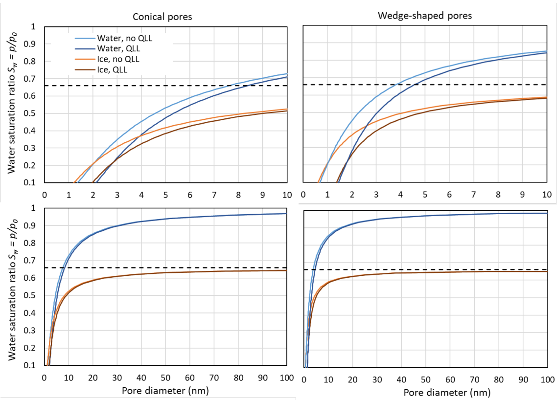
Figure 9. Comparison of pore filling with water and ice for conical (left panels) and wedge-shaped pores (right panels) at 230 K. For water and ice, the Kelvin effect is calculated without QLL, given as light blue and light brown lines, respectively, and assuming a QLL with width t = 0.38 nm, given as dark blue and dark brown lines, respectively. The black, dashed horizontal line indicates ice saturation.
