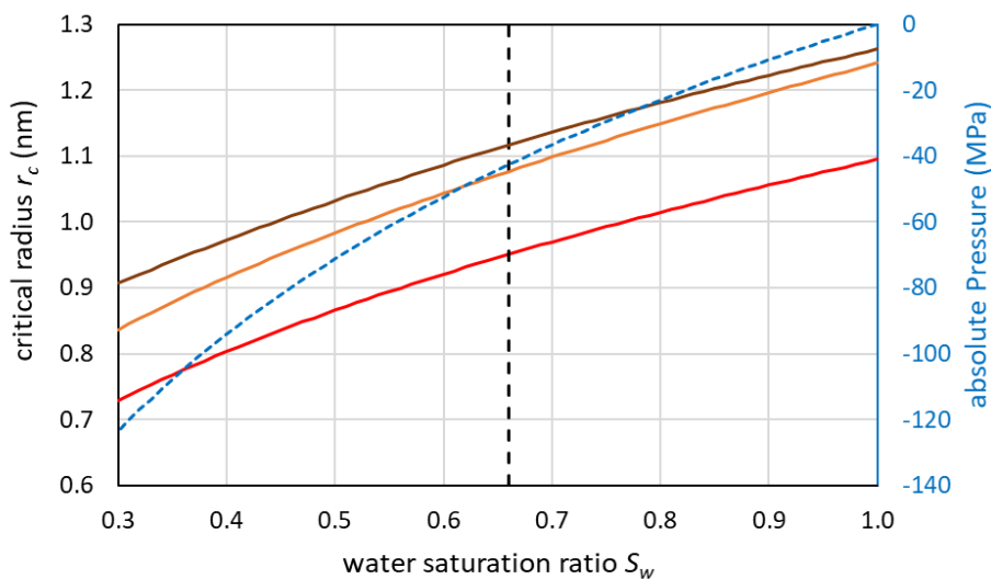
10 Figure 7. Dependence of the critical embryo radius on the water saturation ratio at 230 K for ice nucleation within pores using Ick15 (red) and Mr10 (orange: n = 0.97 ; brown: n = 0.3 ) parameterizations. Saturation with respect to bulk ice is indicated as the black dashed vertical line. The blue dashed line shows the negative pressure that builds up in pore water when the water saturation ratio decreases.
