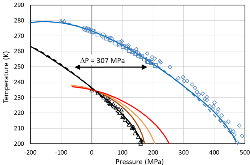
Figure 34. Pressure dependence of melting (blue) and freezing (black) temperatures of ice I. Melting point measurements of ice I are from Kanno et al. (1975) (blue squares), Mishima (1996) (blue diamonds), Henderson and Speedy (1987) (blue circles) and Roedder (1967) (blue triangles). For simplicity, melting data of other ice polymorphs are not shown. The blue solid line is the melting curve calculated by setting Eq. 24 to zero. The dashed blue line is a fit to the measured melting temperatures (blue symbols) using the equation given in Marcolli (2017b): T(K) = 557.2 - 273\exp((300 + P(\text{MPa}))^2/2270000) . Freezing temperatures of ice I (black triangles) are from Kanno et al. (1975). The black solid and dashed lines represent a homogeneous ice nucleation rate of 10^8 \text{ cm}^{-3}\text{s}^{-1} obtained by shifting the blue curves by \Delta P = 307 \text{ MPa} to lower values. Red line: Ick15 parameterization with pressure dependent chemical potential ( \Delta\mu_{iw} of Eq. 24), all other parameters without pressure dependence. Orange and brown lines: Mr10 parameterization with pressure dependent chemical potential ( \Delta\mu_{iw} of Eq. 24) with n = 0.3 (brown) and n = 0.97 (orange), all other parameters without pressure dependence. Fully pressure dependent Ick15 and Mr10 parameterizations were optimized to overlay with the experimental freezing data and are not shown here.
