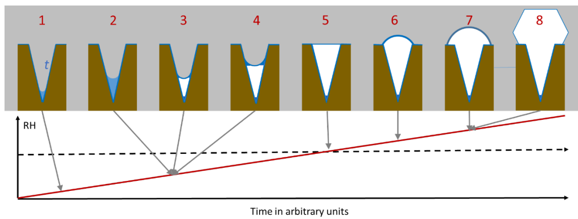
Figure 11. Pore condensation and freezing in conical or wedge shaped pores (brown) assuming continuously increasing RH (red line). The pore is assumed to be covered with a QLL of width t (darker blue) already at low RH. Free water (lighter blue) collects in pores and freezes to ice (white) that further grows within the pore. At ice saturation (dashed black horizontal line), the pore is completely filled with ice.
