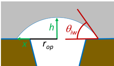
10 Figure 910. Growth of ice out of the pore as a spherical cap with an increasing height h covering an increasing area \pi(r_{op} + x)^2 .
