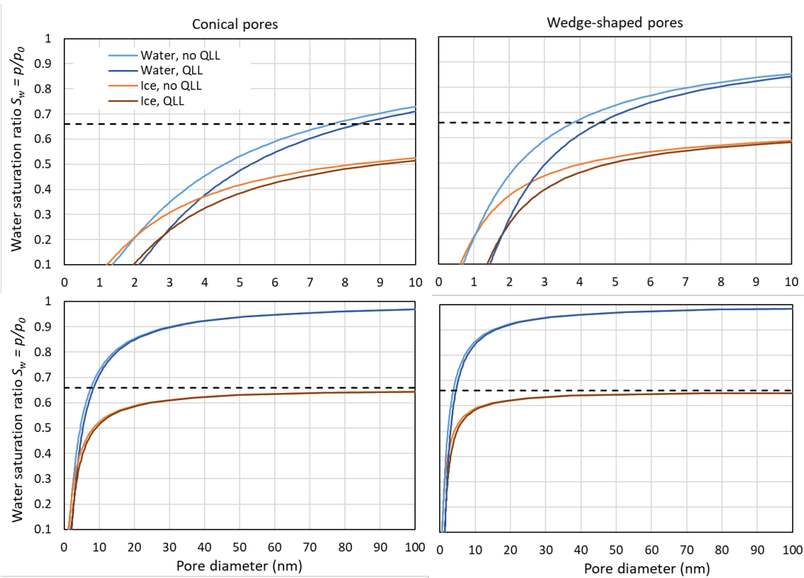
5 Figure 89. Comparison of pore filling with water and ice for conical (left panels) and wedge-shaped pores (right panels) at 230 K . For water and ice, the Kelvin effect is calculated without QLL, given as light blue and light brown lines, respectively, and assuming a QLL with width t = 0.38 nm, given as dark blue and dark brown lines, respectively. The black, dashed horizontal line indicates ice saturation.
