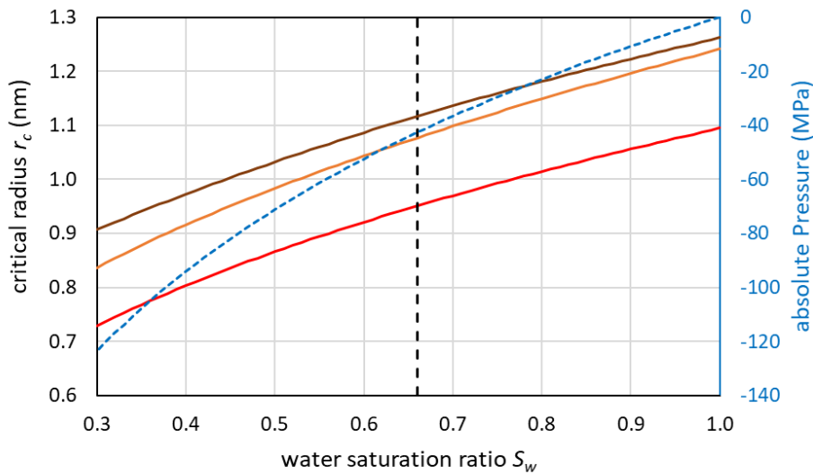
10 Figure 67. Dependence of the critical embryo radius on the water saturation ratio at 230 K for ice nucleation within pores using Ick15 (red) and Mr10 (orange: n = 0.97 ; brown: n = 0.3 ) parameterizations. Saturation with respect to bulk ice is indicated as the black dashed vertical line. The blue dashed line shows the negative pressure that builds up in pore water when the water saturation ratio decreases.
