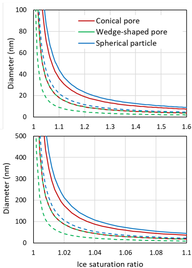
Figure 1011. Diameters of pore opening allowing barrier-free ice growth out of cylindrical or conical pores (red), wedges or trenches (green), and spherical particles (blue) as a function of ice saturation ratio. The lower panel is a zoomed in view of the upper panel. Solid lines are obtained for T = 230 K with \gamma_{vi} = \gamma_{vw} + \gamma_{iw} = 0.0811 \text{ Jm}^{-2} + 0.0226 \text{ Jm}^{-2} = 0.1033 \text{ Jm}^{-2} , \gamma_{iw} from Ick15, and \theta_{iw} = 55^\circ . Dashed lines are calculated by halving all involved interfacial tensions to account for the presence of trace amounts of organic substances that adsorb on surfaces and interfaces. Note that the dashed red line overlays the green solid line.
