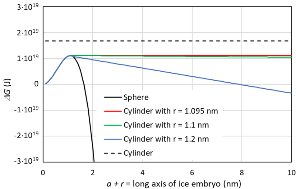
5 Figure 56. Gibbs free energy of a growing ice embryo calculated with CNT using the Ick15 parameterization for T = 230 K and P_0 = 0.1 MPa. The black solid line describes spherical growth of the ice embryo as expected in bulk water. The black dashed line gives \Delta G for the growth in length of a cylinder starting from a thin disk with radius r_c = 1.095 nm. The colored lines show \Delta G for growth in cylindrical pores with radii available for free water of 1.095 nm (critical value, red line), 1.1 nm (green line), and 1.2 nm (blue line), respectively.
