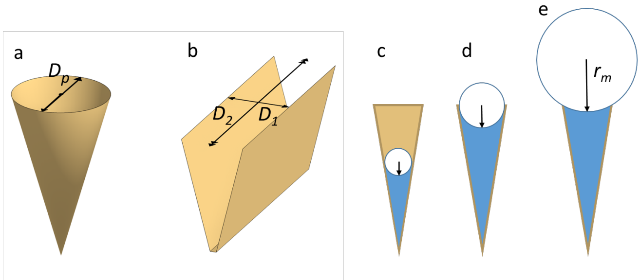
Figure 12. Illustration of pore shapes and pore filling: panel (a) shows an empty conical pore with diameter D_p and panel (b) an empty wedge-shaped pore with a width D_1 and a length D_2 = \infty . Panels (c) to (e) show pore condensation with increasing radius of the meniscus for a conical or wedge-shaped pore assuming complete wetting ( \theta_{ws} = 0^\circ ). The radius of meniscus in a conical or cylindrical pore is denoted r_m and the radius of meniscus in a wedge-shaped pore or trench is denoted r_1 = D_1/2 while r_2 = D_2 = \infty (not shown).
