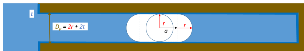
Figure 45. Ice nucleation and growth within a cylindrical pore of diameter D_p = 2r + 2t , with a describing the growth along the pore axis, t being the thickness of the QLL and r being the maximum radius the embryo can reach perpendicular to the pore axis.
