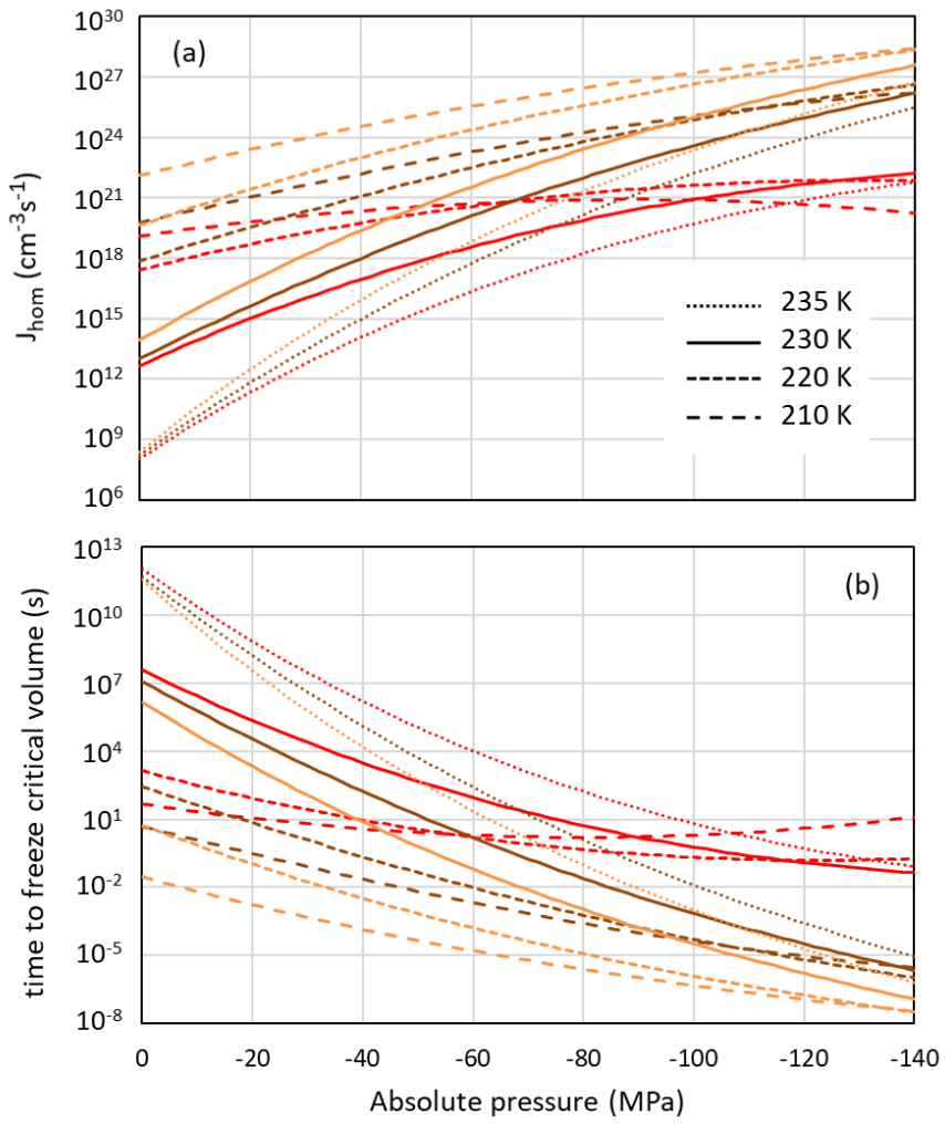
Figure 78. Pressure dependence of homogeneous nucleation rates (panel a) and the time to freeze the critical water volume for homogeneous ice nucleation (panel b) at four different temperatures as indicated in the legend. Ick15 is shown in red, Mr10 in orange for n = 0.97 and in brown for n = 0.3 .
