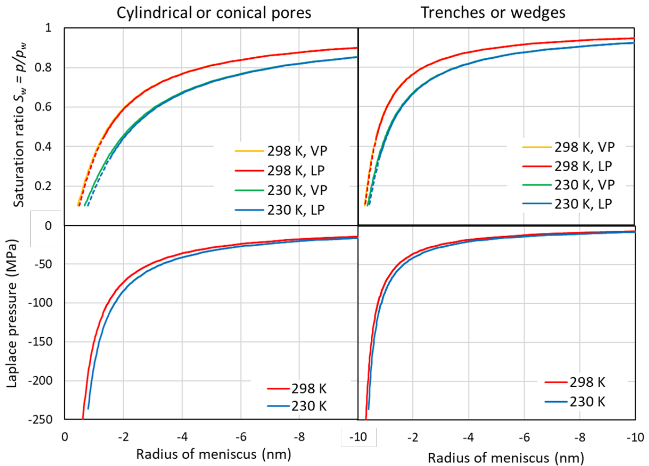
Figure 23. Upper panels: Saturation ratio as a function of the meniscus radius of cylindrical or conical pores ( r_m , left panels) and trenches or wedges ( r_t , right panels) at 298 K and 230 K. Saturation ratios are given neglecting the effect of negative pressure on the molecular volume of water (indicated as VP in the legend and calculated using Eqs. 1 and 2) and accounting for the Laplace pressure exerted on the pore water (indicated as LP and calculated using Eqs. 8 and 10). The dashed portions of the red and blue lines indicate the extrapolation of the molecular volume to strongly negative pressures as shown in the lower panels. Lower panels: Laplace pressure as a function of the radius of the meniscus.
