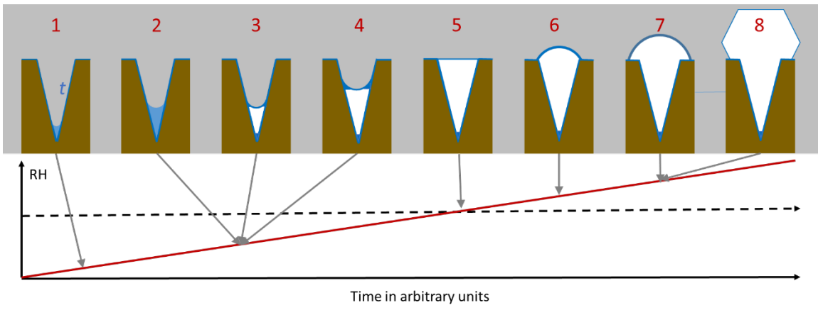
Figure 1. Pore condensation and freezing in conical or wedge-shaped pores (brown) assuming continuously increasing RH (red line). The pore is assumed to be covered with a QLL of width t (darker blue) already at low RH. Free water (lighter blue) collects in pores and freezes to ice (white) that further grows within the pore. At ice saturation (dashed black horizontal line), the pore is completely filled with ice.
