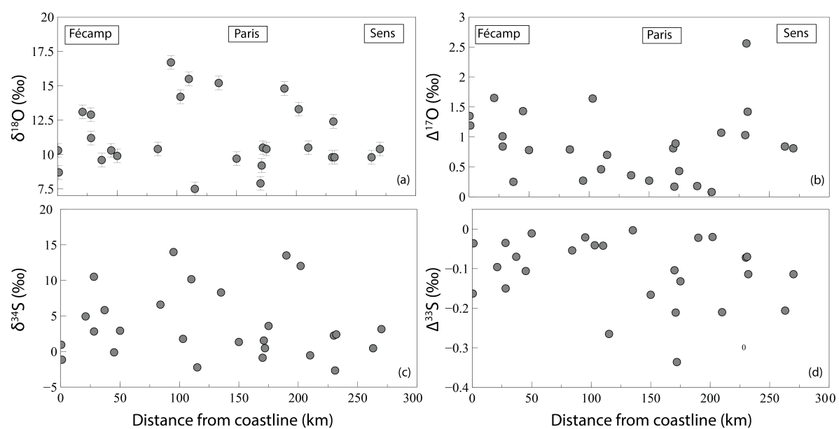
Fig. 1 supplementary Evolution of (a) \delta^{18}\text{O} , (b) \Delta^{17}\text{O} and (c) \delta^{34}\text{S} in function of the distance from coastline. No correlation between oxygen and sulfur isotopic compositions and the distance from the coastline are observed.
