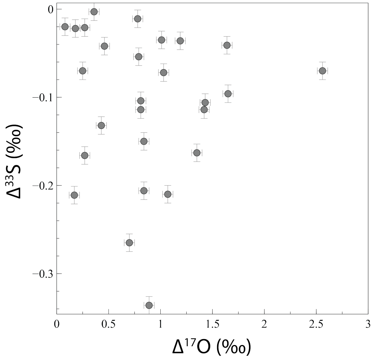
Fig. 2 supplementary Evolution of \Delta^{33}\text{S} with \Delta^{17}\text{O} -values.
