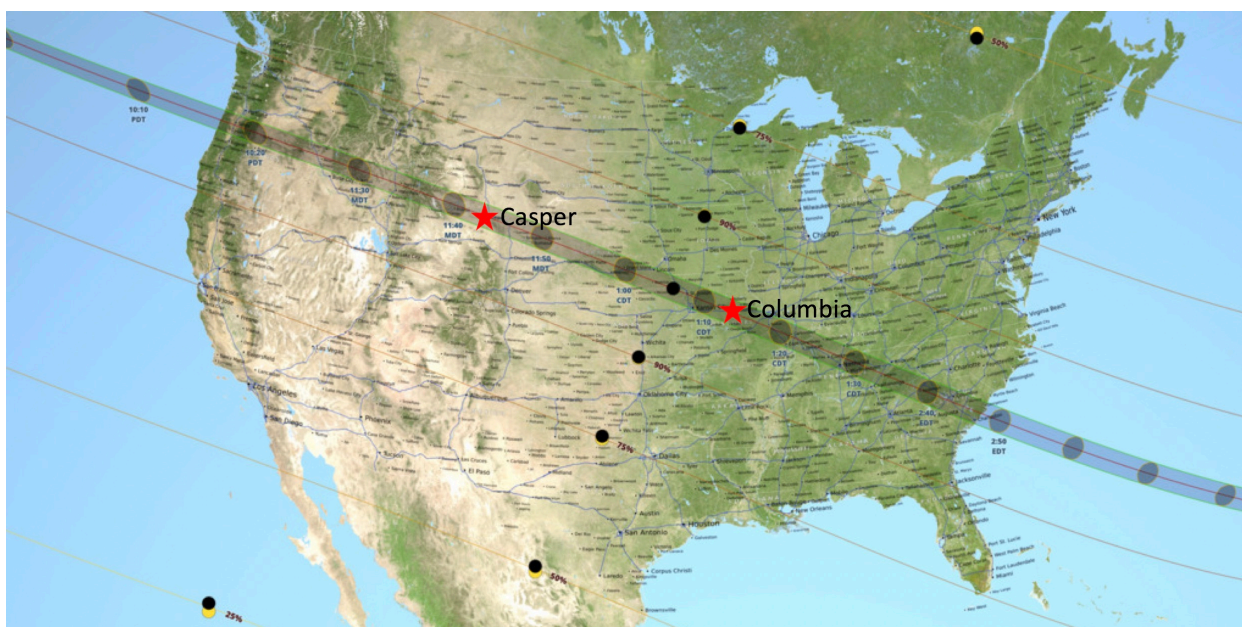
505 Figure 1: The eclipse map (from https://eclipse2017.nasa.gov ) shows the totality path and obscuration levels on 21 August 2017. Radiometers were deployed to make ground-based observations at Casper, Wyoming and Columbia, Missouri.
