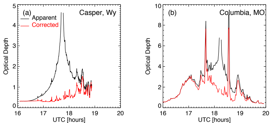
Figure 2: Apparent (black lines) and corrected (red lines) total optical depths that correspond to radiances observed by Pandora systems at (a) Casper and (b) Columbia during solar eclipse on August 21, 2017.
