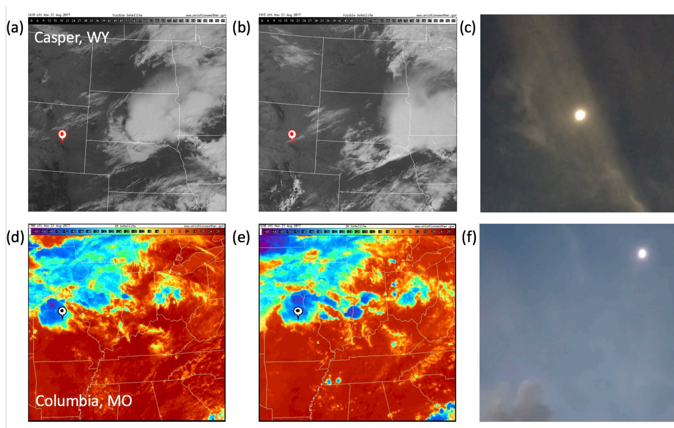
510 Figure 3: Top panel for Casper: (a) and (b) are geostationary satellite (GOES-16) visible images at 16:10 UTC and 19:15 UTC, showing thin cirrus clouds over the Casper site indicated by the mark; (c) photo taken near the totality. Lower panel for Columbia: (d) and (e) are the thermal infrared images 17:00 UTC and 18:30 UTC, showing high level clouds over Columbia site indicated by
