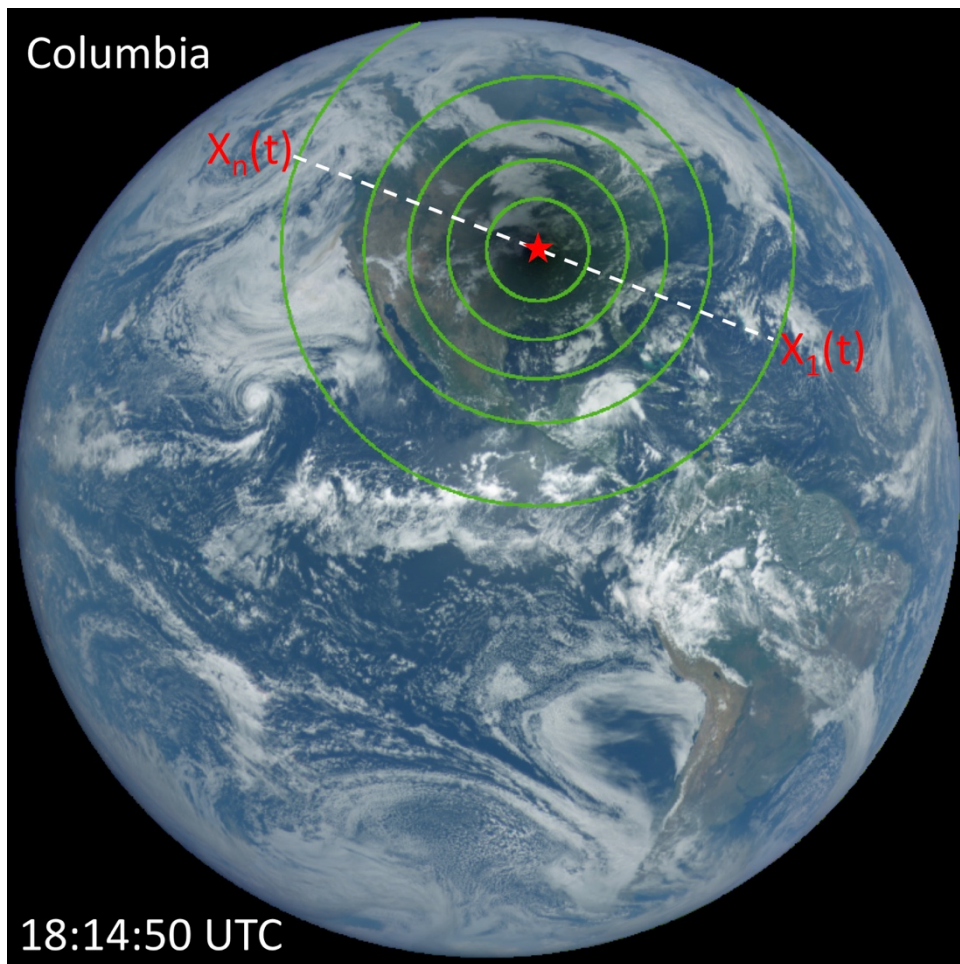
535 Figure 6: A sketch illustrating the conversion from temporal to spatial average. The color image has been adjusted from the images on https://epic.gsfc.nasa.gov by increasing the gamma correction (Cescatti, 2007) to bring out the region of totality over Columbia (red star) and surrounding clouds. The green contours show the levels of obscuration from 0% for the outermost circle with decrement of 20% inward. The dashed line illustrates the totality path.
