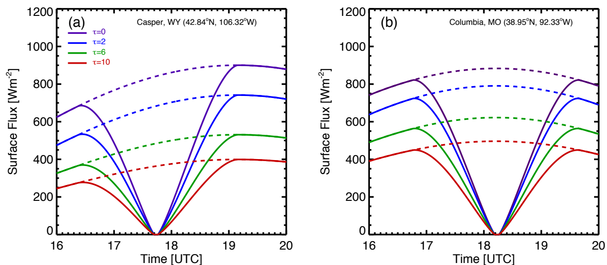
Figure 8: (a) Casper, (b) Columbia. The modelled surface SW flux variations for eclipse (solid lines) and non-eclipse conditions for different cloud optical depth.
