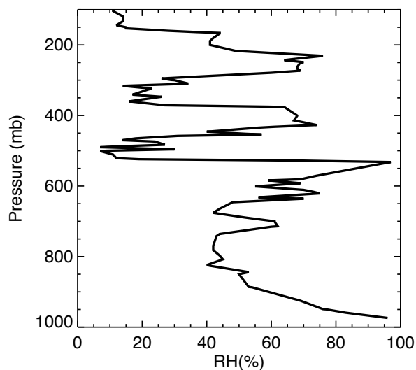
Figure 4: Radiosonde observed vertical profile of relative humidity from nearest station in Springfield, MO (at 37°14' N, 93°24' W) at 12 UTC on 21 August 2017 obtained from http://weather.uwyo.edu/upperair/sounding.html .
