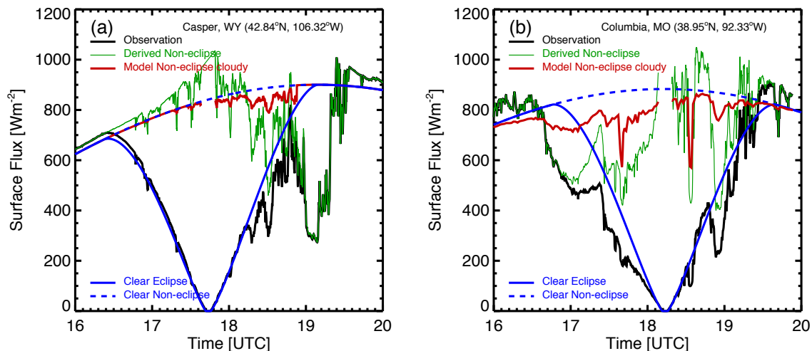
Figure 7: (a) Casper, (b) Columbia. Observed surface flux (black), derived surface SW flux for non-eclipse conditions (green), surface flux for clear atmospheric condition for eclipse (solid blue) and non-eclipse conditions (dashed blue), the modelled surface flux (red) uses observed cloud optical depth assuming 100% cloud coverage. For Casper site, the average reduction in local SW flux is 379\text{W/m}^2 or 50% and average reduction in global surface SW flux is 8%. For Columbia site, the average reduction in local surface SW flux is 329\text{W/m}^2 or 46% and average reduction in global surface SW flux is 7%.
