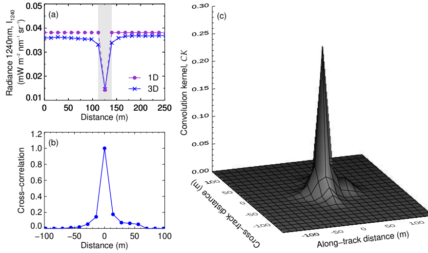
Figure A1. (a) Comparison of the nadir reflected radiance at 1240 nm by a stratiform cloud deck simulated with 1D and 3D radiative transfer simulations. The cloud contains a 15 m region of pure ice (shaded) embedded between two pure liquid water regions (non-shaded). (b) Cross-correlation between the 1D and the 3D cloud top radiance illustrating the extent of the horizontal photon transport. (c) Normalized convolution kernel based on the cross-correlation of the 1D and 3D simulations and different sun-sensor geometries.
