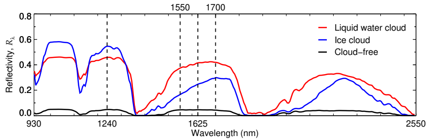
Figure 1. Reflectivity spectra of a pure liquid water cloud and a pure ice cloud of optical thickness 12 compared with a clear sky spectrum in the wavelength range measured by AISA Hawk. The vertical dashed lines indicate the wavelengths needed to calculate the slope phase index (1550 - 1700 nm), and to retrieve the cloud optical thickness (1240 nm) and effective radius (1625 nm)
