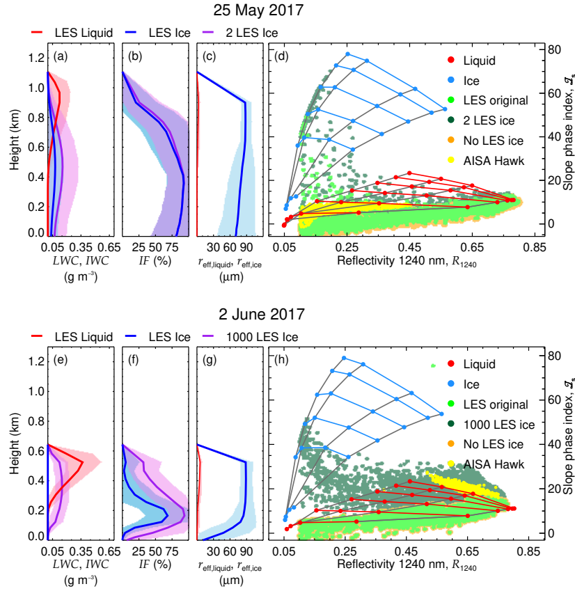
Figure 9. Mean profiles of liquid and ice water content, ice fraction and effective radius ( a , b , and c for 25 May 2017 and e , f , and g for 2 June 2017, respectively). The shaded areas indicate the standard deviation of the considered distribution. The simulated R_{1240} and \mathcal{I}_s corresponding to the original LES profiles, as well as simulations neglecting the IWC (‘No LES ice’) and modifying it (‘2 LES ice’ for 25 May and ‘1000 LES ice’ for 2 June), are compared with R_{1240} and \mathcal{I}_s of pure phase clouds and the AISA Hawk measurements in ( d ) (25 May) and ( h ) (2 June).
