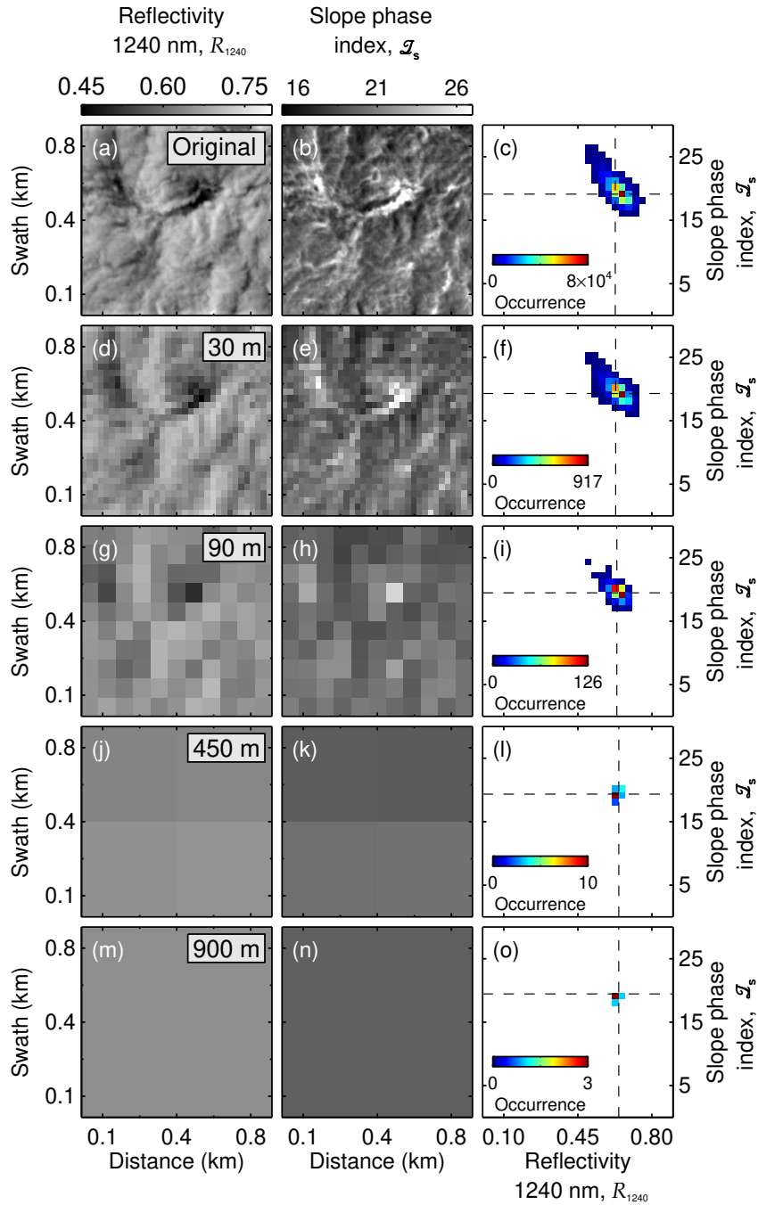
Figure 11. Slope phase index - 1240 nm reflectivity relationship for 5 different pixel sizes (original AISA Hawk resolution, 30 m, 90 m, 450 m, and 900 m). (a), (d), and (g) show a 1 \text{ km} \times 1 \text{ km} subsection of R_{1240} measured on 2 June 2017 as seen by the five different resolutions; (b), (e) and (h), the corresponding 1 \text{ km} \times 1 \text{ km} \mathcal{I}_s ; and (c), (f) and (i) present the scatter between both magnitudes for the complete 1 \text{ km} \times 4 \text{ km} field. The dashed lines indicate the 25th percentile of R_{1240} and \mathcal{I}_s for each resolution.
