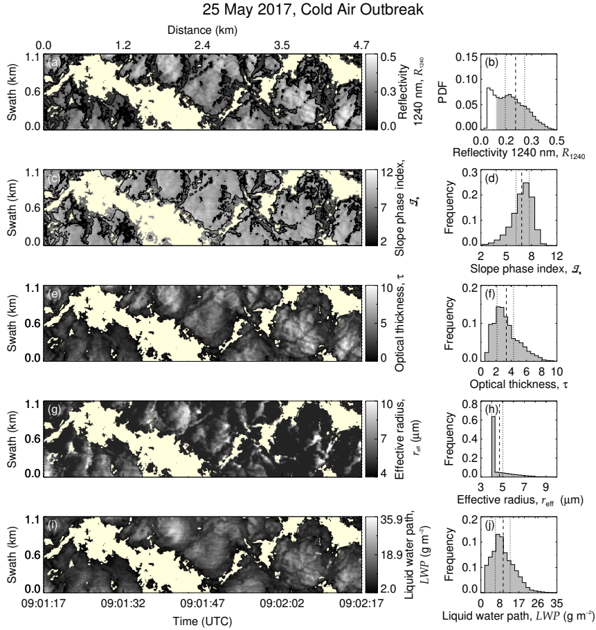
Figure 4. AISA Hawk measurement on 25 May 2017. Cloud top reflectivity (a), slope phase index (c), retrieved optical thickness (e), retrieved effective radius (g) and liquid water path (i). The overlaid contours in (a) and (c) separate the cloud central regions from the cloud edges. The frequency of occurrence histograms are displayed on the corresponding right-hand figures (b, d, f, h, j). Data classified as cloud free is shown by the non-colored histogram in (b). Dashed lines indicates the mean value of each field and the dotted lines show the corresponding 25th and 75th percentile.
