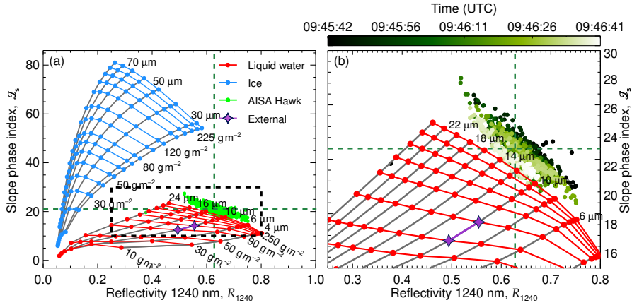
Figure 7. (a) \mathcal{I}_s measured on 2 June 2017 presented as a function of R_{1240} (green dots). The dashed lines indicate the 25th percentile of R_{1240} and the 75th percentile of \mathcal{I}_s . The two grids represent radiative transfer simulations for a range of pure liquid (red) and pure ice (blue) clouds. The liquid water clouds cover droplets with r_{\text{eff}} between 4 and 24 \mu\text{m} and LWP between 1 and 250 \text{g m}^{-2} . The ice clouds are simulated for columnar ice crystals with r_{\text{eff}} between 28 and 90 \mu\text{m} and IWP between 1 and 250 \text{g m}^{-2} . A SZA of 57.9° was considered. The purple stars shows the independent LWP range retrieved by the 89 GHz passive channel of MiRAC and the SID-3 in situ observation of particle size. (b) Zoom into the area highlighted by a dashed rectangle in (a). Color-coded is the acquisition time of measurements illustrating changes along the flight path.
