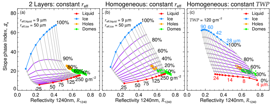
Figure 8. Comparison of \mathcal{I}_s measured on 2 June 2017 as a function of R_{1240} with three mixing scenarios of mixed-phase clouds. Observations in cloud holes are indicated by orange dots. Green dots represent measurements in cloud domes. Scenario (a) simulates a two layer cloud, while in scenarios (b) and (c) a homogeneously mixed cloud is assumed. Scenario (b) considers mixed-phase clouds of fixed particle sizes ( r_{\text{eff,liquid}} of 9 \mu\text{m} and r_{\text{eff,ice}} of 50 \mu\text{m} ) and variable TWP between 25 and 250 \text{ g m}^{-2} . The grey solid lines connect clouds of equal TWP and the solid purple lines, clouds of equal IF (indicated by the percentages). In scenario (c) TWP is fixed to 120 \text{ g m}^{-2} and the particle sizes are varied. Here, purple lines connect clouds of equal ice fraction and the grey lines connect clouds considering equal particle sizes.
