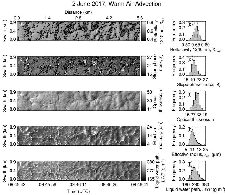
Figure 6. AISA Hawk measurement on 2 June 2017. Cloud top reflectivity (a), slope phase index (c), retrieved optical thickness (e), retrieved effective radius (g) and liquid water path (i). The overlaid contours in (a) and (c) separate the cloud central regions from the cloud edges. The frequency of occurrence histograms are displayed on the corresponding right-hand figures (b, d, f, h, j). The dashed line indicates the mean value and the dotted lines show its 25th and 75th percentile.
