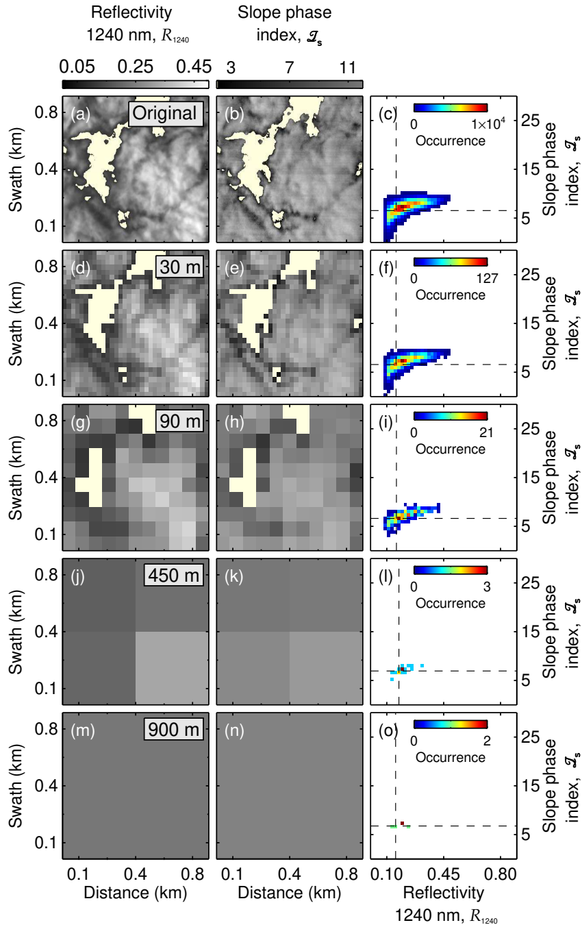
Figure 10. Slope phase index - 1240 nm reflectivity relationship for 5 different pixel sizes (original AISA Hawk resolution, 30 m, 90 m, 450 m, and 900 m). (a), (d), and (g) show a 1 \text{ km} \times 1 \text{ km} subsection of R_{1240} measured on 25 May 2017 as seen by the five different resolutions; (b), (e), and (h), the corresponding 1 \text{ km} \times 1 \text{ km} \mathcal{I}_s ; and (c), (f) and (i) present the scatter between both magnitudes for the complete 1 \text{ km} \times 4 \text{ km} field. The dashed lines indicate the 25th percentile of R_{1240} and \mathcal{I}_s for each resolution.
