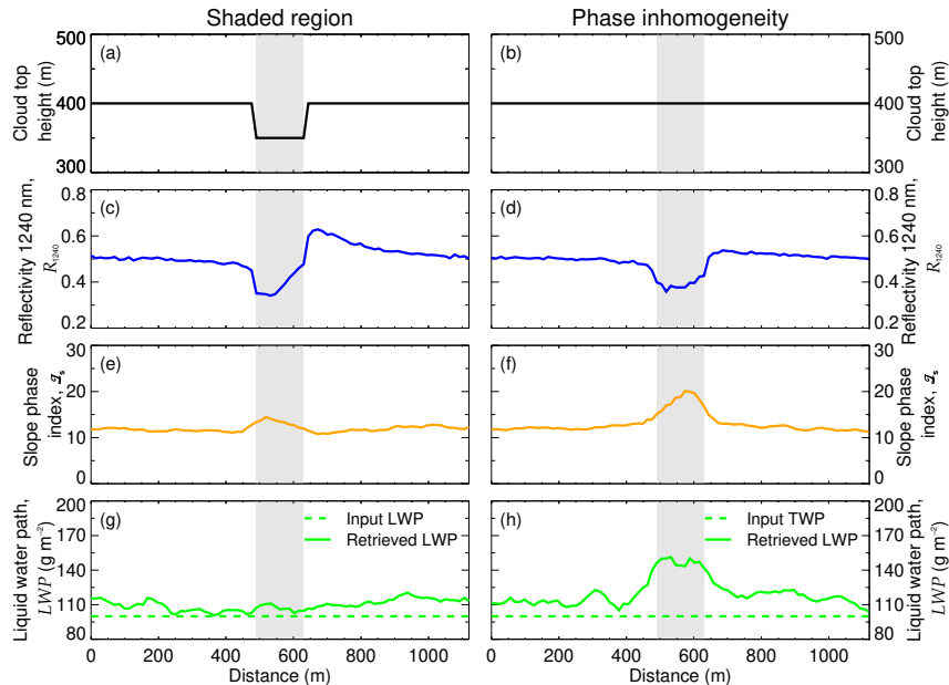
Figure A2. Cloud top properties of a shaded region (a, c, e, g) compared to a region with a different thermodynamic phase composition (b, d, f, h). The shaded areas indicates the artifact affected areas
