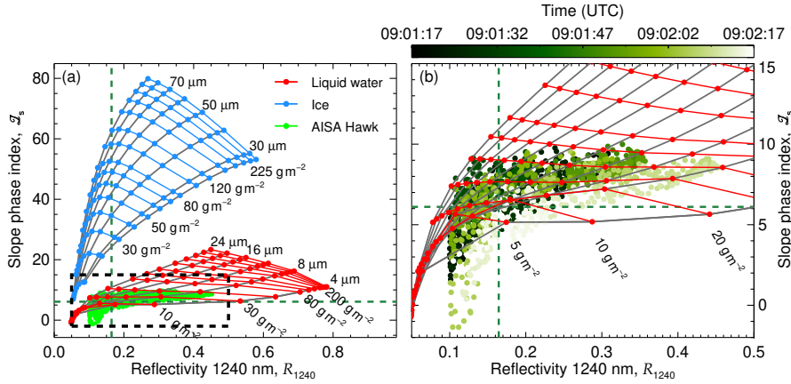
Figure 5. (a) \mathcal{I}_s measured on 25 May 2017 presented as a function of R_{1240} (green dots). The dashed lines indicate the 25th percentile of R_{1240} and \mathcal{I}_s . The two grids represent radiative transfer simulations for a range of pure liquid (red) and pure ice (blue) clouds. The liquid water clouds cover droplets with r_{\text{eff}} between 4 and 24 \mu\text{m} and LWP between 1 and 250 \text{g m}^{-2} . The ice clouds are simulated for columnar ice crystals with r_{\text{eff}} between 28 and 90 \mu\text{m} and IWP between 1 and 250 \text{g m}^{-2} . A \text{SZA} of 60.5° was considered. (b) Zoom of the area highlighted by a dashed rectangle in (a). Color-coded is the acquisition time of the measurements illustrating changes along the flight path.
