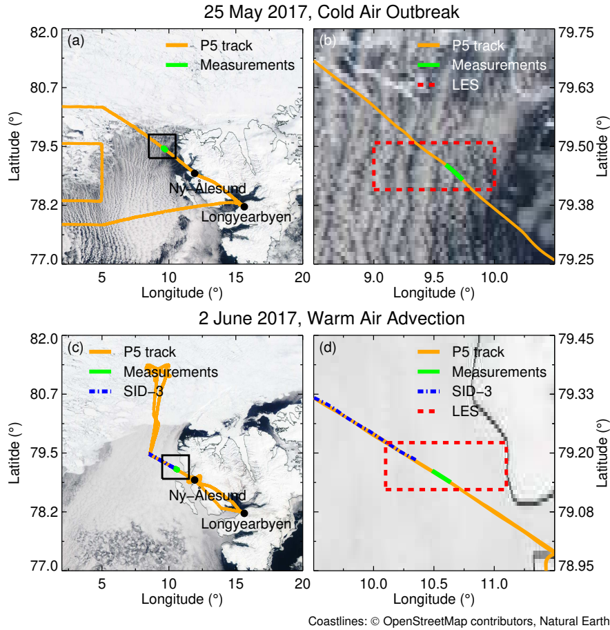
Figure 2. MODIS true color images from the NASA Worldview application ( https://worldview.earthdata.nasa.gov ) on 25 May 2017 (a) during a cold air outbreak and on 2 June 2017 (c) during a warm air advection. Zooms into the regions delimited by black squares are shown in (b) and (d). The measurements location (79.5° N, 9.5° E on 25 May and 79.2° N, 10.7° E on 2 June) is indicated by the green section of the flight track of Polar 5 (orange). The areas extracted from the LES are indicated by the dashed red rectangle. The dashed-dotted blue on 2 June line indicates the location of the SID-3 measurements.
