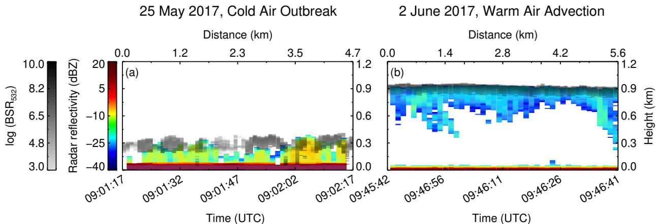
Figure 3. Combination of MiRAC radar reflectivity (color range between blue and red) and AMALi backscatter ratio (colors between white and black) as measured on 25 May 2017 during a cold air outbreak (a) and on 2 June 2017 during a warm air advection (b). AMALi’s lidar backscatter ratio is highly sensitive to the liquid droplets and shows the liquid top layer in both clouds. MiRAC’s radar reflectivity is dominated by larger particles and indicate regions with ice crystals. The radar signal below an altitude of 150 m is heavily influenced by ground clutter and cannot interpreted for cloud studies.
