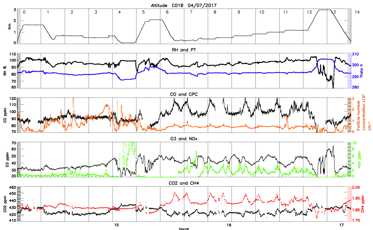
Figure 6: As in Fig. 4 but for the third flight (C018; 4 th July, afternoon).
