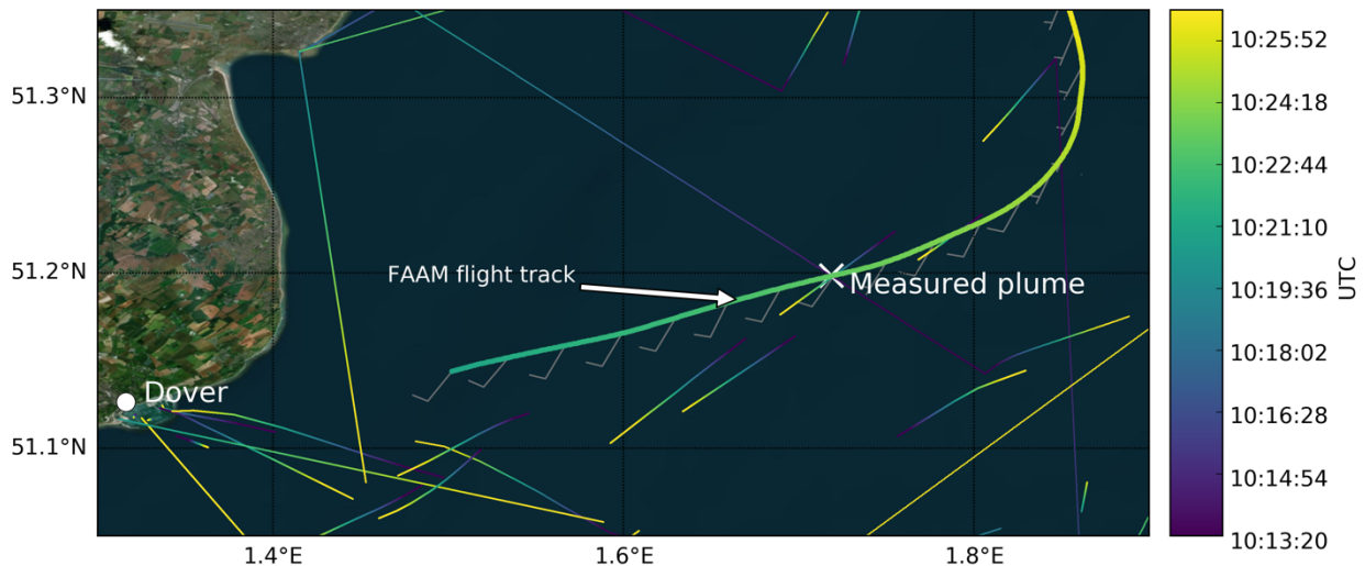
Figure 9: Flight track of FAAM BAe-146 (thick coloured line) during flight C017 at the beginning of the level run at ~40 m a.m.s.l where a large ship plume was measured (indicated with a white cross). Wind speed and direction measured by FAAM BAe-146 are shown by the wind barbs. The trajectories of all the ships >10 kton are shown by thin coloured lines with the colour scale denoting time. The base map was created using the World Imagery maps in ArcGIS® software by Esri. ArcGIS® and ArcMap™ are the intellectual property of Esri and are used herein under license. Copyright © Esri. All rights reserved. For more information about Esri® software, please visit www.esri.com .
