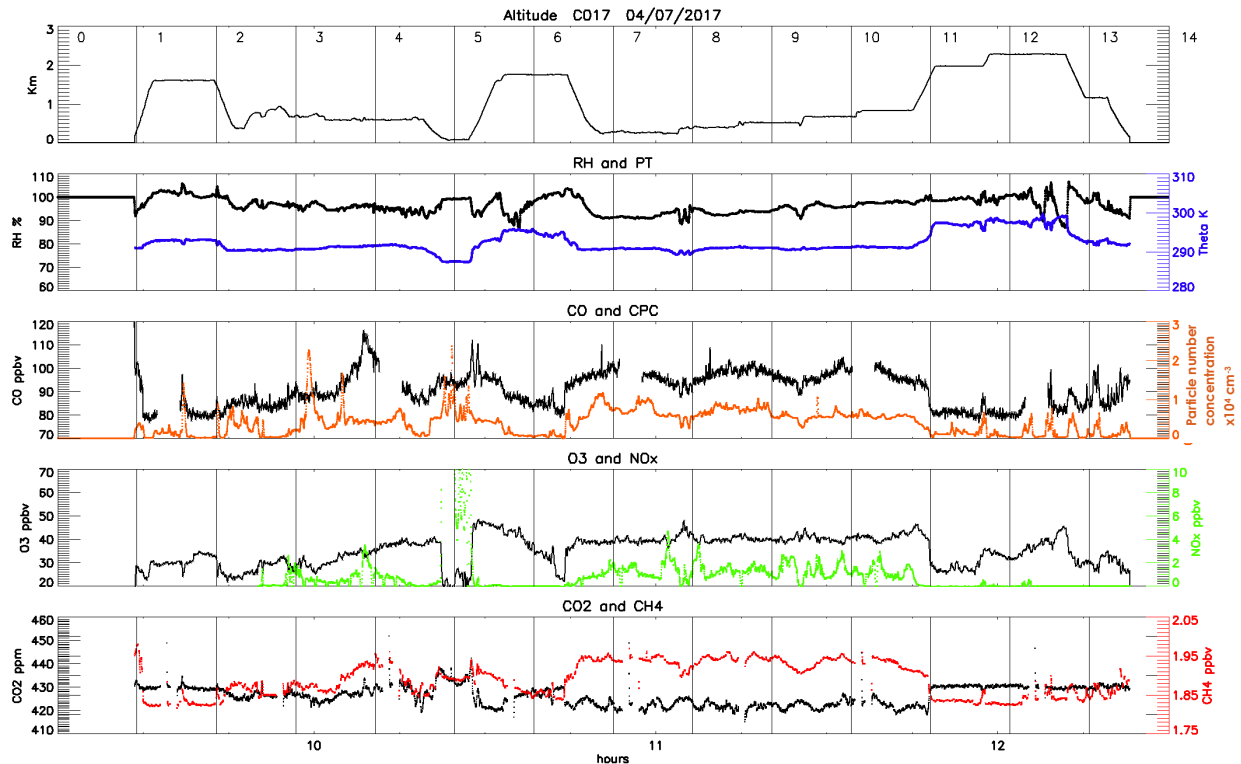
Figure 5: As in Fig. 4 but for the second flight (C017; 4th July, morning).
