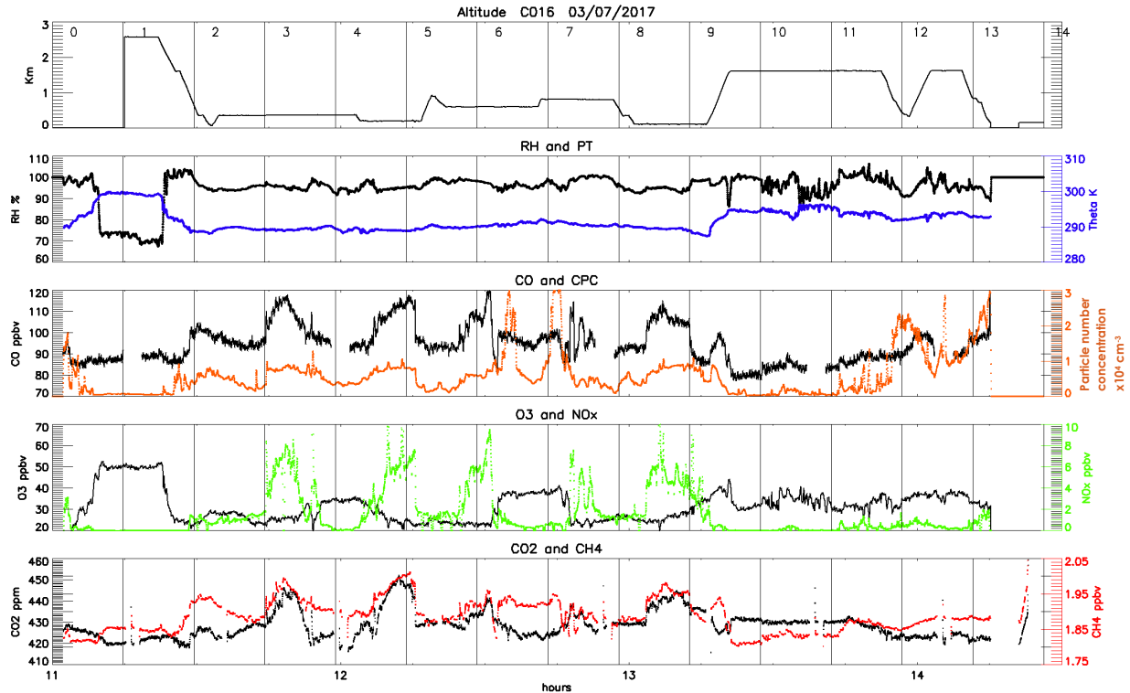
Figure 4: Time series of the main observations during the first flight (3 rd July, late morning) showing: the altitude of the aircraft (top panel), relative humidity (second panel, black) and potential temperature (blue), CO concentration (third panel, black) and particle number concentration (orange), O 3 (fourth panel, black) and NO x (green) concentrations, CO 2 (fifth panel, black) and CH 4 (red) concentrations. The numbered vertical lines correspond to the numbers along the flight path shown in Fig. 1.
