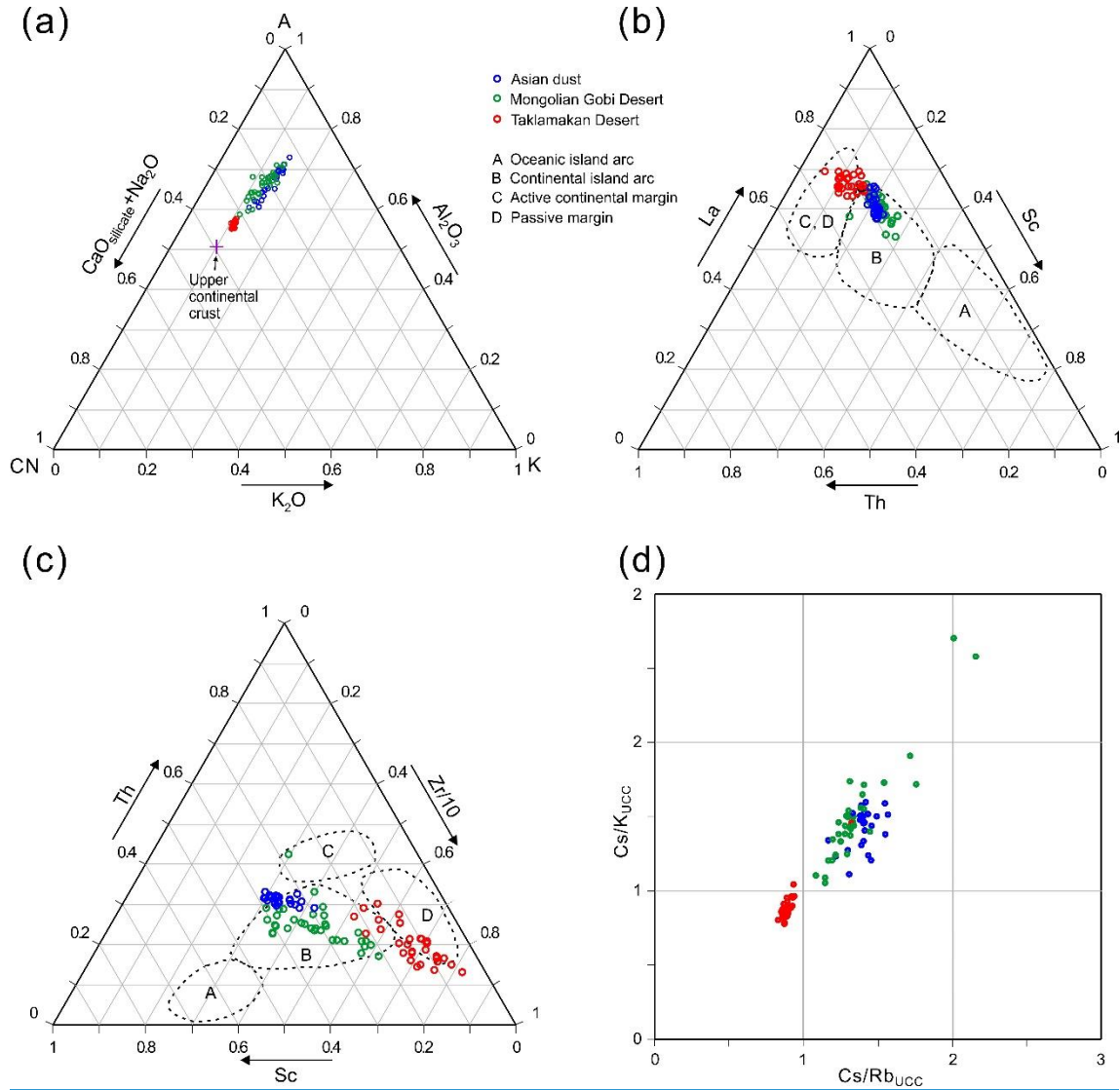
Figure 11. Plots of trace and major element compositions for discriminating the source of Asian dust. (a) A–CN–K diagram showing the molecular proportions of \text{Al}_2\text{O}_3 , \text{K}_2\text{O} , and \text{CaO}_{\text{silicate}} + \text{Na}_2\text{O} . Value of \text{Al}_2\text{O}_3 is equivalent to CIA. \text{CaO}_{\text{silicate}} was obtained by the correction of carbonate CaO (Honda and Shimizu, 1998). (b) La–Th–Sc plot. (c) Th–Sc–Zr/10 plot. (d) \text{Cs}/\text{K}_{\text{UCC}} – \text{Cs}/\text{Rb}_{\text{UCC}} plot. Data were normalized to UCC. Data of Asian dust and Mongolian Gobi Desert soils ( < 20 \mu\text{m} ) from this study. Trace element data for Taklamakan Desert soils from Jiang and Yang (2019) ( < 63 \mu\text{m} ). Major element data for Taklamakan Desert soils from Honda and Shimizu (1998) ( < 45 \mu\text{m} ) and Jiang and Yang (2019) ( < 63 \mu\text{m} ).
