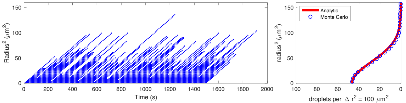
Figure 1. (Left) Radius squared versus time for 150 droplets growing by condensation in 100.1% supersaturation with probability of fallout per unit time of u/h = k_1 r^2/h u/h = k_1 r^2/h for h = 1 m. (Right) Frequency distributions of the radius squared from the Monte Carlo model (for 6000 1.5 \times 10^6 droplets) and from the analytic solution (20) for the same parameters.
