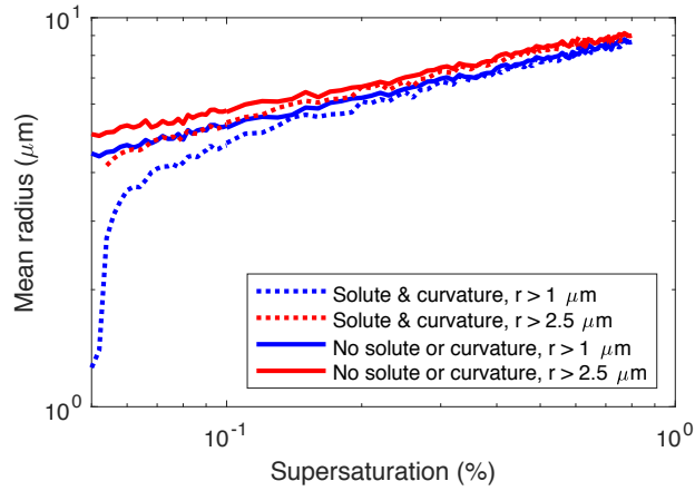
Figure 8. Average over the 11 DSDs of the coefficient of variation of the nominal mean Mean droplet radius versus supersaturation values implied by from the three measured moments versus the truncation radius Monte Carlo model: with solute and droplet curvature effects (dotted lines) and without (solid lines) for all droplets (blue) and excluding droplets with radii < 2.5 \mu\text{m} .
