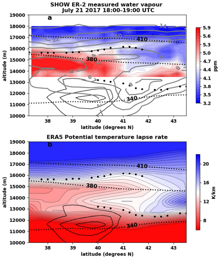
205 Figure 6: SHOW measured water vapour profile (from 18:00 UTC to 19:00 UTC) (a) and the potential temperature lapse rate determined from the ERA5 reanalysis for the 19:00 UTC time step along the SHOW measurement track (b). The dark dotted line shows the location of the thermal tropopause. The grey contours show the potential vorticity, several zonal wind contours are shown in black, and the light black dotted line shows the 340 K, 380 K and 410 K isentropes respectively. The longitude is along the 124.5° W line and is nearly constant for the measurements.
