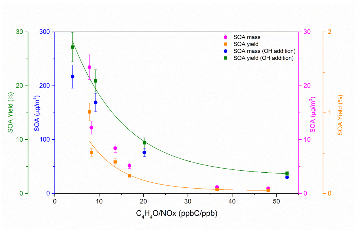
Figure 3: Dependence of the SOA mass concentration and SOA yield on the C_4H_4O/NO_x ratio. Since the particle wall loss has a weak RH dependence in our chamber, a mean value of 3.6 \times 10^{-5} s^{-1} was used for wall loss correction. A density of 1.4 g cm^{-3} was used in SMPS (Jia and Xu, 2018; Kostenidou et al., 2007).
