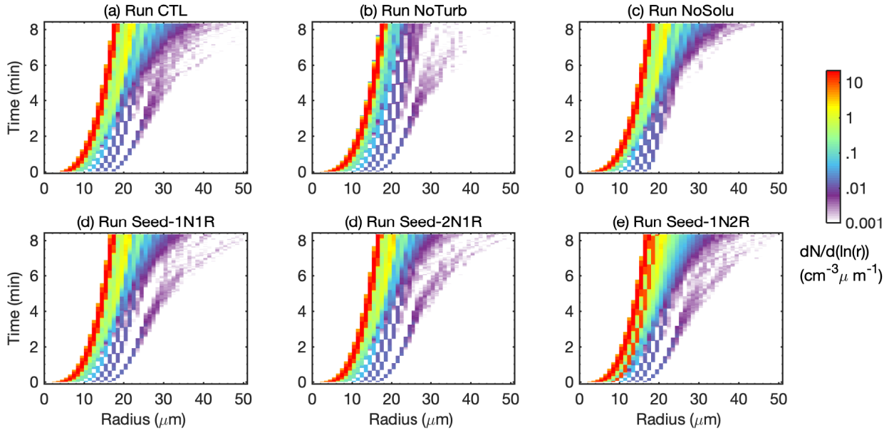
Figure 3. Time evolution of the droplet size distribution in the condensation-collision set of experiments. The droplet number concentration ( cm^{-3} ) is indicated by colors with its value shown in the color bar. The configuration of each experiment is listed in Table 2.
