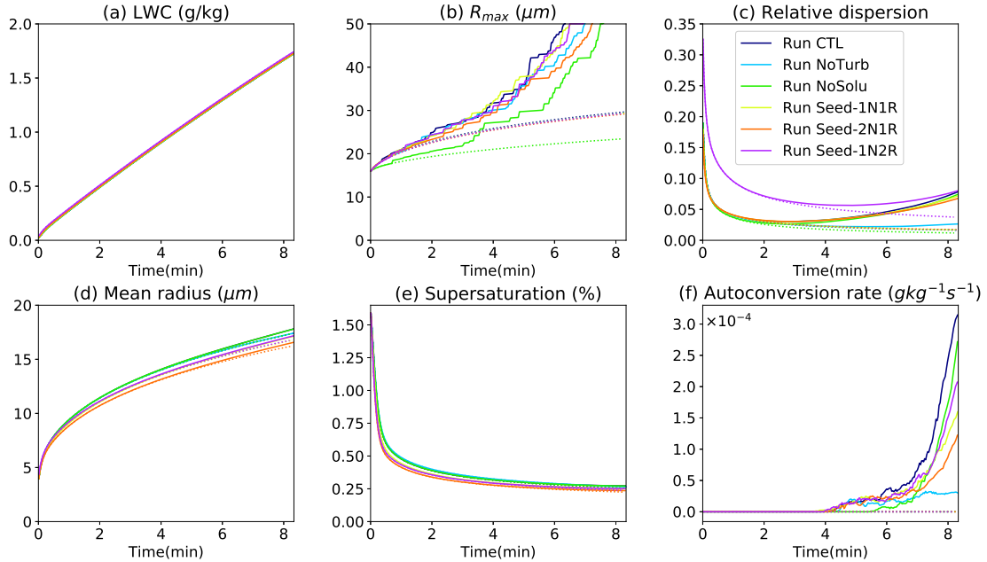
Figure 7. The temporal variation of bulk (a) liquid water content (LWC), (b) maximum droplet radius ( R_{max} ), (c) relative dispersion, (d) droplet mean radius, (e) supersaturation ratio, and (f) autoconversion rate in the condensation-collision set of experiments (solid lines) and in the condensation-only set of experiments (dotted lines). The relative dispersion is defined as the standard deviation of the droplet radius divided by the mean radius. The autoconversion rate here is defined as the mass transfer rate from droplets smaller than R = 30 \mu m to droplets larger than 30 \mu m . The droplets over 50 \mu m are treated as fall-outs and removed from the domain. Thus (b) only shows a maximum droplet size at 50 \mu m .
