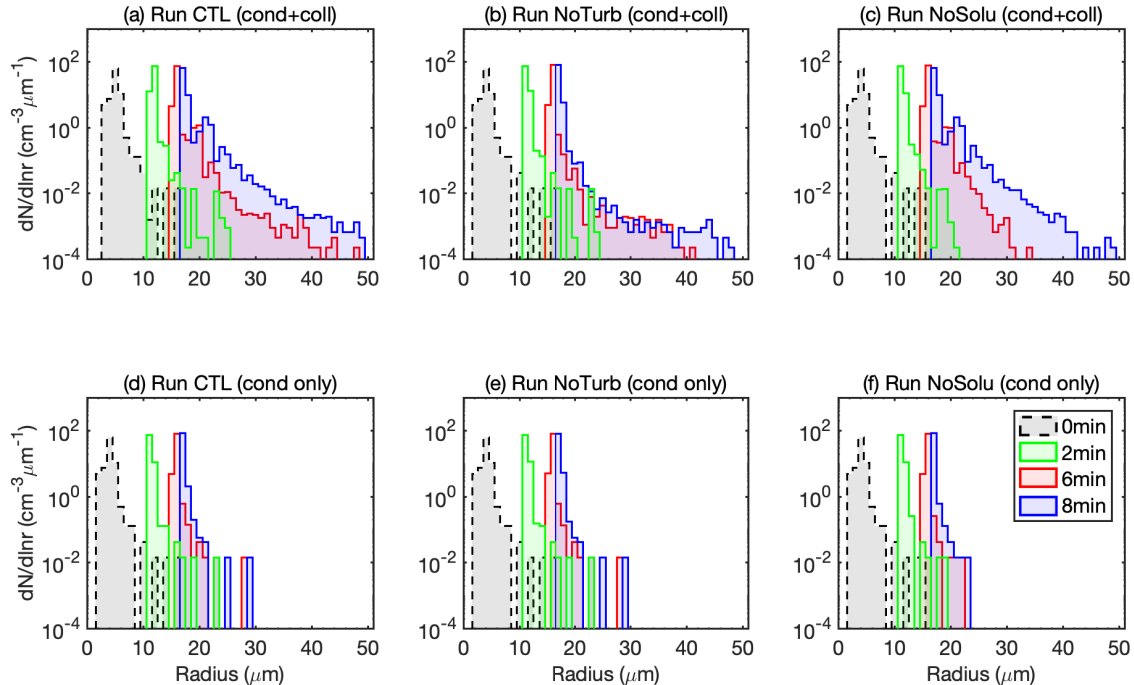
Figure 4. Droplet size distributions (DSDs) at T = 0 \text{ min} (grey), T = 2 \text{ min} (green), T = 6 \text{ min} (red), and T = 8 \text{ min} (blue) of the natural cases (Runs CTL, NoTurb, and NoSolu). The upper panel (a-c) is the DSD in the condensation-collision set of experiments, and the lower panel (d-e) is the DSD in the condensation-only set of experiments.
