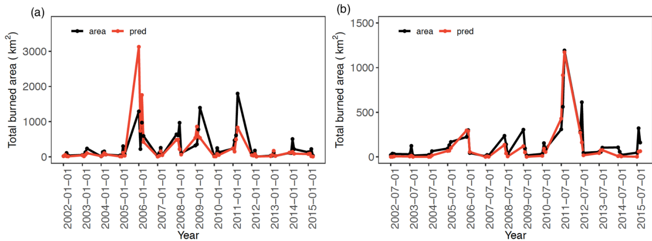
975 Figure 5. Timeseries of observed (black line) and predicted total burned area (red line) over South Central US for the (a) winter-spring and (b) summer fire season.
