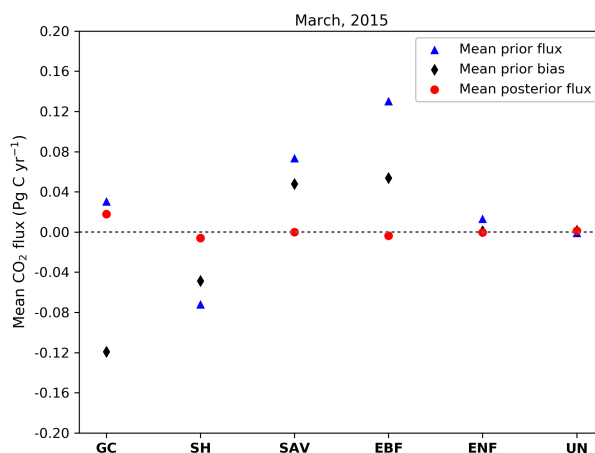
Figure 11. Prior (blue) and posterior (red) monthly mean CO 2 flux of a ensemble of five realizations and monthly mean prior bias (black) added to the true prior fluxes (dashed grey line). Note: results are shown for adding the same biases to our five realizations.
