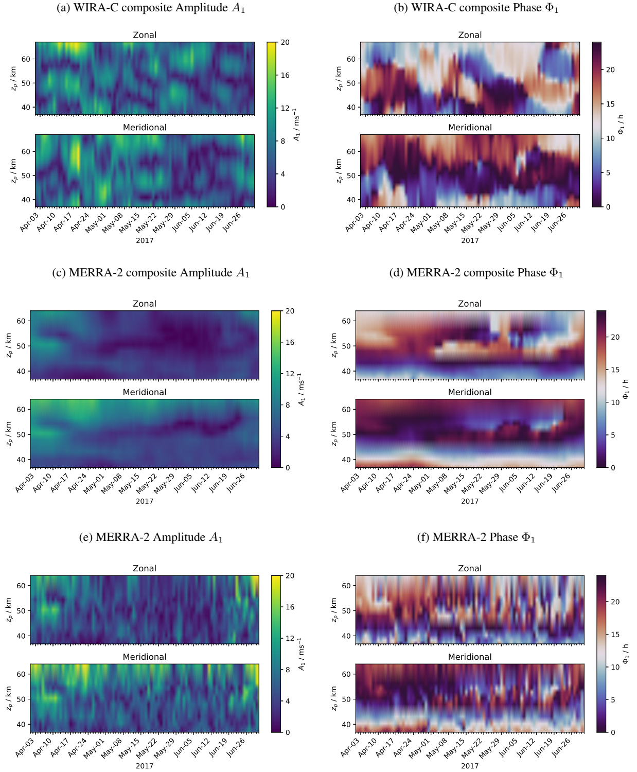
Figure 4. Amplitude and phase of the diurnal tide over three months from WIRA-C measurements (a,b), smoothed MERRA-2 reanalysis (c,d), and original MERRA-2 (e,f) during the tropical campaign at the Maïdo observatory.
