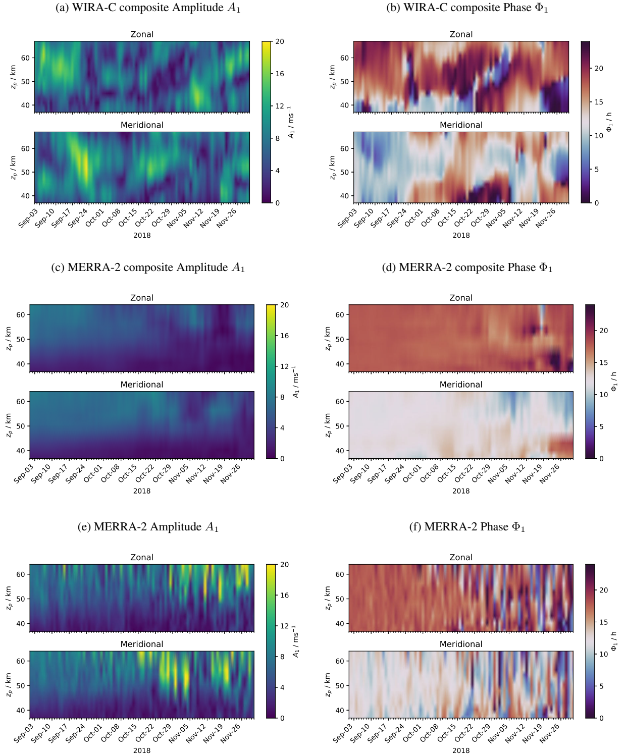
Figure 10. Amplitude and phase of the diurnal tide over three months from WIRA-C measurements (a,b), smoothed MERRA-2 reanalysis (c,d), and original MERRA-2 (e,f) during the arctic campaign at the 25 OMAR observatory.
