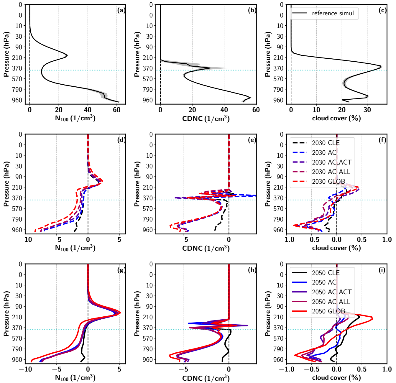
Figure 5. Arctic vertical profiles (top row) in 2010 and their respective changes in 2030 (middle row) and 2050 (bottom row) for N 100 (left), CDNC (center), and cloud cover fraction (right). The grey shading in panels a – c denotes the interval between the 10 th and 90 th percentile of the data.
