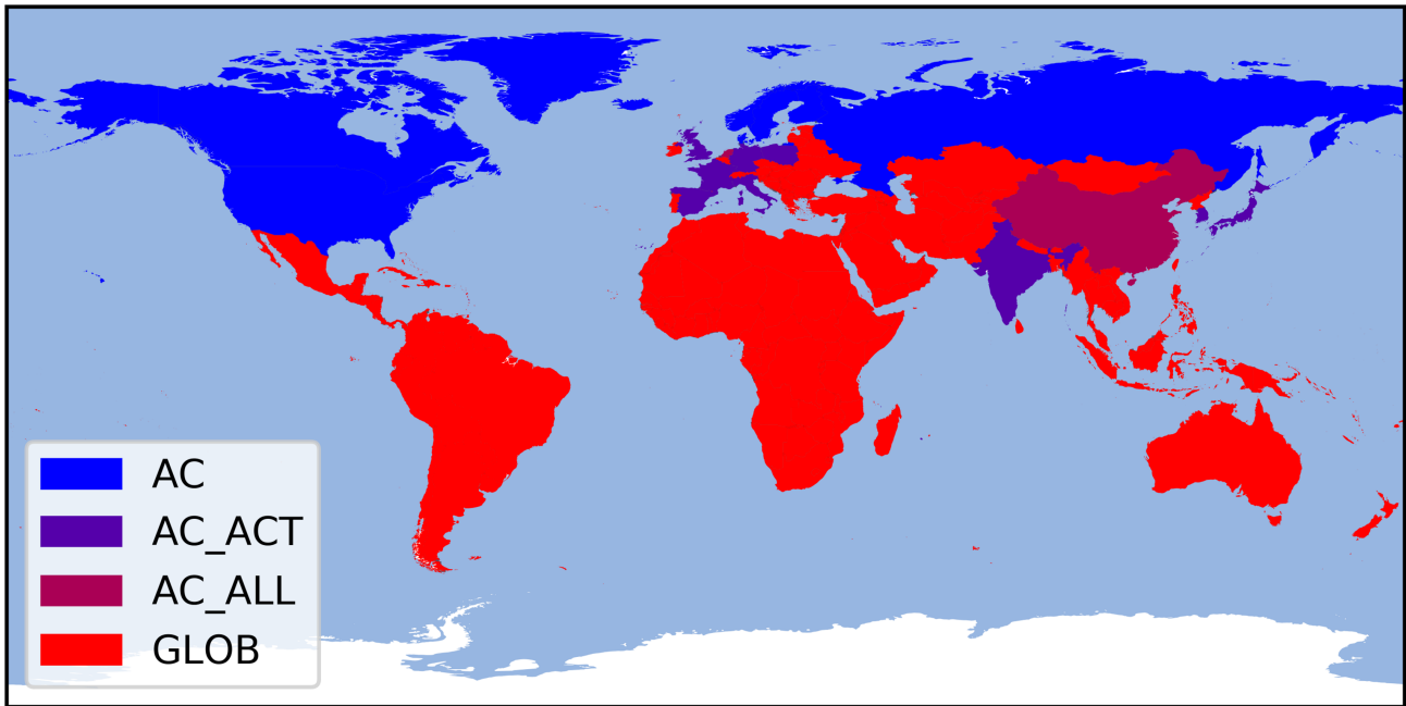
Figure 1. Global extend of SLCF reductions for the different scenarios. Starting from AC, each scenario includes all countries of the previous scenario (e.g. AC_ACT = AC plus active observer states).
