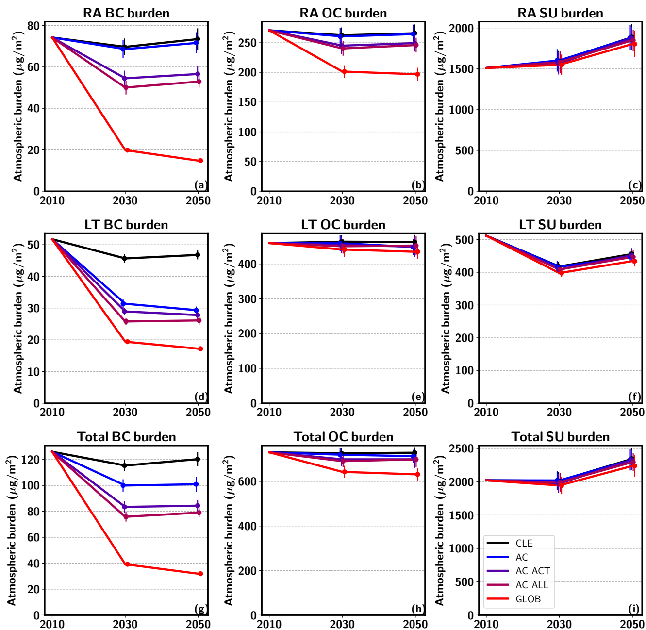
Figure 4. Arctic aerosol mass burdens for BC (left), OC (center), and SU (right). The top row shows the rest of the atmosphere (RA) burdens, middle row shows lower troposphere (LT) burdens, and bottom row shows the total column burden. The error bars show the standard deviation of the data.
