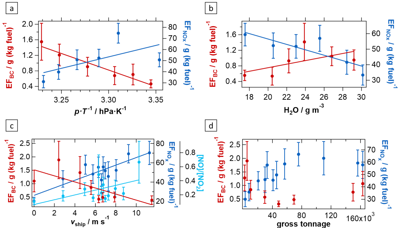
5 Figure 3: Influences of combustion conditions on ship emission plumes. The dependencies of the NO x and BC emission factors on the ratio between atmospheric pressure and ambient temperature (a) and on ambient water vapour concentration (b) are demonstrated. Additionally, the dependencies of the NO x and BC emission factors as well as of the NO to NO 2 ratio of average excess concentrations on the vessel speed are presented (c). The correlations between the NO x and BC emission factors and the vessel gross tonnage are shown (d). Error bars present the combination of estimated quantification and measurement uncertainties and one sigma standard deviations of the data distributions in each bin. The corresponding fit parameters and correlation coefficients are listed in Table 2. 10
