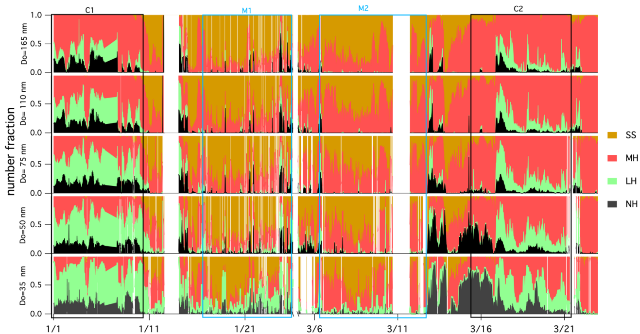
Figure 4. Time series of the number fraction of NH mode in black ( GF < 1.11 ), LH mode in green, ( 1.11 < GF < 1.33 ), MH mode in red ( 1.33 < GF < 1.85 ) and SS mode in brown ( GF > 1.85 ) of aerosols with pre-selected dry diameter.
