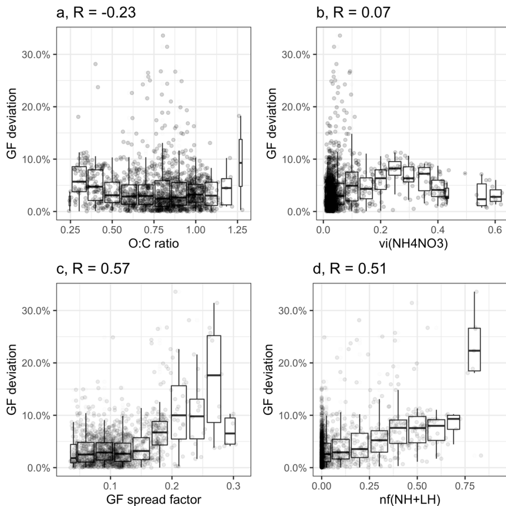
Figure 8. The relationship of GF deviation to (a) O:C ratio, (b) volume fraction of \text{NH}_4\text{NO}_3 , (c) GF spread factor and (d) n_f(\text{NH}+\text{LH}) over the whole period.
