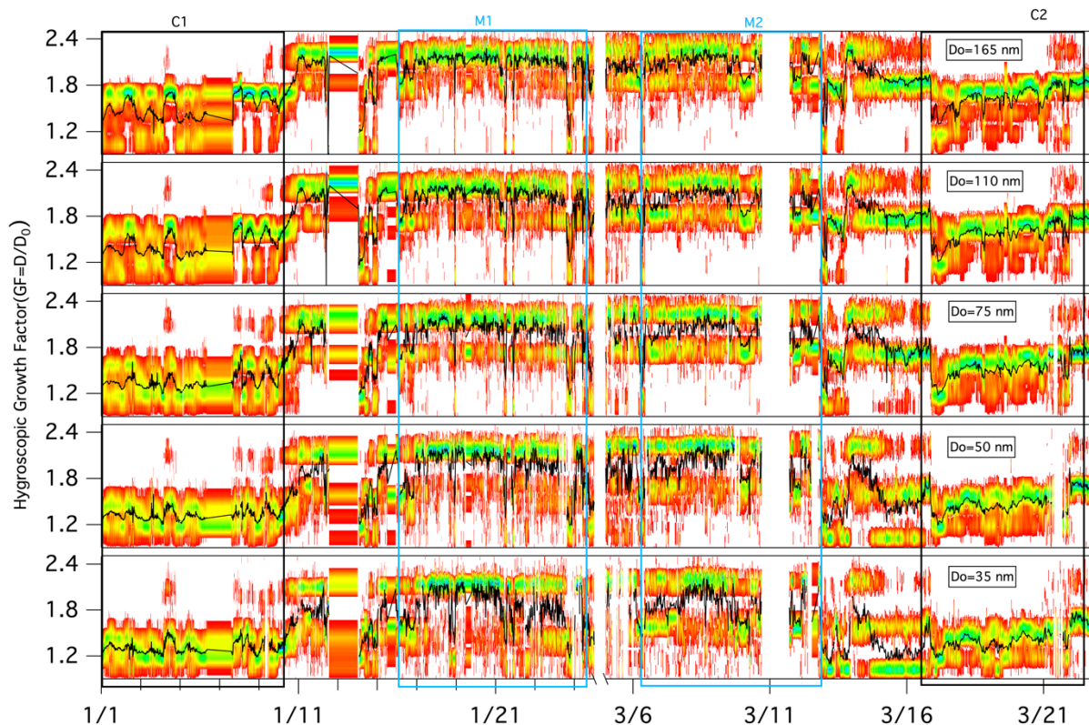
535 Figure 3. Growth factor probability distribution function (GF-PDF) for different particle dry sizes as measured by the HTDMA. The colour bar indicates the probability density and the black line represents the averaged GF.
