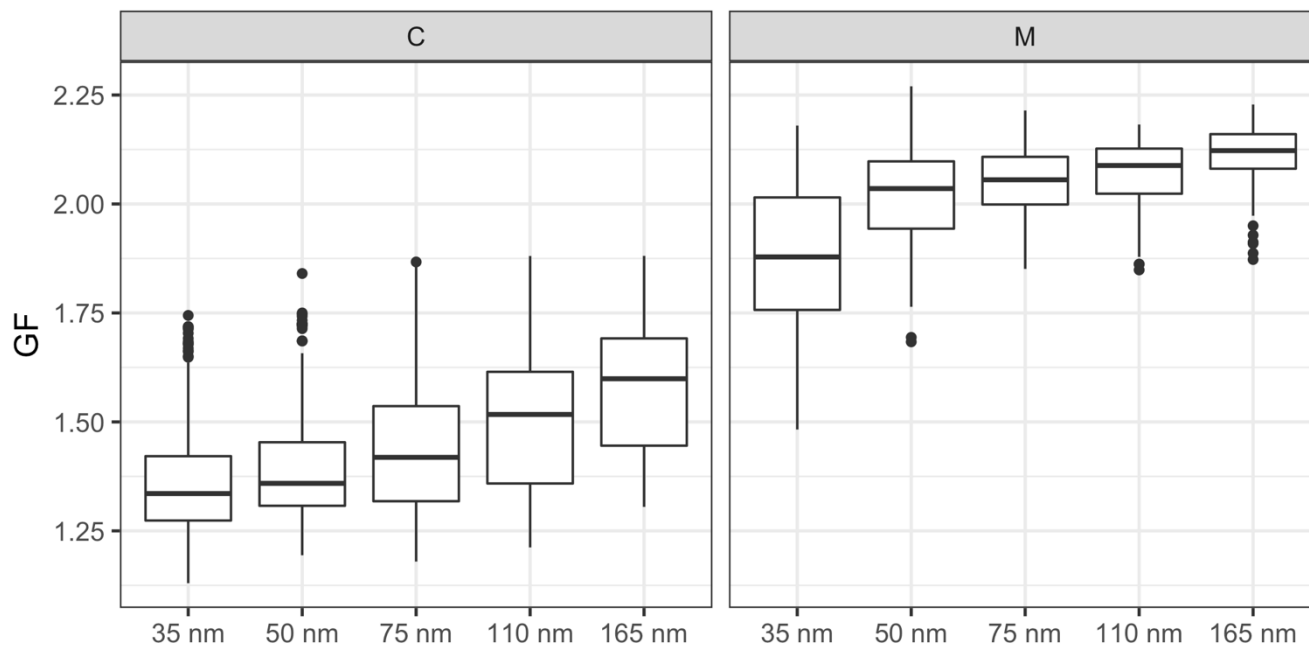
Figure 5. Size resolved GFs for (a) C1 & C2 and (b) M1 & M2. The horizontal lines represent median GF, the boxes represent 25-75 % percentile and whiskers represent 1.5 \times \text{IQR} from the boxes (where the IQR is the interquartile range). Data beyond the end of whisker are plotted individually as outliers.
