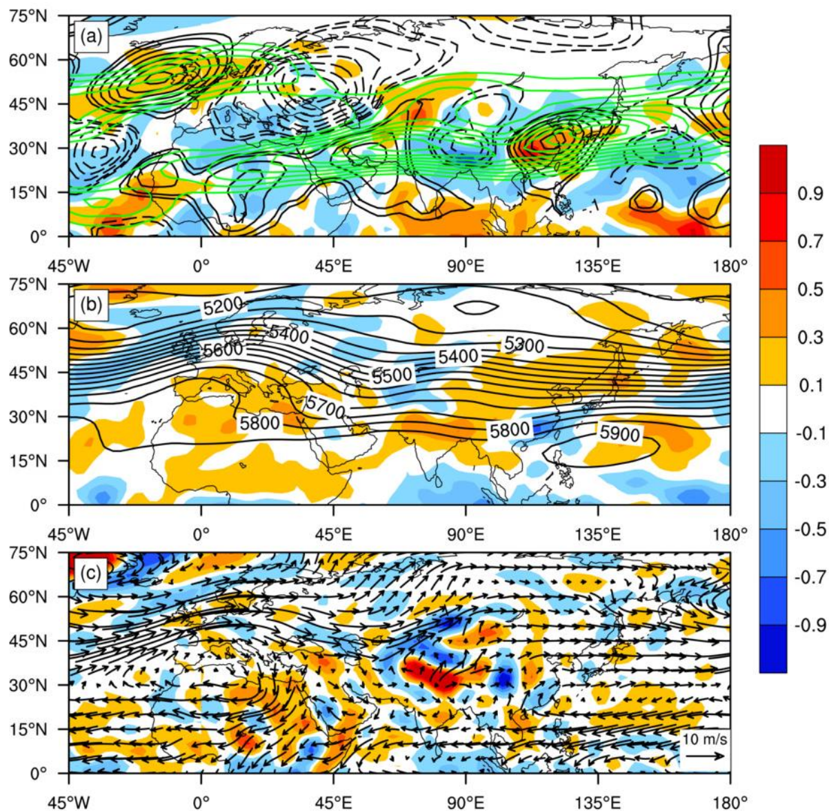
Figure 5: The same as Figure 4 but a composite of absolute values during the periods of November 9-15 and 19-21, December 6-10 and 19-25 in 2015 of : (a) meridional wind (black contours, CI (contour interval) = 1 \text{ m s}^{-1} , solid (dashed) lines represent southerly (northerly) wind), divergence (shading, 10^{-5} \text{ s}^{-1} ) and westerly jet (green line) (zonal mean
