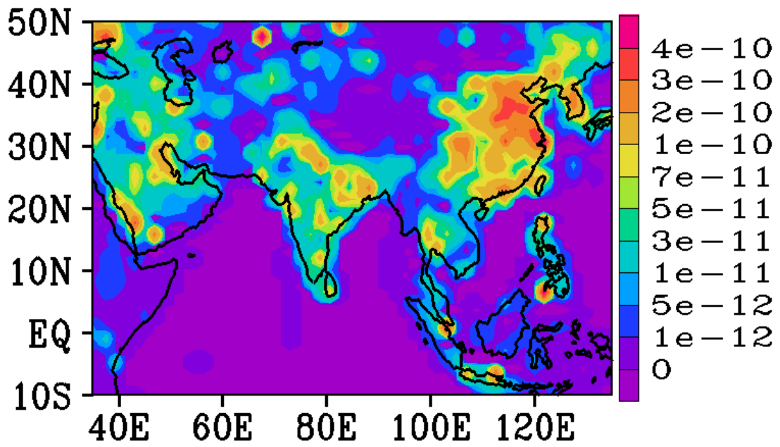
Figure S1. Distribution of SO 2 emission mass flux (kg·m -2 ·s -1 ) averaged for June–September from AEROCOMM-ACCIM II.
