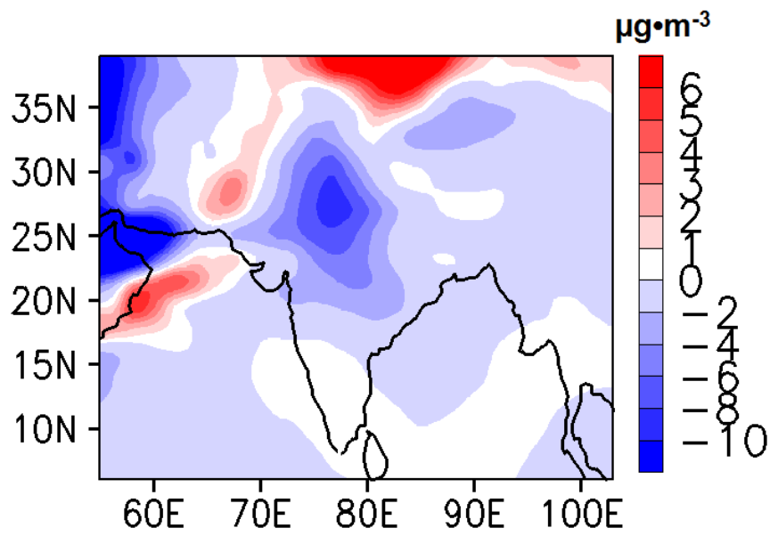
Figure S2: Distribution of anomalies (CTRL-Ind48) averaged for June-September for dust aerosols ( \mu\text{g}\cdot\text{m}^{-3} ) averaged over 1000 - 850 hPa pressure levels.
