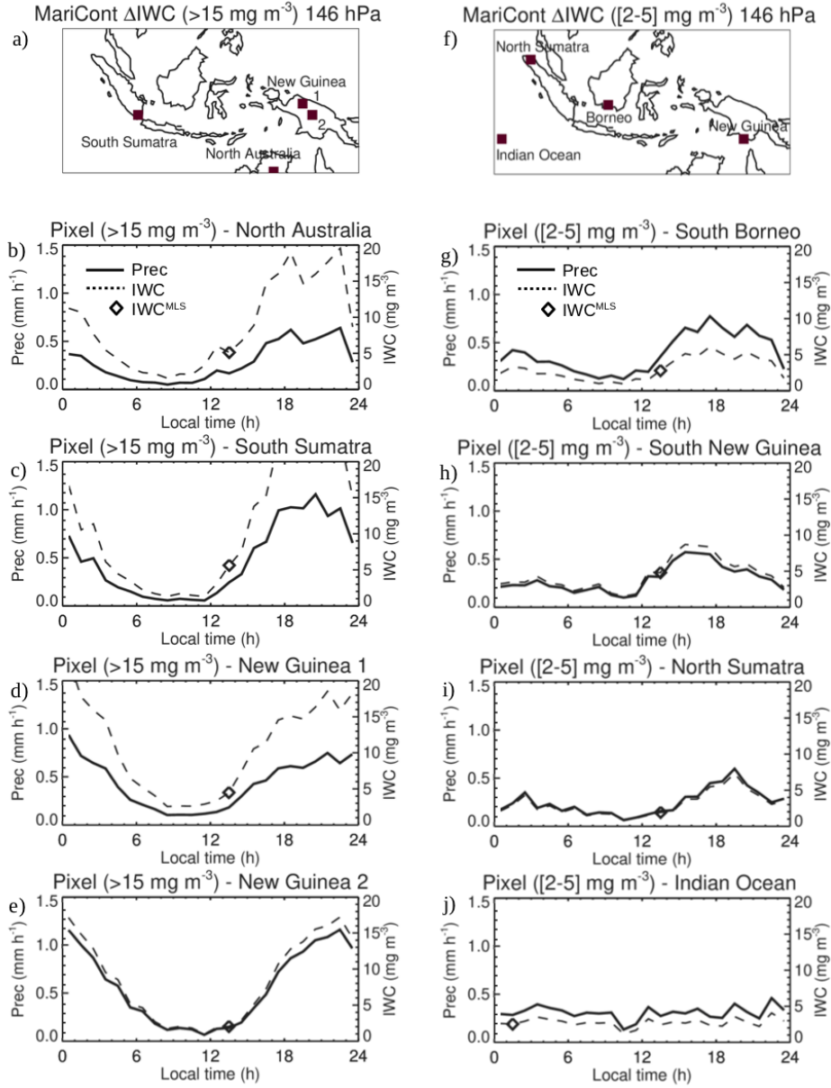
Figure 5. a) and f) Location of 2^\circ \times 2^\circ pixels in Fig. 4 where a) \Delta\text{IWC} have been found higher than > 15 \text{ mg m}^{-3} (in Fig. 4) and where \Delta\text{IWC} have been found between 2 and 5 > \Delta\text{IWC} > 2 \text{ mg m}^{-3} (in Fig. 4), respectively. Diurnal cycle of Prec (solid line) over 4 pixels (in Fig. 4) where \Delta\text{IWC} > 15 \text{ mg m}^{-3} (b, c, d, e) over 4 pixels where and 5 > \Delta\text{IWC} have been found higher than 15 > 2 \text{ mg m}^{-3} (in Fig. 4); (g, h, i, j) over 4 pixels where \Delta\text{IWC} have been found between 2 and 5 \text{ mg m}^{-3} (in Fig. 4), during DJF 2004-2017. The diamond represents \text{IWC}^{\text{MLS}} during the increasing phase of the convection. The dashed line is the diurnal cycle of IWC estimated from the diurnal cycle of Prec and from \text{IWC}^{\text{MLS}} .
