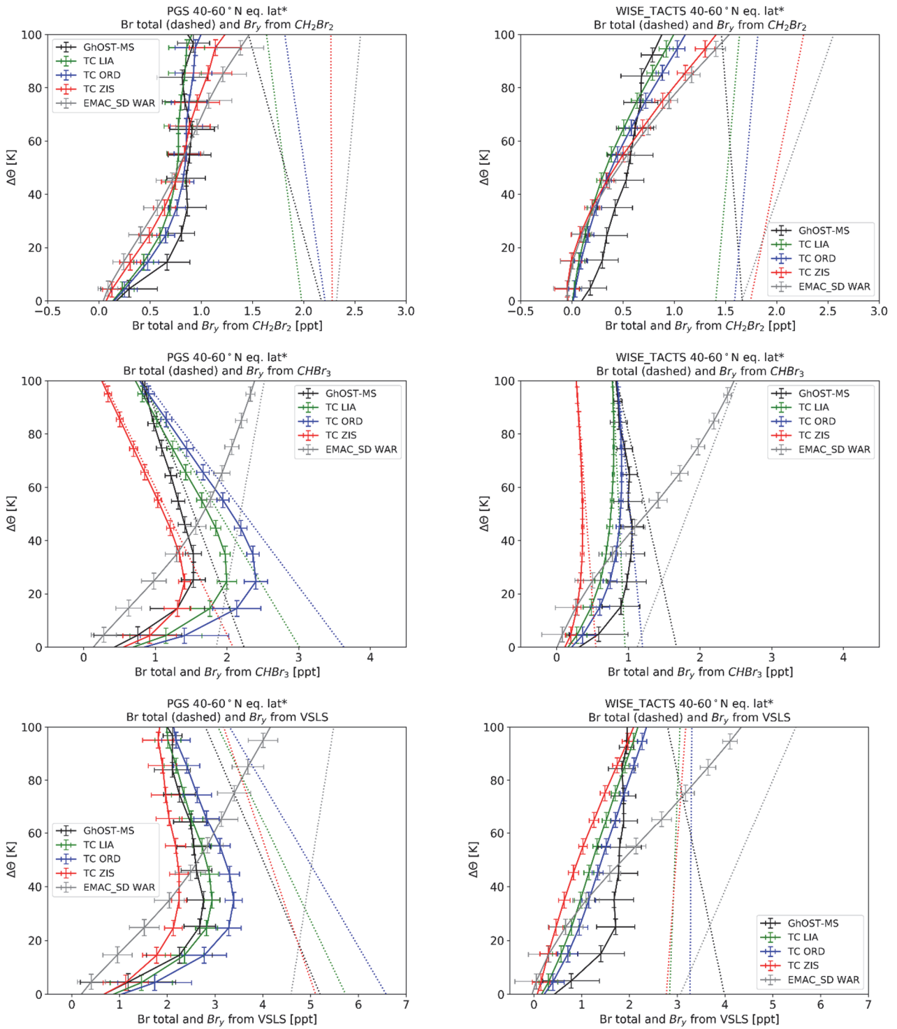
Figure 14 Vertical profiles of Br_y (solid lines) and total bromine (dotted lines) from CH_2Br_2 , from CHBr_3 and from total organic VLSL bromine averaged over 40-60° of equivalent latitude* for the winter PGS campaign (left, late December 2015 to March 2016) and for late summer to early fall period (right, WISE and TACTS campaigns) in comparison to model results from the TOMCAT and the EMAC model using different emission scenarios (see text for details on calculation of Br_y ). Total bromine is calculated from data at the tropical and extratropical tropopause and using assumptions about fractional input from these two source regions (see text for details). The data are displayed as function of potential temperature above the tropopause. In case no model information on the tropopause altitude was available (TOMCAT), climatological tropopause values have been used (see text for details).
