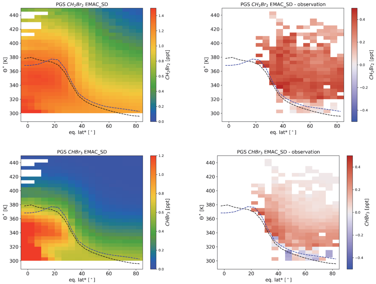
5 Figure 12: As Fig. 9-11 but Latitude-altitude cross section of \text{CH}_2\text{Br}_2 (top) and \text{CHBr}_3 (bottom) for the EMAC model using the Warwick et al. (2006) emission scenario, (left) and differences to the observations (right) for all flights during the PGS campaign from late December 2015 to March 2016. The data are binned using equivalent latitude* and \theta^* as coordinates (see text for details). Also shown in the climatological mean tropopause (black dashed line, see text for details) and the model tropopause (dashed blue line, see text for details). Boxes in which due to the vertical resolution of the model no values are available are left blank.
