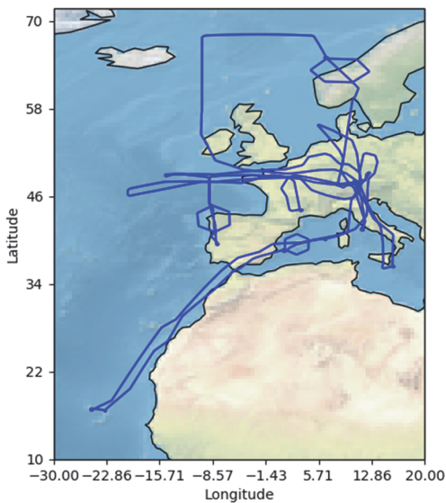
Figure 1: Flight tracks of HALO during the a) TACTS campaign (late August and September 2012) and b) WISE campaign (September/October 2017). The basis of the TACTS campaign was mainly Oberpfaffenhofen (near Munich) in Germany, while the basis of the WISE campaign was Shannon (Ireland).
