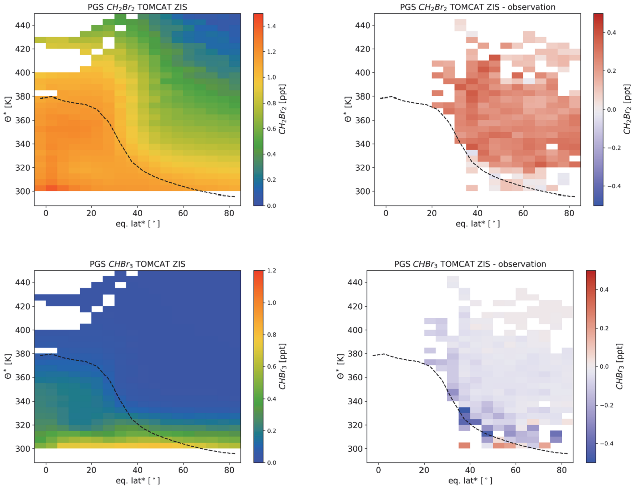
5 Figure 11: -As Fig. 9 and 10 but Latitude-altitude cross section of \text{CH}_2\text{Br}_2 (top) and \text{CHBr}_3 (bottom) for the TOMCAT model using the Ziska et al. (2013) emission scenario, (left) and differences to the observations (right) for all flights during the PGS campaign from late December 2015 to March 2016. The data are binned using equivalent latitude* and \theta^* as coordinates (see text for details). Also shown in the climatological mean tropopause (see text for details; dashed line). Boxes in which due to the vertical resolution of the model no values are available are left blank.
