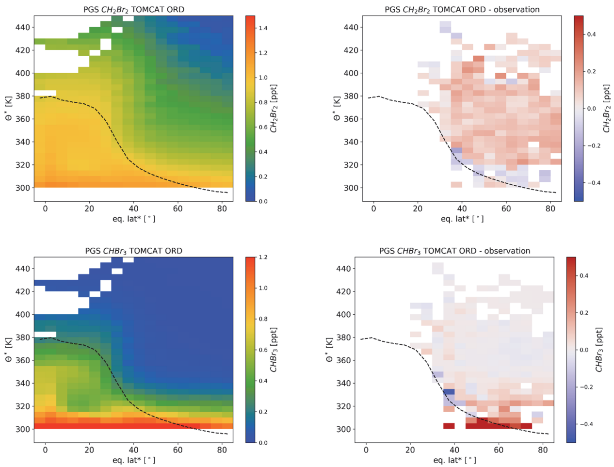
Figure 10: As Fig. 9 but Latitude-altitude cross section of \text{CH}_2\text{Br}_2 (top) and \text{CHBr}_3 (bottom) for the TOMCAT model using the Ordóñez et al. (2012) emission scenario (left) and differences to the observations (right) for all flights during the PGS campaign from late December 2015 to March 2016. The data are binned using equivalent latitude* and \theta^* as coordinates (see text for details). Also shown in the climatological mean tropopause (see text for details; dashed line). Boxes in which due to the vertical resolution of the model no values are available are left blank.
