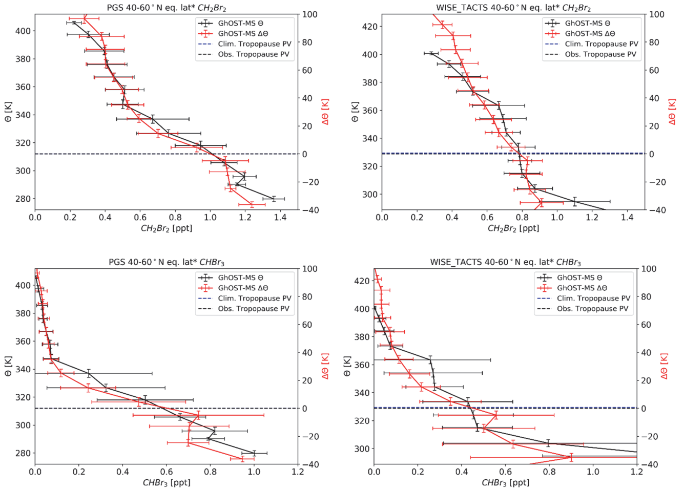
Figure 4: Vertical profiles of \text{CH}_2\text{Br}_2 (top) and \text{CHBr}_3 (bottom) averaged over 40\text{-}60^\circ of equivalent latitude* and all flights during the PGS campaign (left, late December 2015 to March 2016) and from the merged data set from the TACTS and WISE campaigns (right, representative of late summer to fall). The data are displayed as function of potential temperature and potential temperature above the tropopause. The dashed blue line shows the zonal mean dynamical tropopause derived from ERA Interim during September and October of the respective years in the Northern Hemisphere between 40 and 60^\circ latitude, while the black dashed line is the average dynamical tropopause derived for the times and locations of our observations. Both vertical and horizontal error bars denote 1\ \sigma variability.
