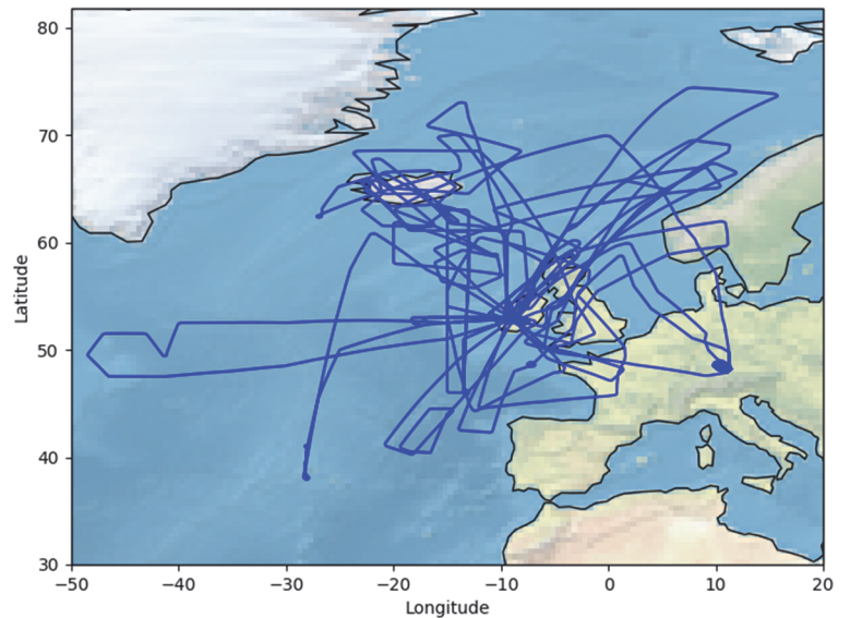
Figure 1: Flight tracks of HALO during the a) TACTS campaign (late August and September 2012) and b) WISE campaign (September/October 2017). The basis of the TACTS campaign was mainly Oberpfaffenhofen (near Munich) in Germany, while the basis of the WISE campaign was Shannon (Ireland).
