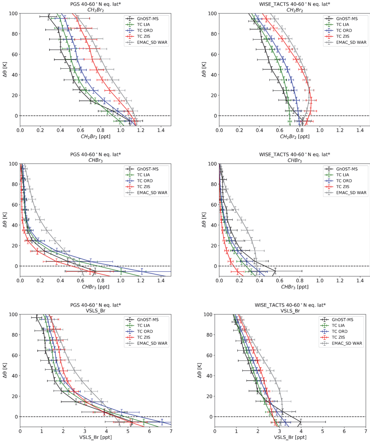
Figure 7: Vertical profiles of \text{CH}_2\text{Br}_2 (top), \text{CHBr}_3 (middle) and total organic VLSL bromine (bottom) -averaged over 40-60° of equivalent latitude* and all flights during the PGS campaign from late December 2015 to March 2016 (left hand side) and from the combined WISE_TACTS data set, representative of late summer to fall conditions. Also shown are model results from the TOMCAT and EMAC model using different emission scenarios (see text for details). The data are displayed as function of potential temperature above the dynamical tropopause. In case no model information on the tropopause altitude was available (TOMCAT), climatological tropopause values have been used (see text for details).
