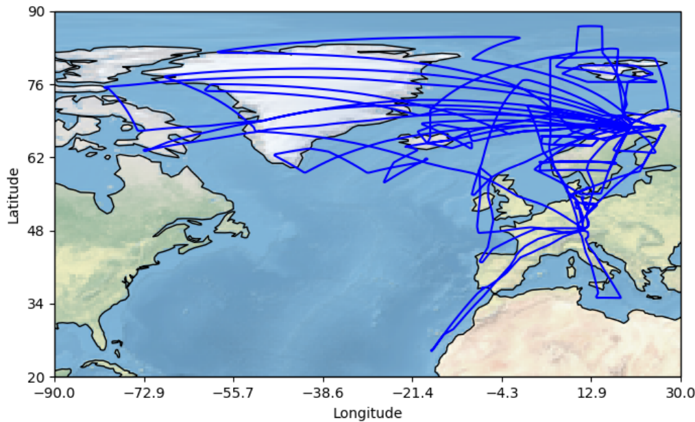
Figure 2: Flight tracks of High Altitude and Long Range Research Aircraft HALO during the PGS ( Polar Stratosphere in a Changing Climate, Investigation of the Life cycle of gravity waves and Seasonality of Air mass transport and origin in the Lowermost Stratosphere ) campaign (December 2015 to April 2016). The basis of the campaign was mainly Kiruna in Northern Sweden.
