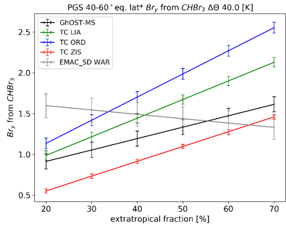
Figure 15: Sensitivity of Br_y from CH_2Br_2 and CHBr_3 (parts per trillion, ppt, 10^{-12} ) at \Delta\theta of \approx 40 K as a function of the fraction of extratropical air for the PGS ( Polar Stratosphere in a Changing Climate, Investigation of the Life cycle of gravity waves and Seasonality of Air mass transport and origin in the Lowermost Stratosphere ) campaign from January to April 2016 for observations in comparison to the different model calculation.
