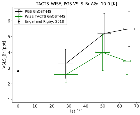
5 Figure 6: Latitudinal cross section of \text{CH}_2\text{Br}_2 , (to left), \text{CHBr}_3 (top right) and total organic VLSLs bromine (bottom) (parts per trillion, ppt; 10^{-12} ) for all three campaigns, binned by latitude and averaged within 10 K below the local dynamical tropopause. Also included are the reference values for the tropical tropopause (Engel and Rigby, 2018).
