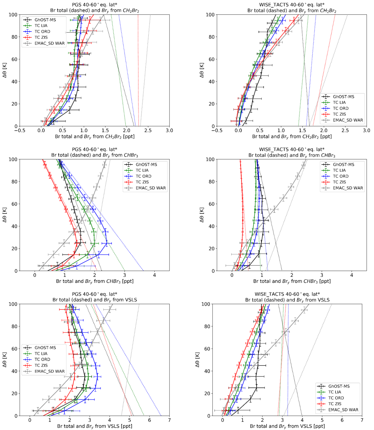
Figure 14 Vertical profiles of Br_y (solid lines; parts per trillion, ppt, \cdot 10^{-12} ) and total Bromine (dotted lines; ppt) from CH_2Br_2 , from CHBr_3 and from total organic VSLs bromine averaged over 40-60° of equivalent latitude* for the winter PGS ( Polar Stratosphere in a Changing Climate, Investigation of the Life cycle of gravity waves and Seasonality of Air mass transport and origin in the Lowermost Stratosphere ) campaign (left, late December 2015 to March 2016) and for late summer to early fall period (right, Wave driven isentropic exchange (WISE) and Transport and Composition in the Upper Troposphere/Lowermost Stratosphere (TACTS) ) campaigns) in comparison to model results from the Toulouse Off-line Model of Chemistry And Transport (TOMCAT) and the ECHAM/MESy Atmospheric Chemistry (EMAC) model using different emission scenarios (see text for details on calculation of Br_y ). Total Bromine is calculated from data at the tropical and extratropical tropopause and using assumptions about fractional input from these two source regions (see text for details). The data are displayed as function of potential temperature above the tropopause. In case no model information on the tropopause altitude was available (TOMCAT), climatological tropopause values have been used (see text for details).
