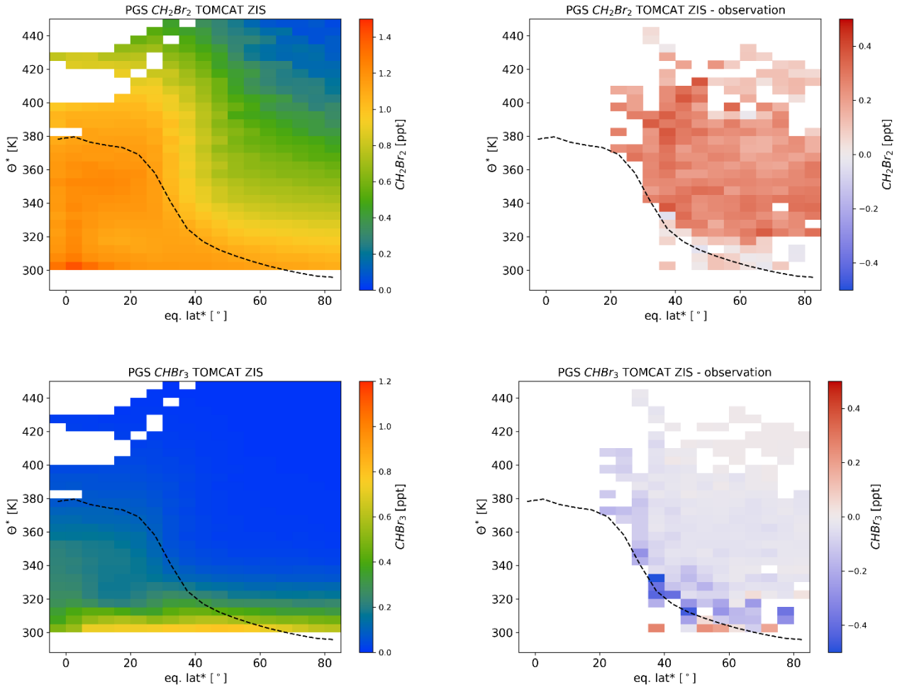
5 Figure 11: Latitude altitude cross section of \text{CH}_2\text{Br}_2 (top) and \text{CHBr}_3 (parts per trillion, ppt; 10^{-12} bottom) for the Toulouse Off line Model of Chemistry And Transport (TOMCAT) model using the Ziska et al. (2013) emission scenario (left) and differences to the observations (right) for all flights during the PGS (Polar Stratosphere in a Changing Climate, Investigation of the Life cycle of gravity waves and Seasonality of Air mass transport and origin in the Lowermost Stratosphere) campaign from late December 2015 to March 2016. The data are binned using equivalent latitude* and \theta^* as coordinates (see text for details). Also shown in the climatological mean tropopause (see text for details; dashed line). Boxes in which due to the vertical resolution of the model no values are available are left blanc. 10
