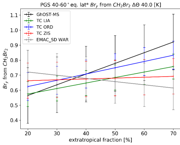
Figure 15: Sensitivity of Br_y from CH_2Br_2 and CHBr_3 (parts per trillion, ppt, 10^{-12} ) at \Delta\theta of \approx 40 K as a function of the fraction of extratropical air for the PGS ( Polar Stratosphere in a Changing Climate, Investigation of the Life cycle of gravity waves and Seasonality of Air mass transport and origin in the Lowermost Stratosphere ) campaign from January to April 2016 for observations in comparison to the different model calculation.
