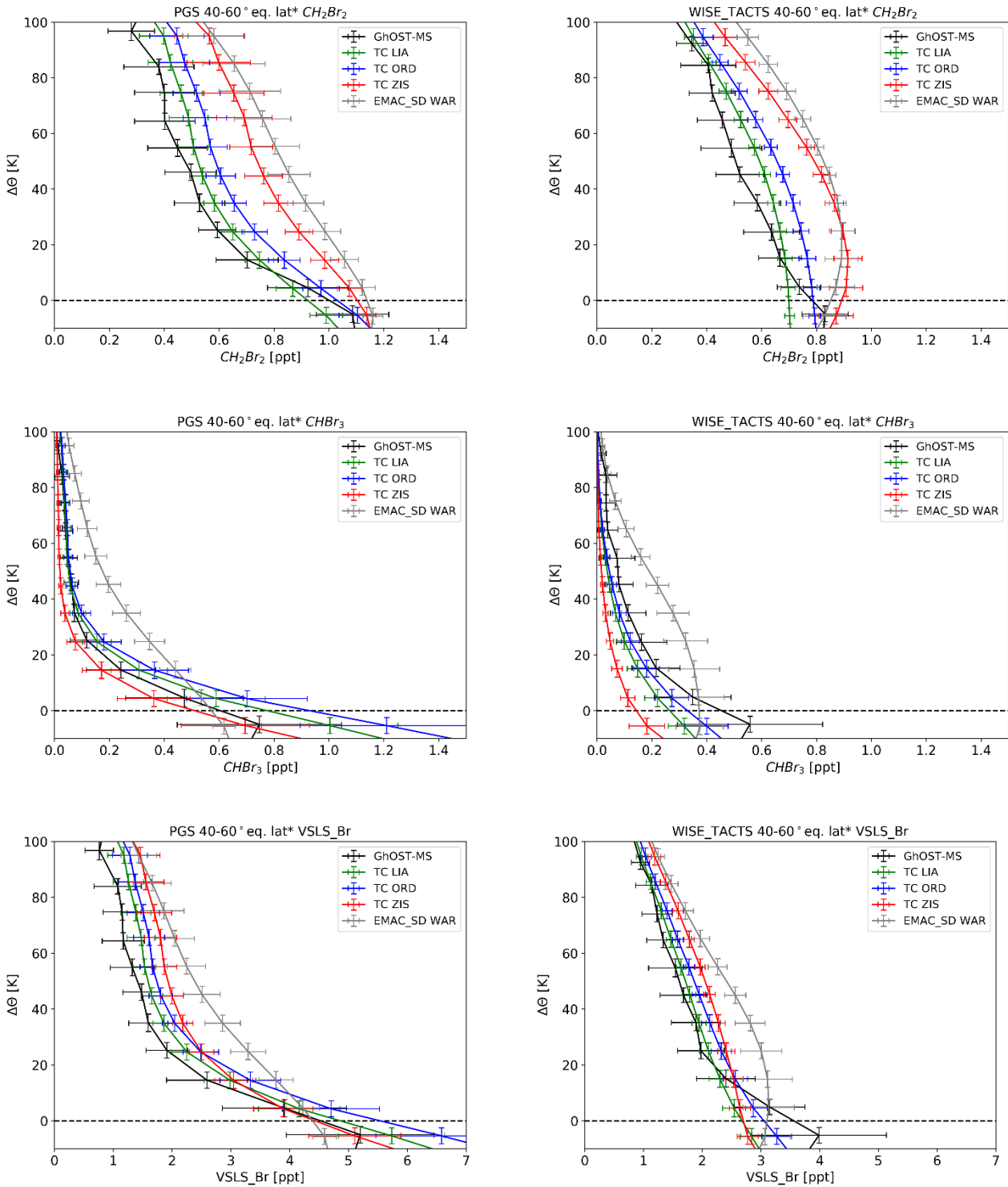
Figure 7: Vertical profiles of \text{CH}_2\text{Br}_2 (top), and \text{CHBr}_3 (middle) and total organic VLSL bromine (bottom) (parts per trillion, ppt; 10^{-12} ) averaged over 40-60° of equivalent latitude* and all flights during the PGS (Polar Stratosphere in a Changing Climate, Investigation of the Life-cycle of gravity waves and Seasonality of Air-mass transport and origin in the Lowermost Stratosphere) campaign from late December 2015 to March 2016 (left hand side) and from the combined WISE_TACTS (Wave driven isentropic exchange, WISE; and Transport and Composition in the Upper Troposphere/Lowermost Stratosphere, TACTS) data set, representative of late summer to fall conditions. Also shown are model results from the Toulouse Off line Model of Chemistry And Transport (TOMCAT) and ECHAM/MESy Atmospheric Chemistry (EMAC) model using different emission scenarios (see text for details). Data from some flight of the TACTS campaign have been omitted due to some extremely high values, which are suspected to be a contamination. The data are displayed as function of potential temperature above the dynamical tropopause. In case no model information on the tropopause altitude was available (TOMCAT), climatological tropopause values have been used (see text for details).
