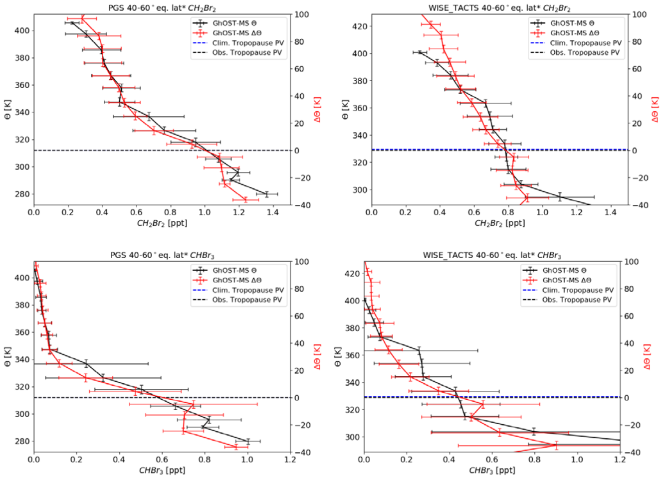
Figure 4: Vertical profiles of \text{CH}_2\text{Br}_2 (top) and \text{CHBr}_3 (bottom) (parts per trillion, ppt; 10^{-12} ), averaged over 40-60° of equivalent latitude* and all flights during the PGS ( Polar Stratosphere in a Changing Climate, Investigation of the Life cycle of gravity waves and Seasonality of Air mass transport and origin in the Lowermost Stratosphere ) campaign (left, late December 2015 to March 2016) and from the merged data set from the Transport and Composition in the Upper Troposphere/Lowermost Stratosphere and Wave driven isentropic exchange TACTS and WISE campaigns (right, representative of late summer to fall). The data are displayed as function of potential temperature and potential temperature above the tropopause. The dotted-dashed blue line shows the zonal mean dynamical tropopause derived from ERA Interim during September and October of the respective years in the Northern Hemisphere between 40 and 60° latitude, while the black dashed line is the average dynamical tropopause derived for the times and locations of our observations. Both vertical and horizontal error bars denote 1 sigma variability.
