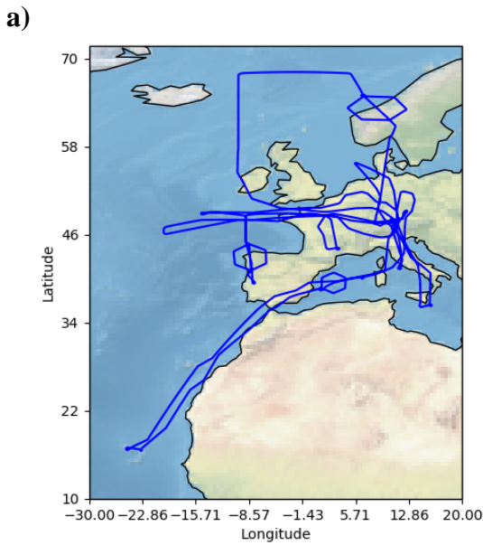
Figure 1: Flight tracks of High Altitude and Long Range Research Aircraft HALO during the a) Transport and Composition in the Upper Troposphere/Lowermost Stratosphere (TACTS) campaign (late August and September 2012) and b) the Wave driven isentropic exchange (WISE) campaign (September/October 2017). The basis of the TACTS campaign was mainly Oberpfaffenhofen (near Munich) in Germany, while the basis of the WISE campaign was Shannon (Ireland).
