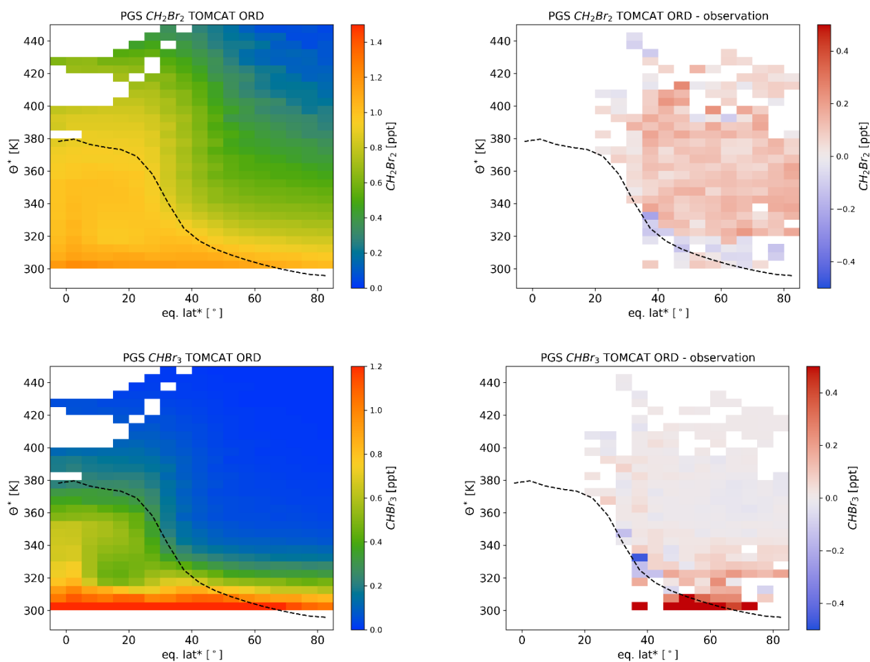
Figure 10: Latitude altitude cross section of \text{CH}_2\text{Br}_2 (top) and \text{CHBr}_3 (bottom) (parts per trillion, ppt; 10^{-12} ) for the Toulouse Off line Model of Chemistry And Transport (TOMCAT) model using the Ordóñez et al. (2012) Ordóñez et al. (2012) emission scenario (left) and differences to the observations (right) for all flights during the PGS (Polar Stratosphere in a Changing Climate, Investigation of the Life cycle of gravity waves and Seasonality of Air mass transport and origin in the Lowermost Stratosphere) campaign from late December 2015 to March 2016. The data are binned using equivalent latitude* and \theta^* as coordinates (see text for details). Also shown in the climatological mean tropopause (see text for details; dashed line). Boxes in which due to the vertical resolution of the model no values are available are left blanc.
