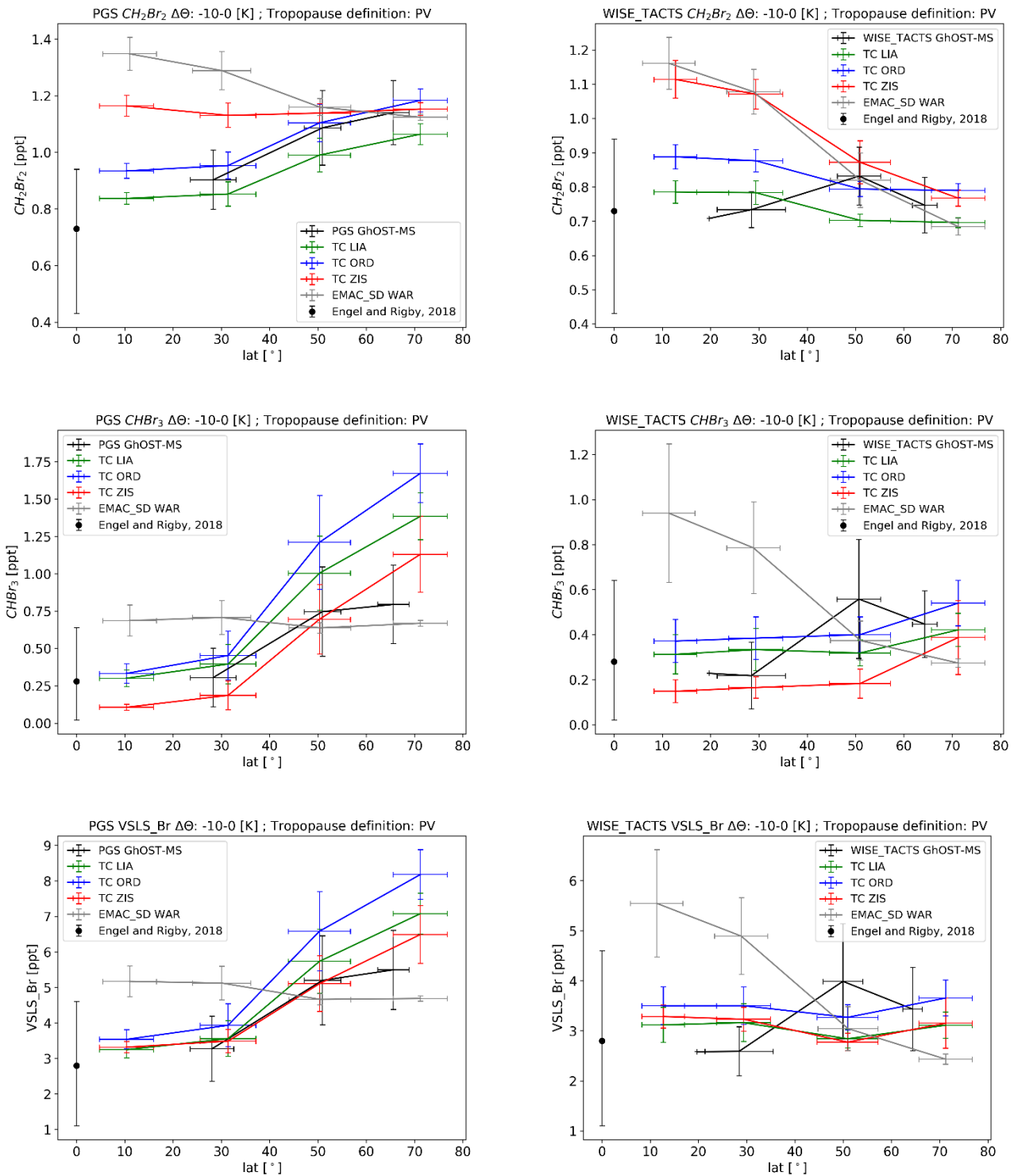
5 Figure 13: Latitude cross section of tropopause representative values of \text{CH}_2\text{Br}_2 (top) \text{CHBr}_3 (middle) and total organic VLS bromine (parts per trillion, ppt; 10^{-12} ) for all the measurements from the PGS (Polar Stratosphere in a Changing Climate, Investigation of the Life cycle of gravity waves and Seasonality of Air mass transport and origin in the Lowermost Stratosphere) campaign (left) and WISE_TACTS (Wave driven isentropic exchange, WISE; and Transport and Composition in the Upper Troposphere/Lowermost Stratosphere, TACTS) dataset (right) from observations in comparison to all model emissions scenario combinations. Data are binned by latitude and averaged over 10 K below the tropopause. Due to the different sampling of the observations and the models the centers of the different latitude bins are not the same for observations and models. 10
