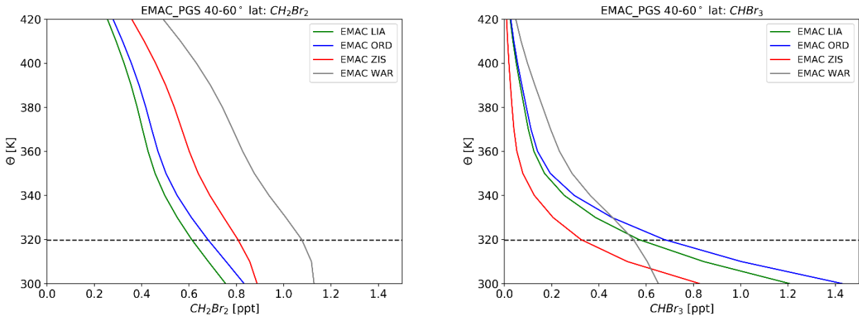
Figure 8: Vertical profiles of CH 2 Br 2 (left) and CHBr 3 (right) (parts per trillion, ppt; 10^{-12} ) averaged over 40-60° latitude from four model simulations with the EMAC model using the emission scenarios by (Liang et al., 2010; Warwick et al., 2006; Ordóñez et al., 2012; Ziska et al., 2013). The data have been averaged for January/February and March, i.e. representative of the time period covered by the PGS ( Polar Stratosphere in a Changing Climate, Investigation of the Life cycle of gravity waves and Seasonality of Air mass transport and origin in the Lowermost Stratosphere ) campaign. The dashed line represents the model tropopause. Model results are for nudged simulations of EMAC but do not cover the time period of our observations.
