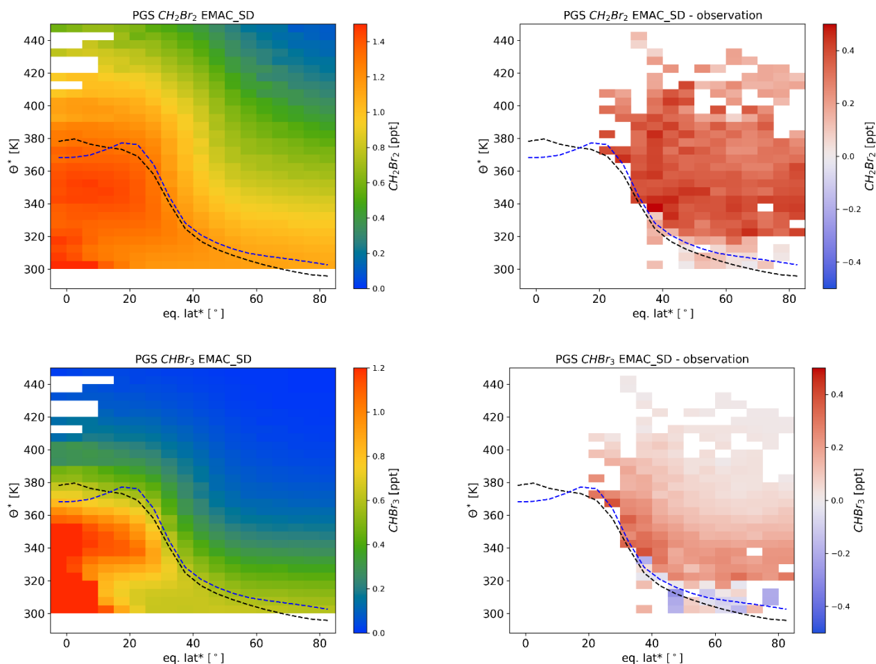
5 Figure 12: Latitude altitude cross section of \text{CH}_2\text{Br}_2 (top) and \text{CHBr}_3 (parts-per-trillion, ppt; 10^{-13} bottom) for the ECHAM/MESy Atmospheric Chemistry (EMAC) model using the Warwick et al. (2006) emission scenario (left) and differences to the observations (right) for all flights during the PGS (Polar Stratosphere in a Changing Climate, Investigation of the Life cycle of gravity waves and Seasonality of Air mass transport and origin in the Lowermost Stratosphere) campaign from late December 2015 to March 2016. The data are binned using equivalent latitude* and \theta^* as coordinates (see text for details). Also shown in the climatological mean tropopause (black dashed line, see text for details) and the model tropopause (dashed blue line, see text for details). Boxes in which due to the vertical resolution of the model no values are available are left blanc. 10
