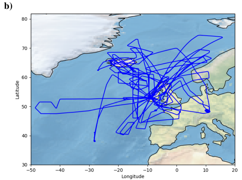
Figure 1: Flight tracks of High Altitude and Long Range Research Aircraft HALO during the a) Transport and Composition in the Upper Troposphere/Lowermost Stratosphere (TACTS) campaign (late August and September 2012) and b) the Wave driven isentropic exchange (WISE) campaign (September/October 2017). The basis of the TACTS campaign was mainly Oberpfaffenhofen (near Munich) in Germany, while the basis of the WISE campaign was Shannon (Ireland).
