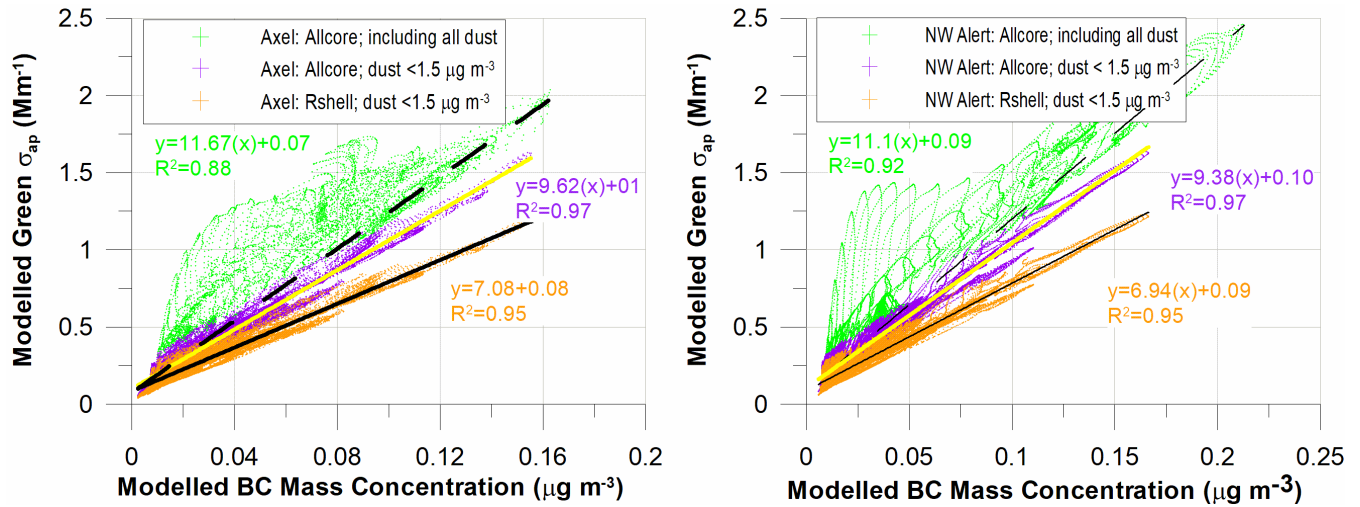
Figure 6. Modelled and observed particle light absorption coefficients ( \sigma_{ap} ) at 550 nm plotted versus black carbon and refractory black carbon (rBC) mass concentrations, respectively: a) modelled data for Axel grid showing all data based on the 'Allcore' assumption (green), data based on the 'Allcore' assumption and with dust limited to less than 1.5 \mu g m^{-3} (purple), data based on the 'Rshell' assumption and with dust limited to less than 1.5 \mu g m^{-3} (orange).
