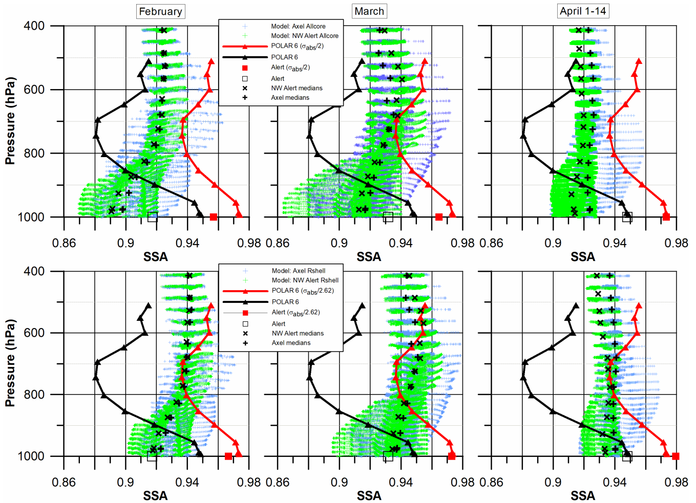
Figure 11. Vertical profile plot of SSA with atmospheric pressure showing modelled results for February (a), March (b) and April 1-14 (c) based on the 'Allcore' assumption and results for February (d), March (e) and April 1-14 (f) based on the 'Rshell' assumption. Median values of SSA from the POLAR 6 observations and the Alert Observatory shown in a, b and c are based on the measured absorption (black points) and the absorption overestimation assumption ( \sigma_{ap}/2 ; red points), corresponding to the 'Allcore' assumption. Median values of SSA from the POLAR 6 observations and the Alert Observatory shown in a, b and c are based on the measured absorption (black points) and the absorption overestimation assumption ( \sigma_{ap}/2.62 ; red points), corresponding to the 'Rshell' assumption.
