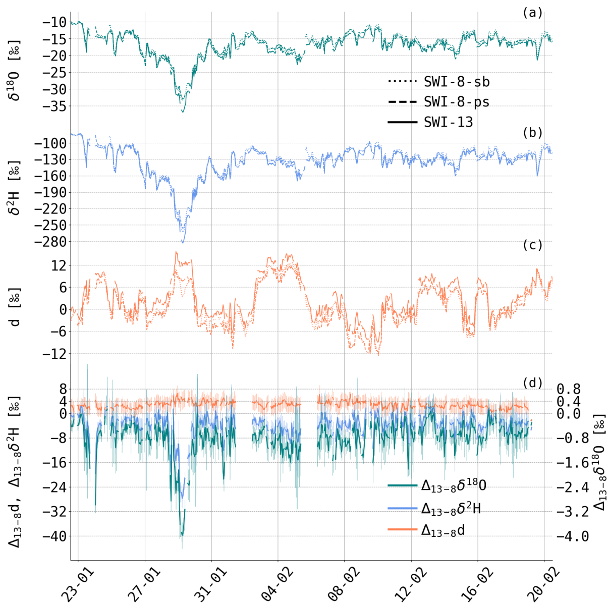
Figure 5. Time series of hourly means of (a) \delta^{18}\text{O} , (b) \delta^2\text{H} , (c) d , and (d) \Delta_{13-8} for leg 2 from SWI-13, SWI-8-ps, and SWI-8-sb measurements. \Delta_{13-8} is the difference between SWI-13 and SWI-8-ps. The errorbars in panel (d) denote hourly standard deviations of the 1s data.
