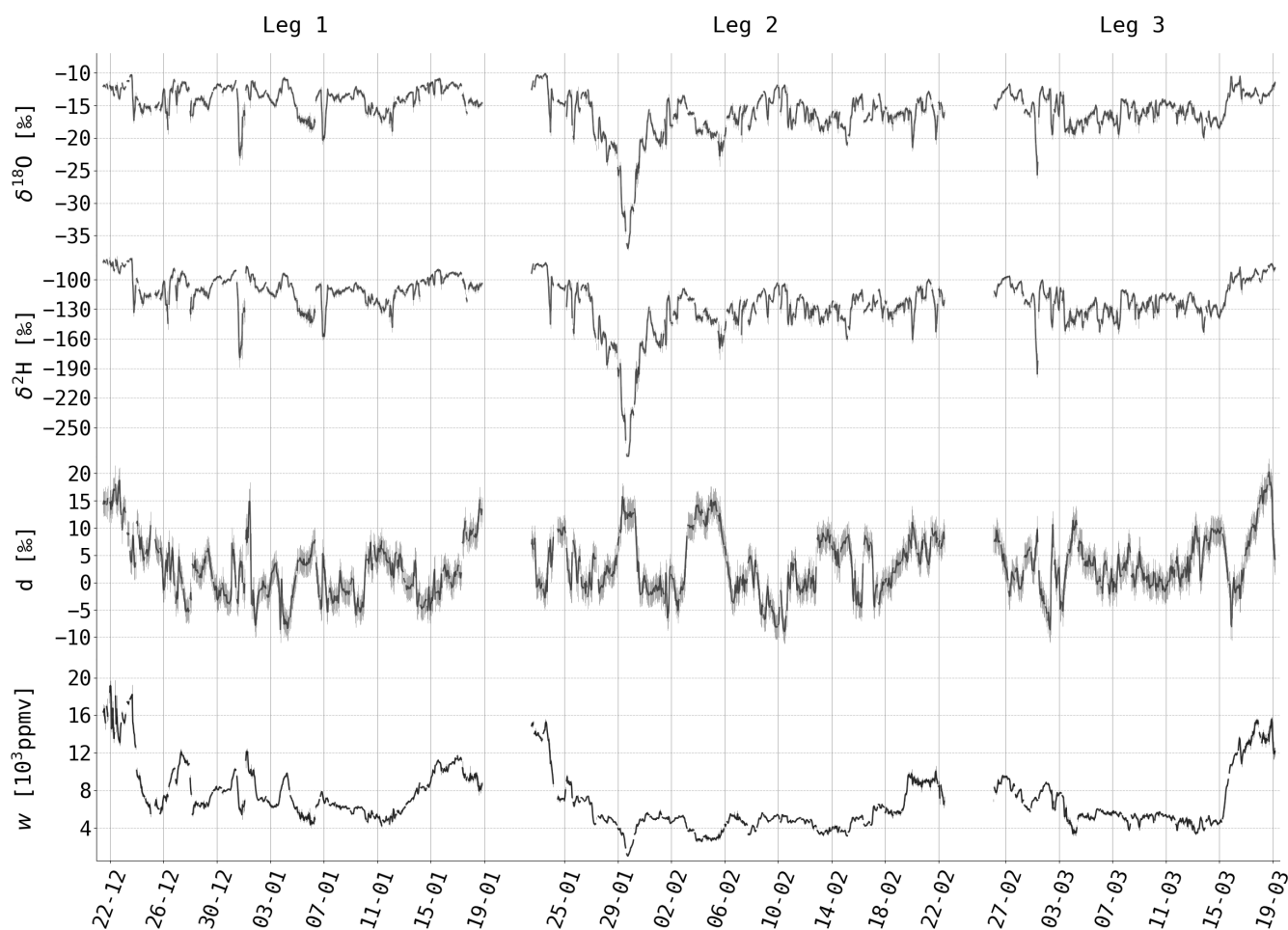
Figure 4. Time series of hourly \delta^{18}\text{O} , \delta^2\text{H} , d , and w for legs 1-3 from SWI-13. The errorbars denote hourly standard deviations of the 1s data.
