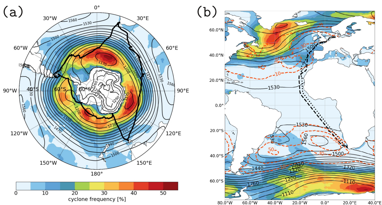
Figure 9. Mean cyclone frequencies (coloured contours, [%]) with geopotential height at 850 hPa (black contours, [m]) are shown for legs 1-3 (a) and legs 0 and 4 (b). The mean anticyclone frequencies (orange, dashed contours, [%]) for legs 0 and 4 are additionally plotted in panel (b). The thick black line shows the ship tracks for legs 1-3. The dashed and dotted black lines show the ship track of legs 0 and 4, respectively. ECMWF operational analysis data was used to produce this Figure.
